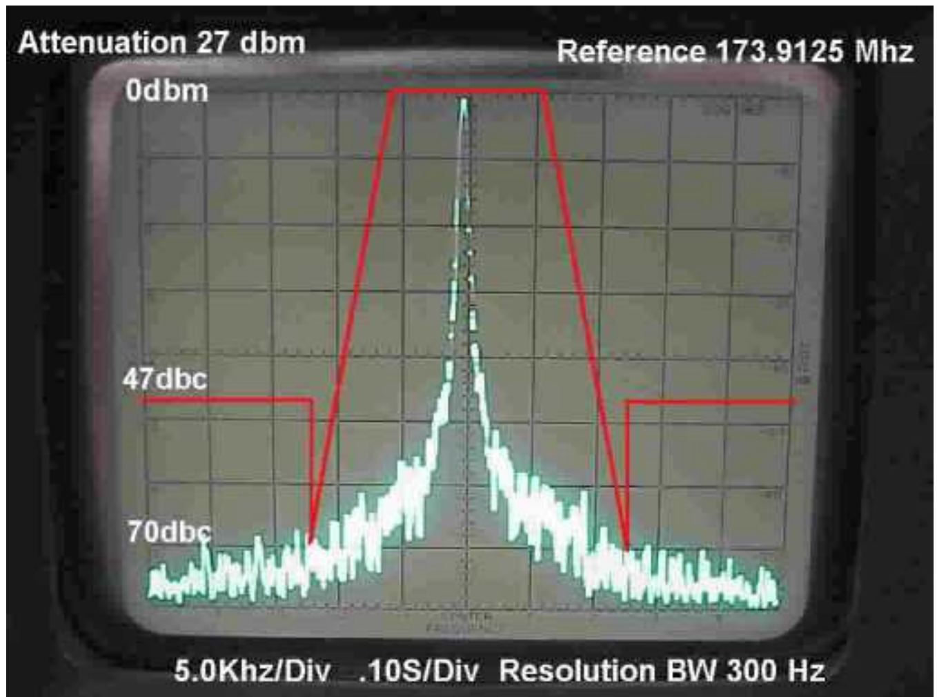
Figure 4 Unmodulated Bandwidth
