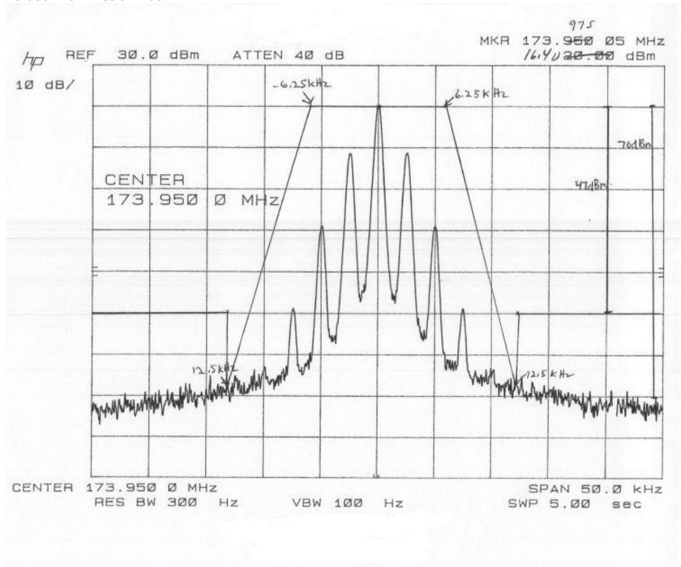
Part 90.210 Emission Mask D
