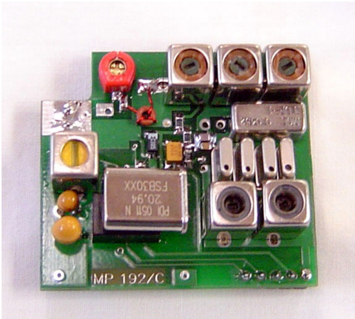
RECEIVER PCB TOP
