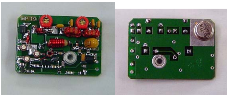
RF PRE-AMP & RF FINAL AMPLIFIER PCB TOP & BOTTOM
