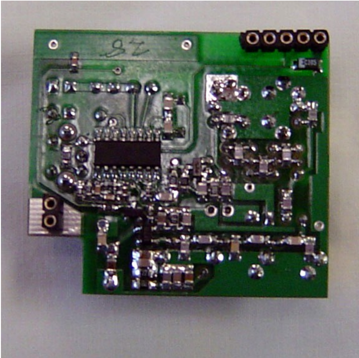
RECEIVER PCB BOTTOM
