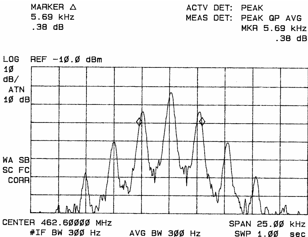
Figure nine Occupied Band Width (voice).
