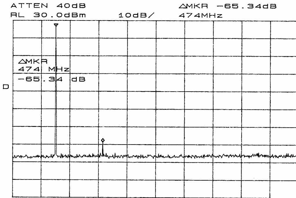
START 30MHz STOP 2.900GHz *RBW 100kHz VBW 100kHz SWP 800ms Figure ten Emissions at Antenna Terminal for FRS unit.
