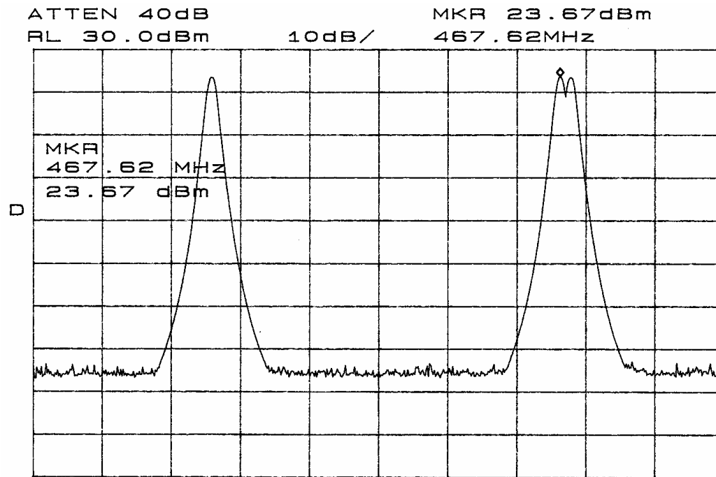
START 460.00MHz STOP 470.00MHz *RBW 100kHz VBW 100kHz SWP 50ms Figure one Power Output at antenna terminal (FRS channels)
