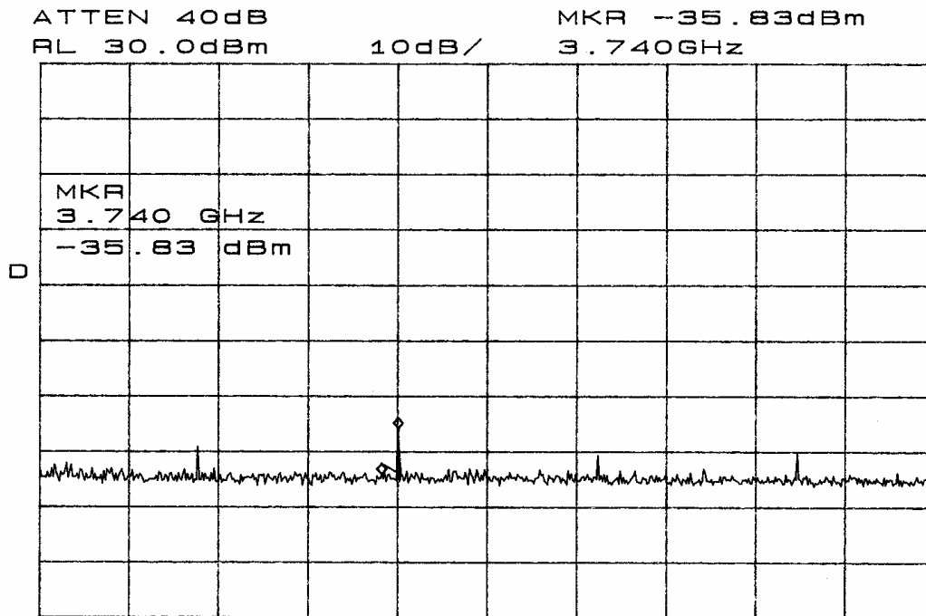
START 2.900GHz STOP 5.000GHz *RBW 100kHz VBW 100kHz SWP 600ms Figure eleven Emissions at Antenna Terminal for FRS unit.
