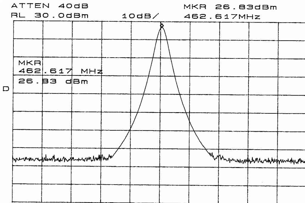
CENTER 462.600MHz SPAN 5.000MHz *RBW 100kHz VBW 100kHz SWP 50ms Figure two Power Output at antenna terminal (GMRS channels)
