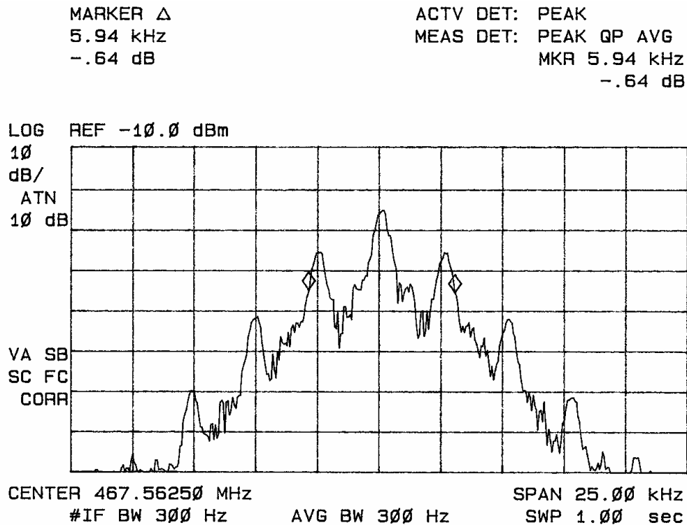
Figure six Occupied Band Width (voice).
