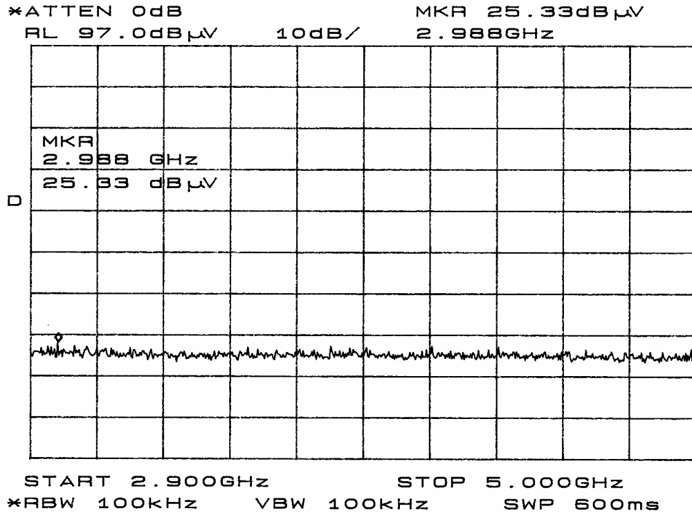
Figure eight Plot of analyzer display showing emissions at 1 meter.
