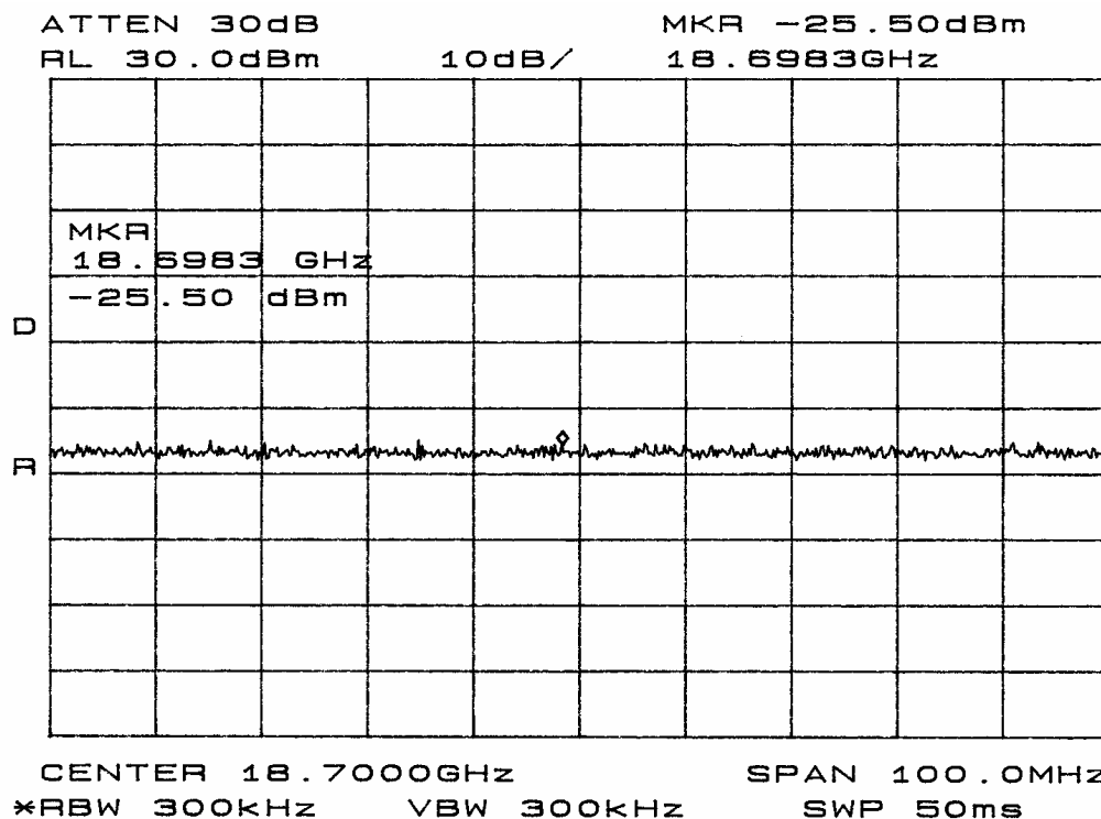
Figure four Plot of analyzer screen showing first harmonic output.
