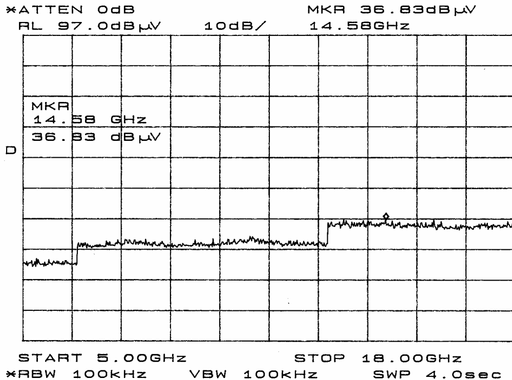
Figure nine Plot of analyzer display showing emissions at 1 meter.
