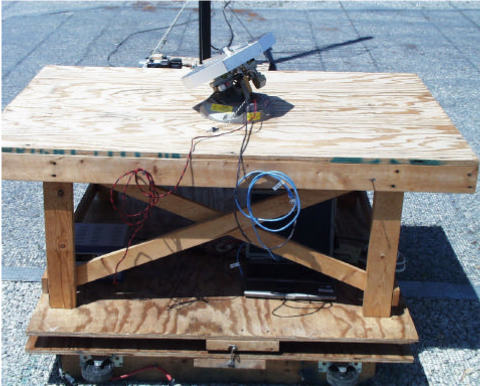
General emissions setup with load over antenna.
