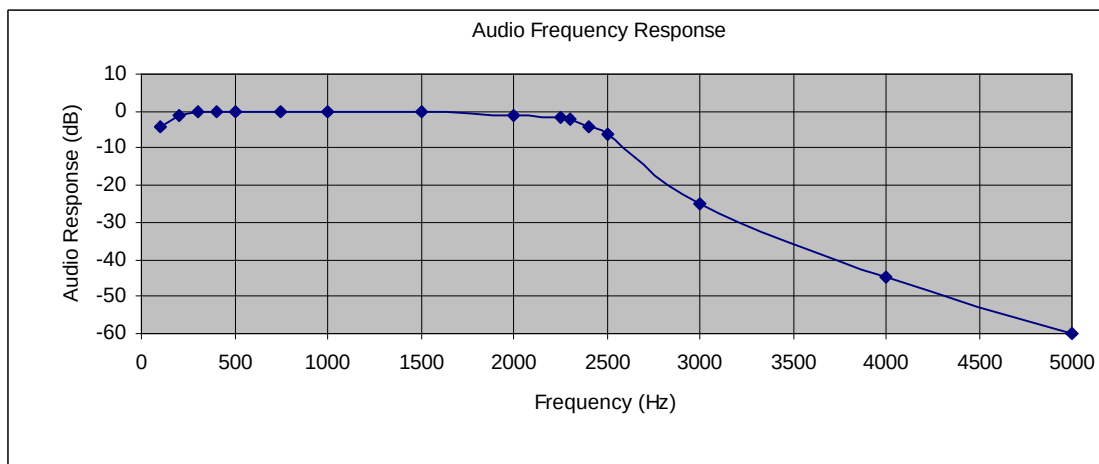
Figure 4: Frequency Response of Audio Lowpass Filter.
