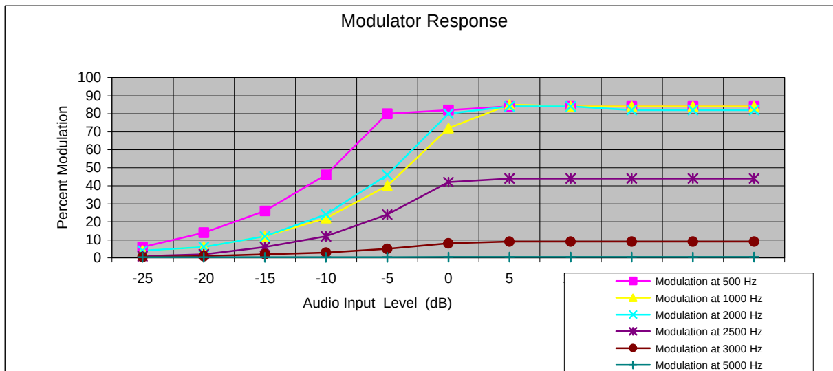
Figure 3: Modulation characteristics.
