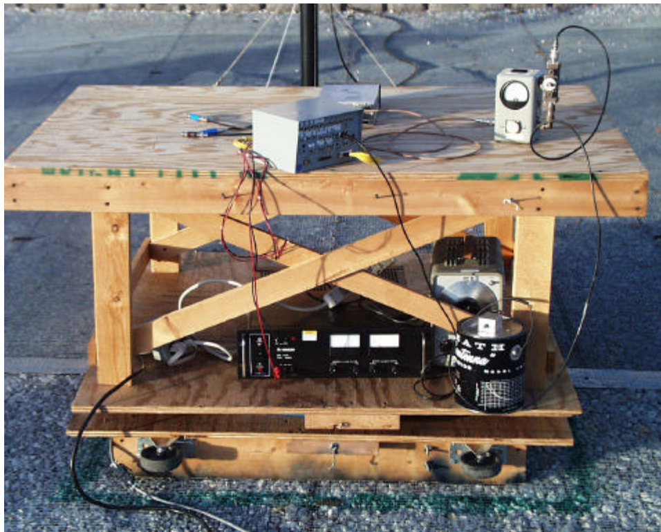
Photographs of Test setups for GNS430A
