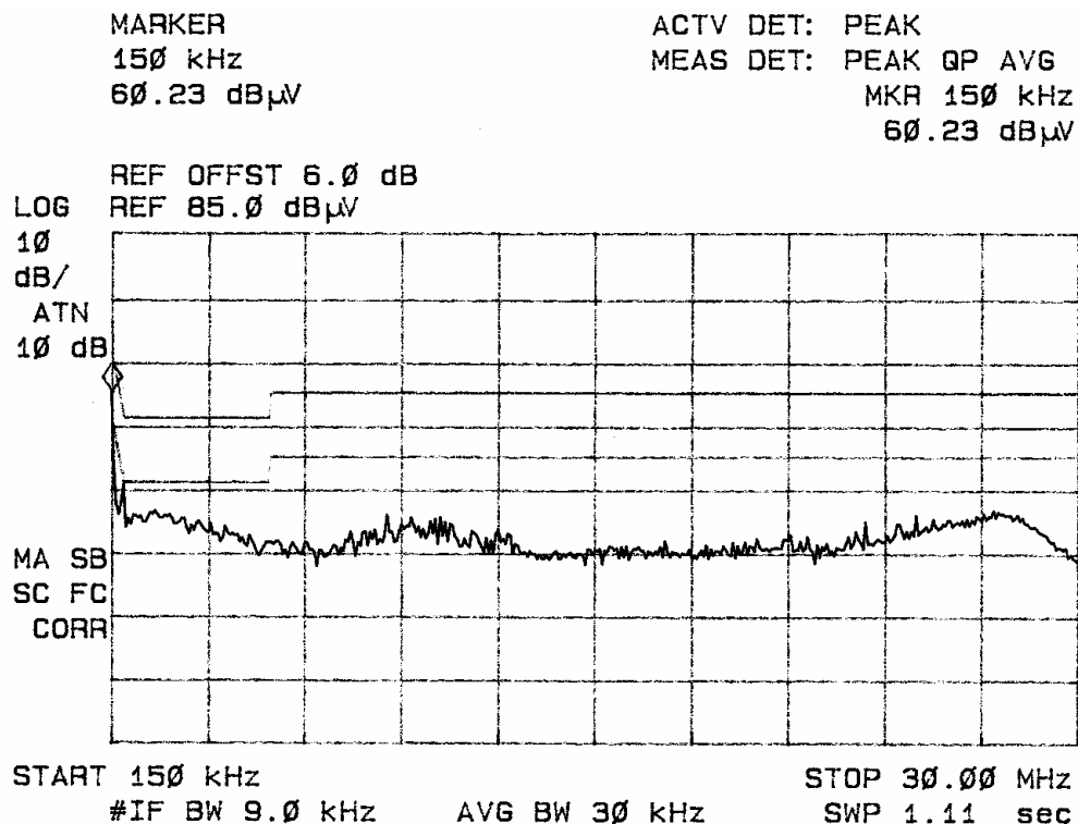
Figure two Conducted emissions of EUT line 2 (configuration #2).
