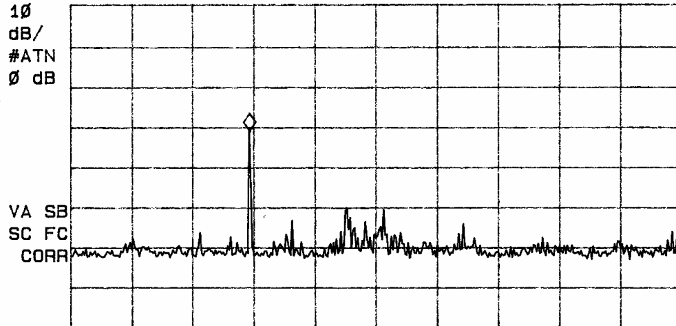
Figure seven Radiated Emissions @ 1 Meter in Screen Room
