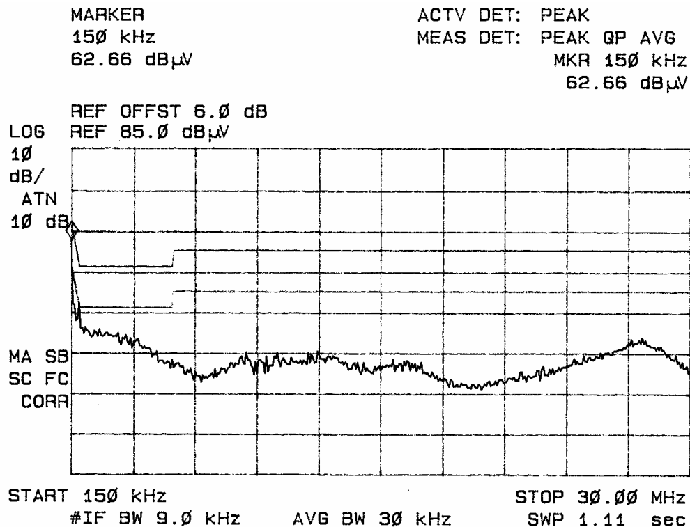
Figure one Conducted emissions of EUT line 1 (configuration #2).
