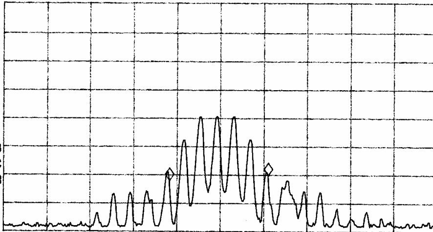
Figure five 200 kHz Occupied Bandwidth requirement
