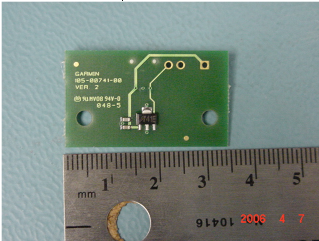
Rotation detector top and bottom
