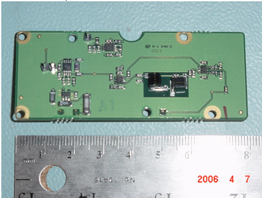
IF Board 1 Top and Bottom
