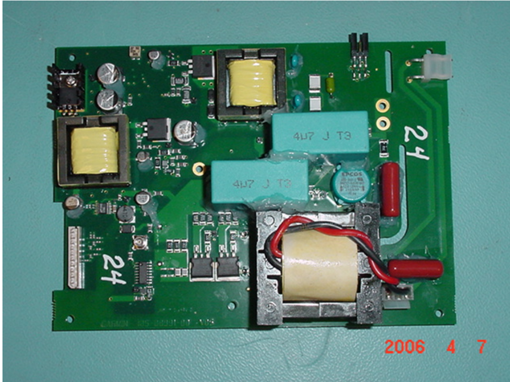
Internal photographs of GMR 40X. Modulator Top and Bottom
