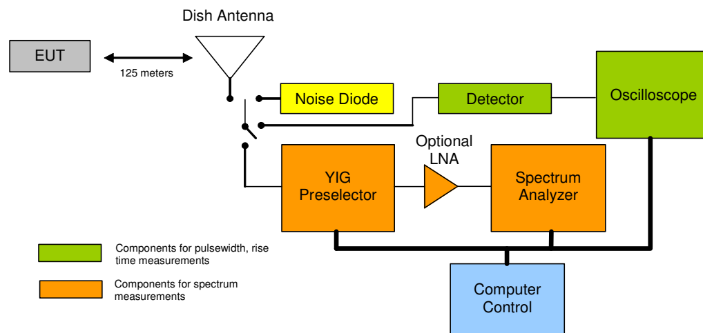
Figure 1. Measurement diagram.
