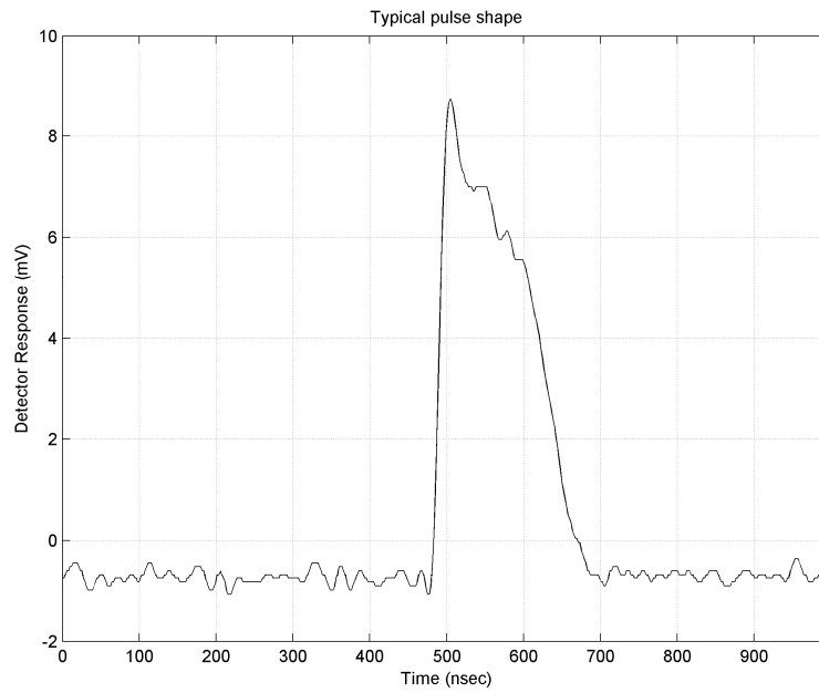
Figure 2. Typical pulse from EUT using wideband detector.
