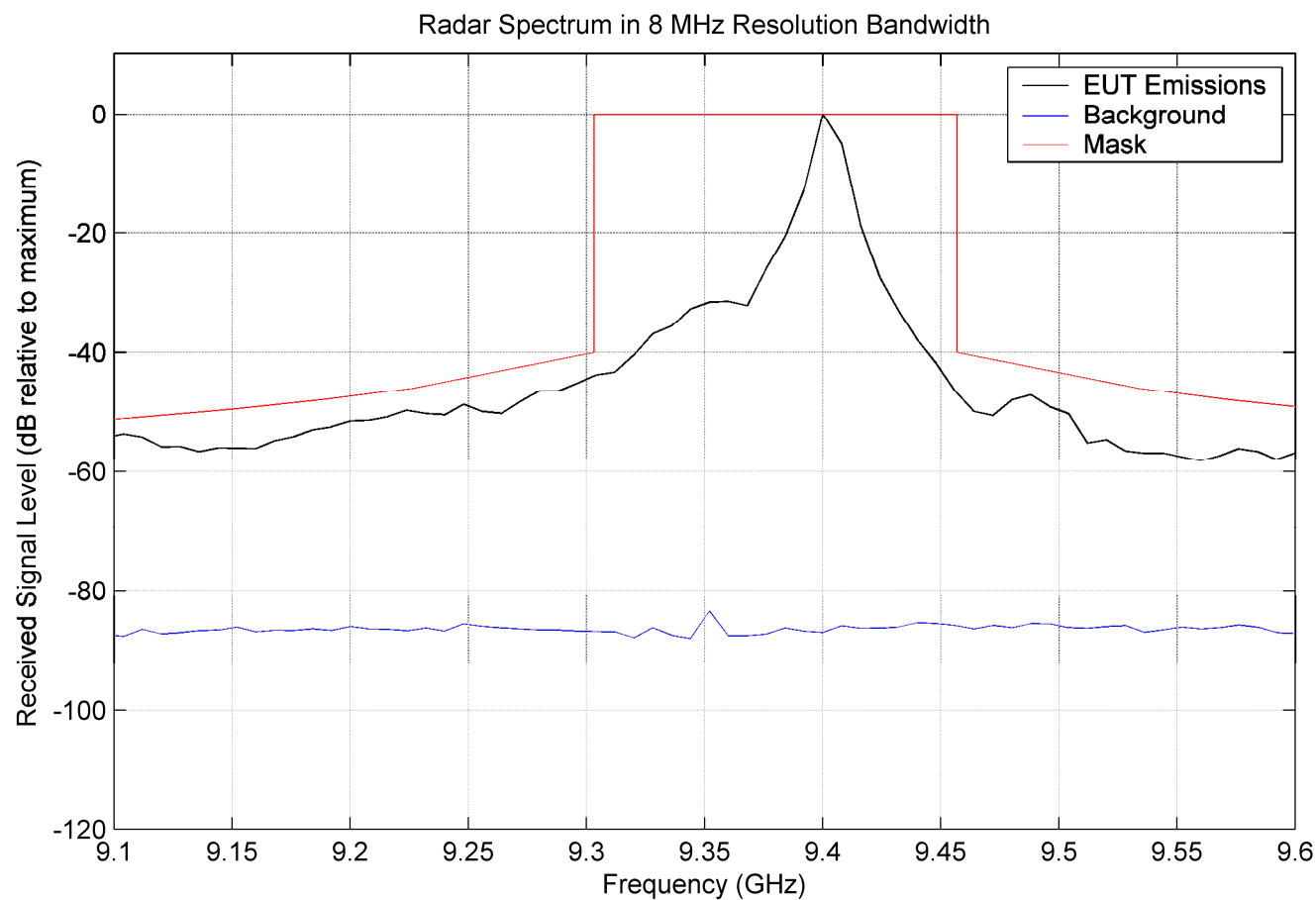
Figure 5. 9.3 to 9.5 GHz band.
