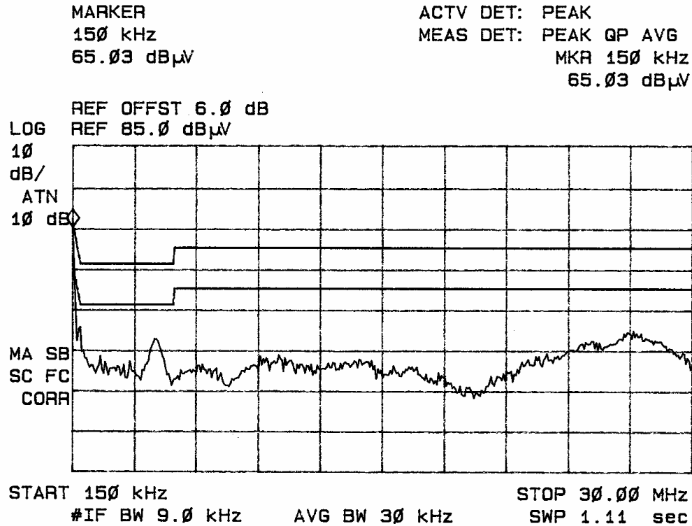
Figure seven Conducted emissions of EUT line 1 (320-00171-14)
