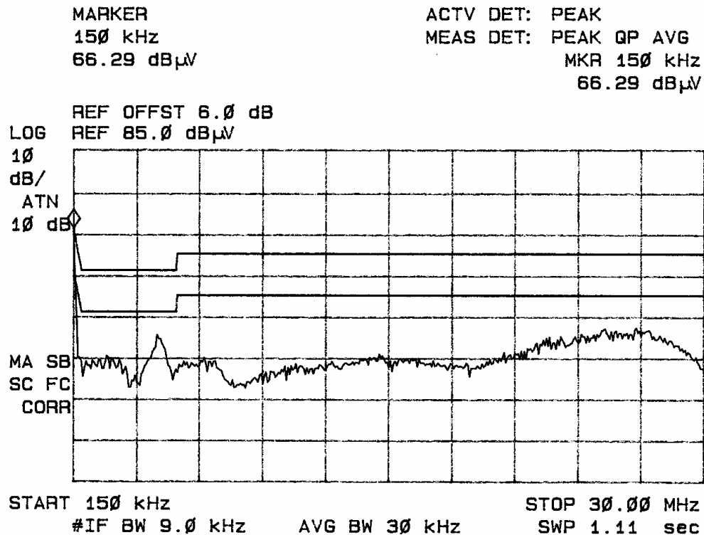
Figure eight Conducted emissions of EUT line 2 (320-00171-14)
