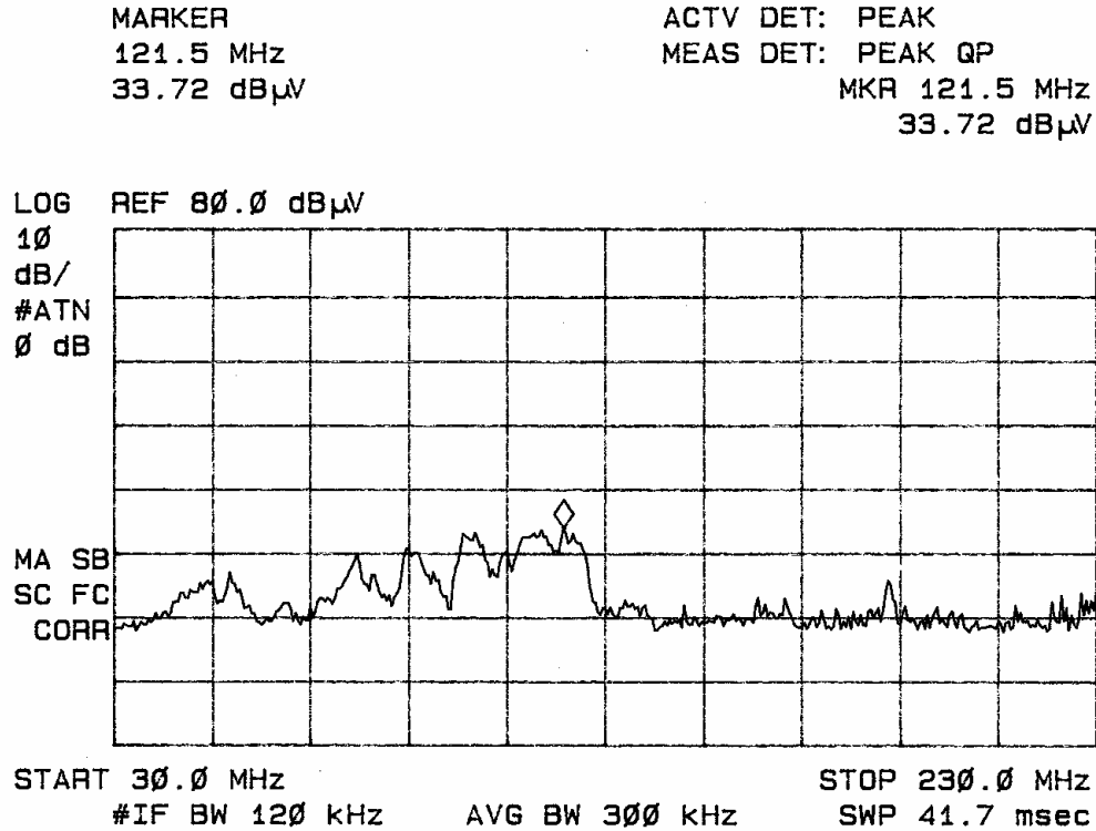
Figure nine Radiated Emissions taken at 1 meter in screen room.
