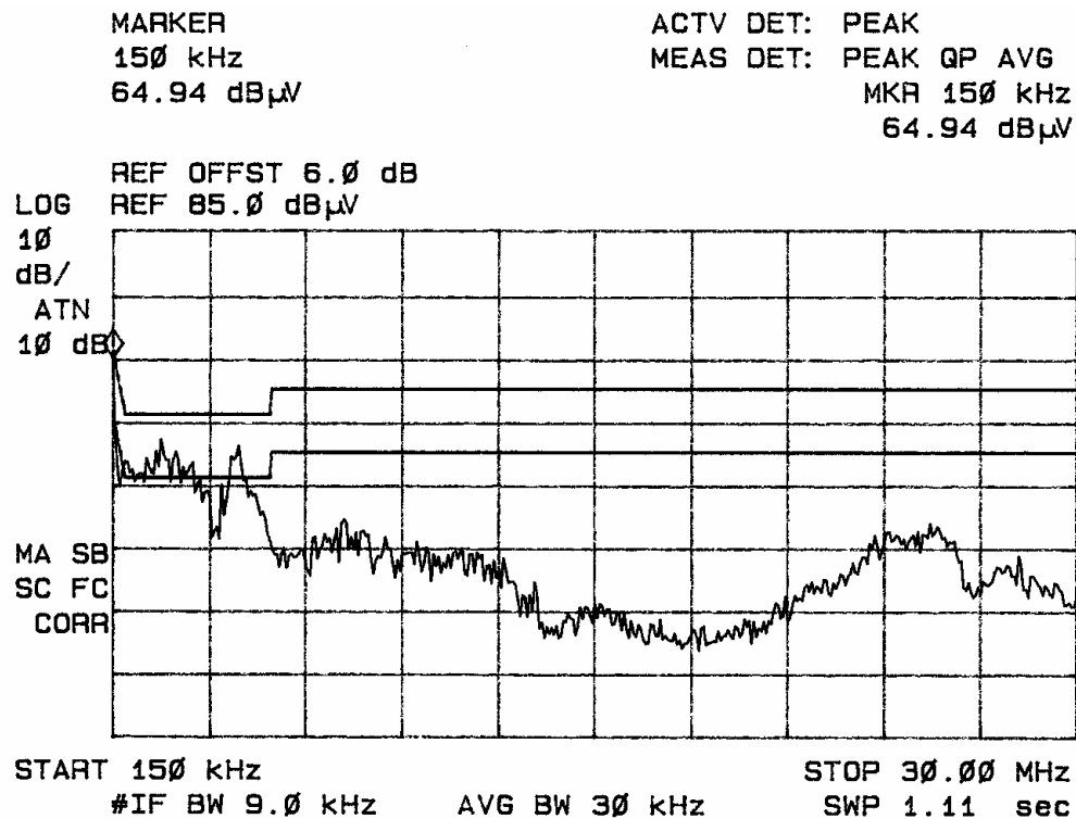
Figure four Conducted emissions of EUT line 2 (320-00171-11)
