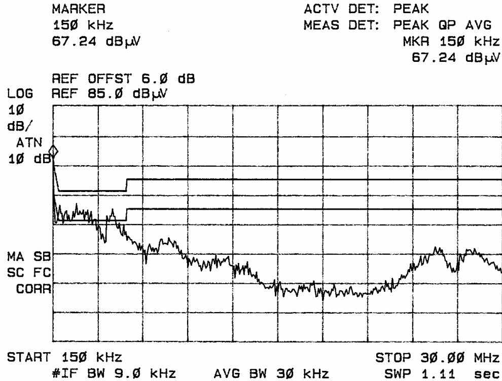
Figure three Conducted emissions of EUT line 1 (320-00171-11)
