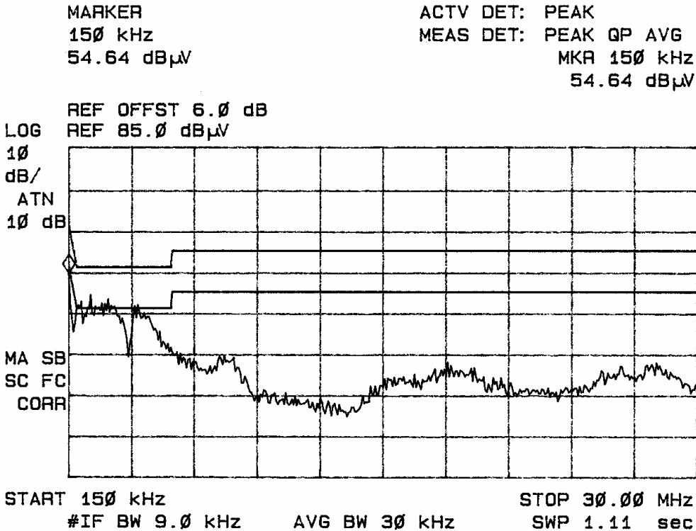
Figure five Conducted emissions of EUT line 1 (320-00171-13)
