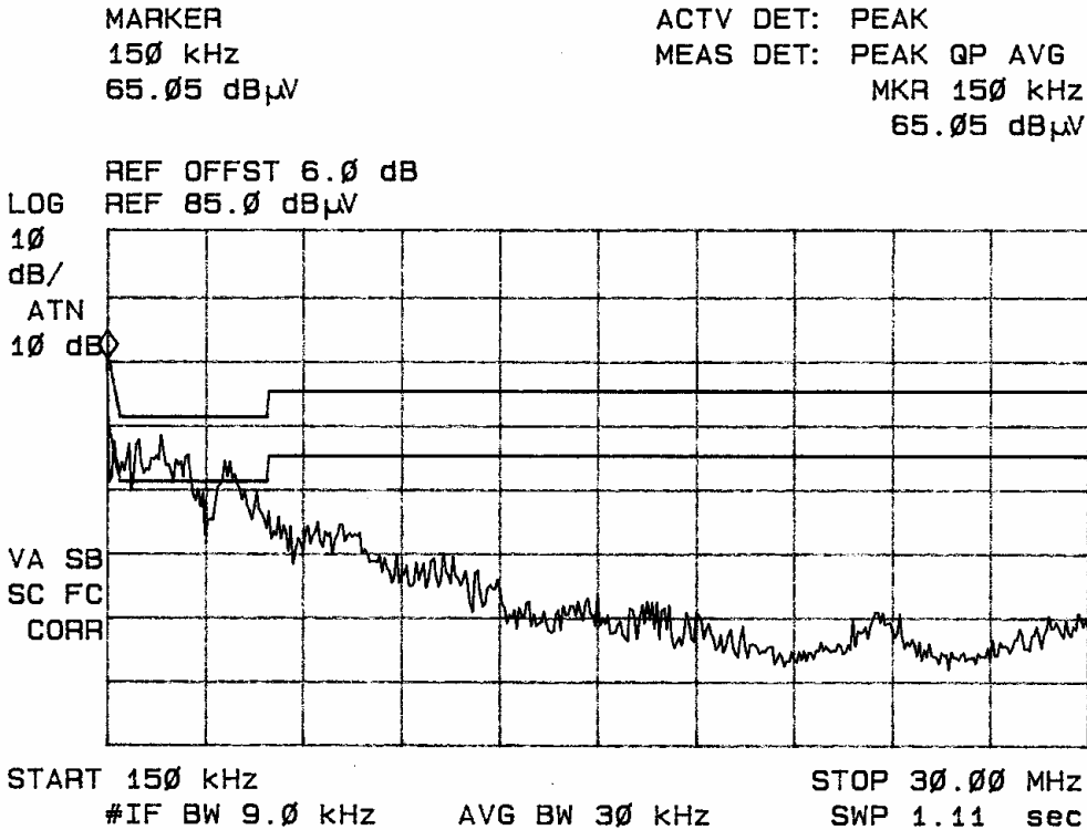
Figure one Conducted emissions of EUT line 1 (320-00171-12)
