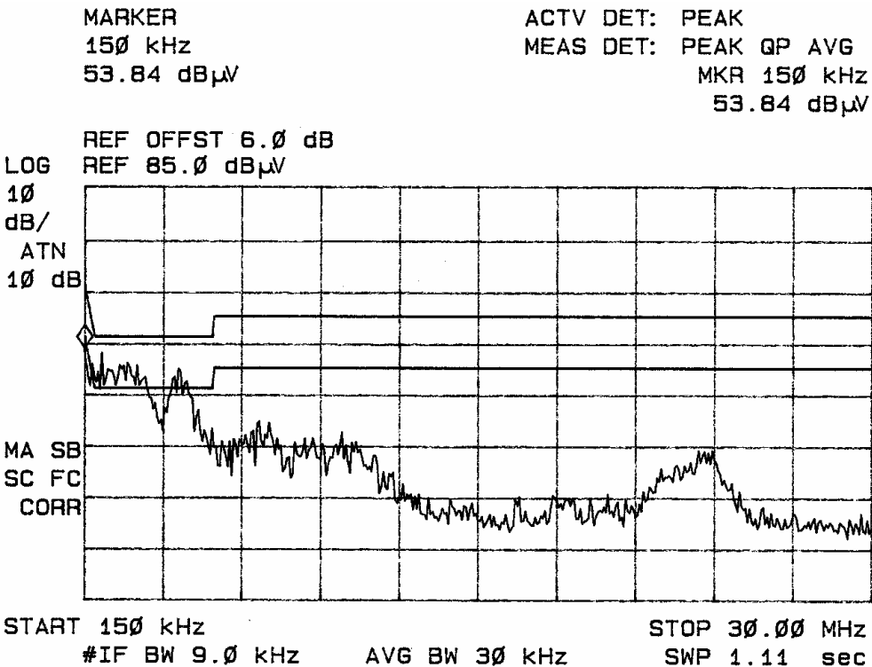
Figure two Conducted emissions of EUT line 2 (320-00171-12)
