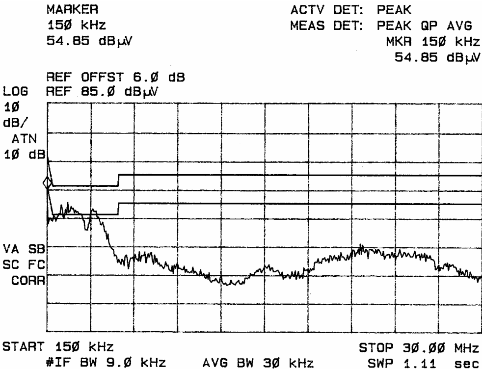
Figure Six Conducted emissions of EUT line 2 (320-00171-13)
