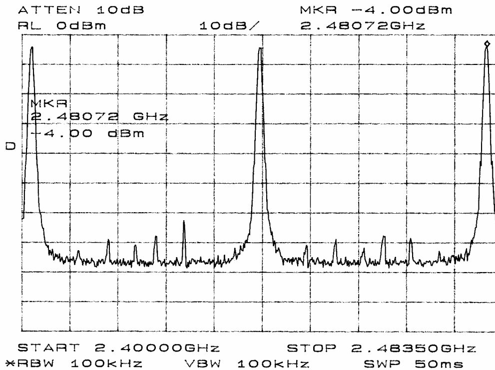
Figure twelve Power output measured at temporary antenna terminal
