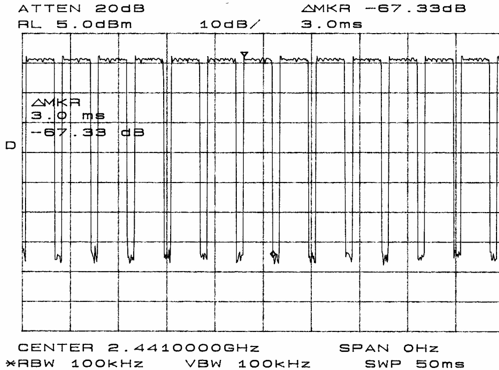
Figure thirteen Dwell Time of Occupancy
