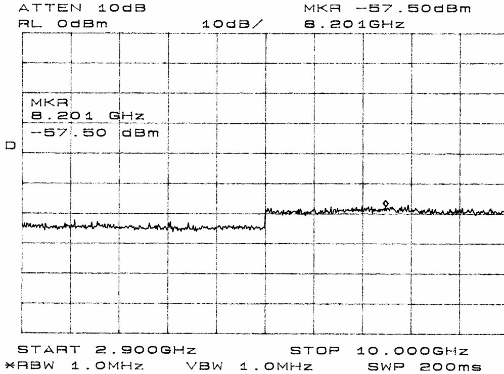
Figure nine Power output measured at temporary antenna terminal
