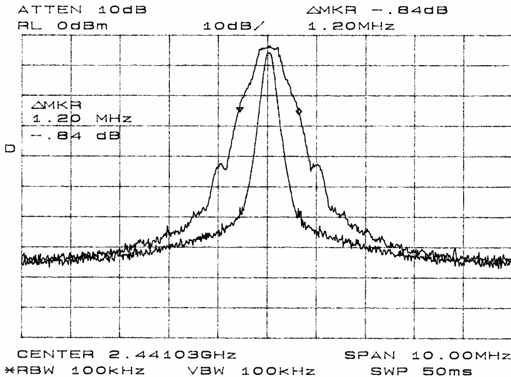
Figure fourteen Occupied bandwidth
