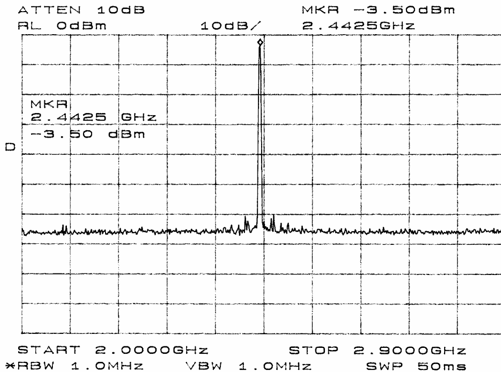
Figure eight Power output measured at temporary antenna terminal
