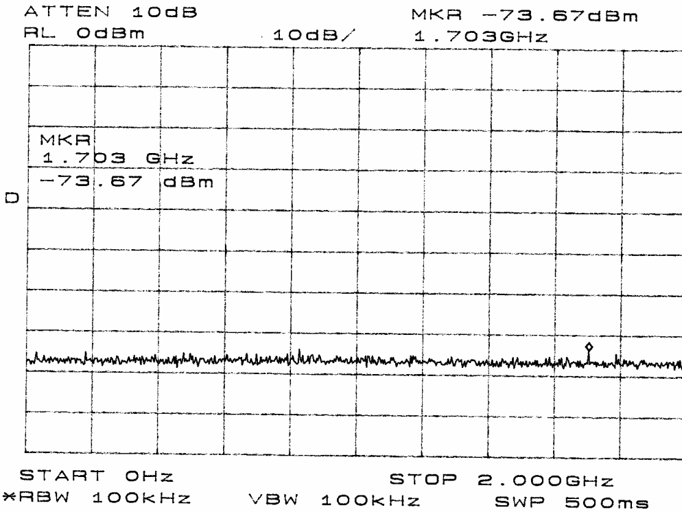
Figure seven Power output measured at temporary antenna terminal
