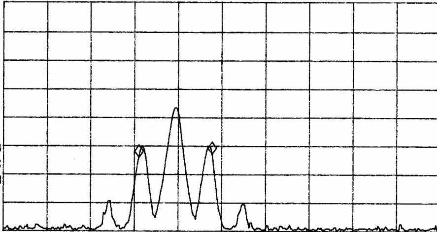
Figure fourteen Band Edges of operation (at 88.1 MHz)
