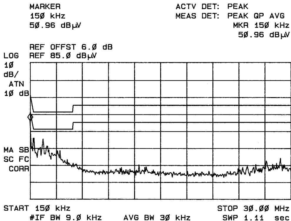
Figure five Conducted emissions of EUT line 1 (Jet (USB))
