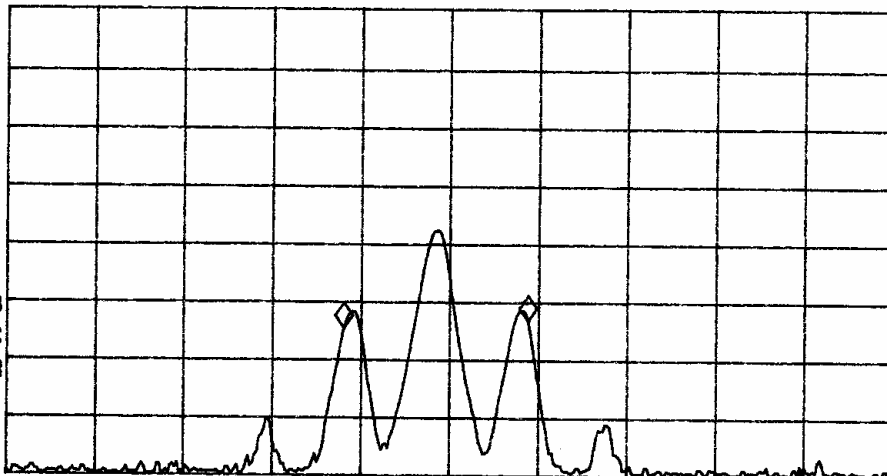
Figure sixteen 200 kHz Occupied Bandwidth requirement
