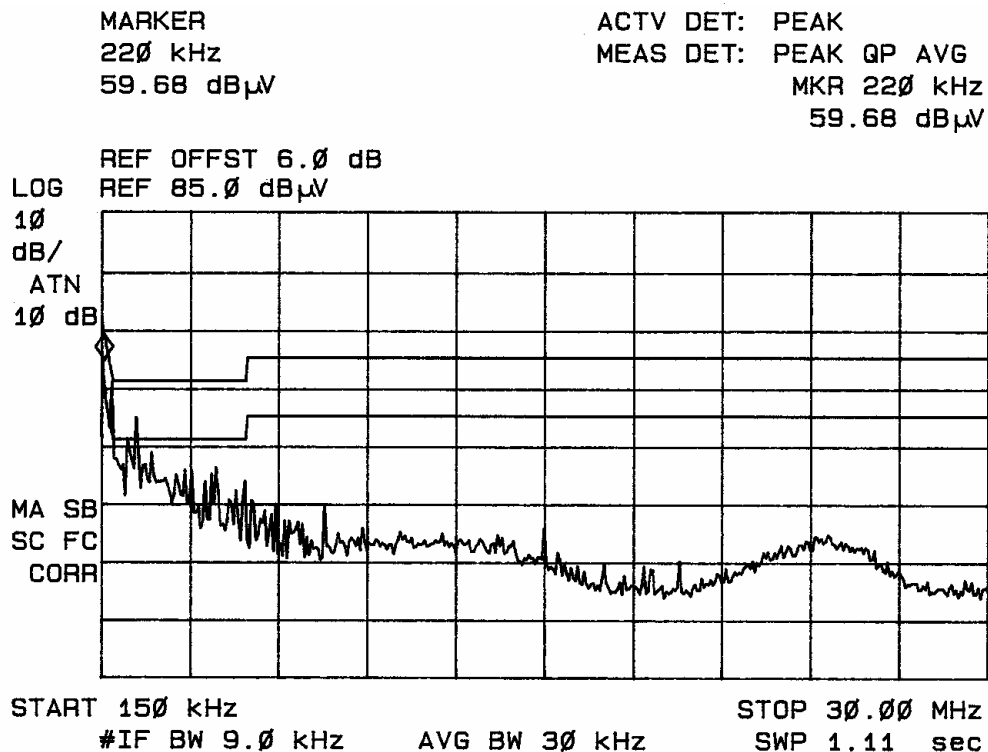
Figure two Conducted emissions of EUT line 2 (Jet)
