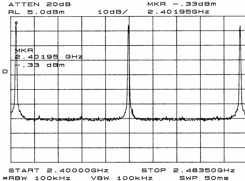
Figure twenty-five Power output measured at temporary antenna terminal
