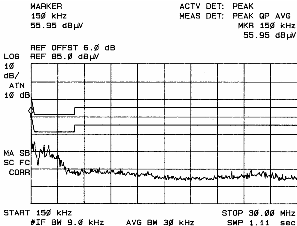
Figure Six Conducted emissions of EUT line 2 (Jet (USB))
