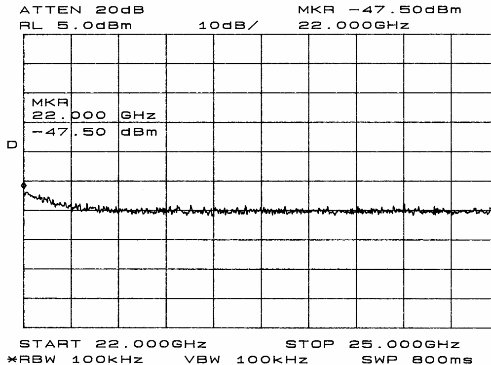
Figure twenty-four Power output measured at temporary antenna terminal
