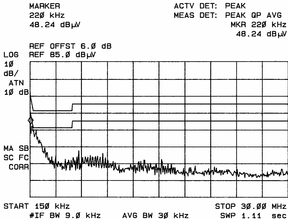
Figure eight Conducted emissions of EUT line 2 (CPU)
