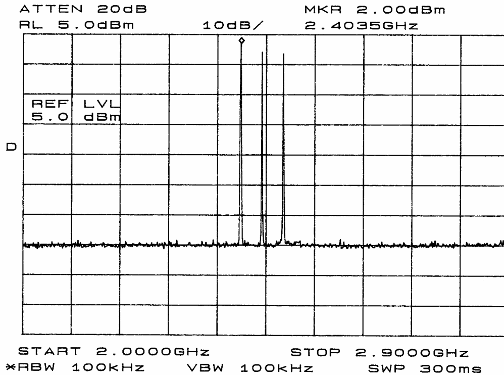
Figure twenty-one Power output measured at temporary antenna terminal
