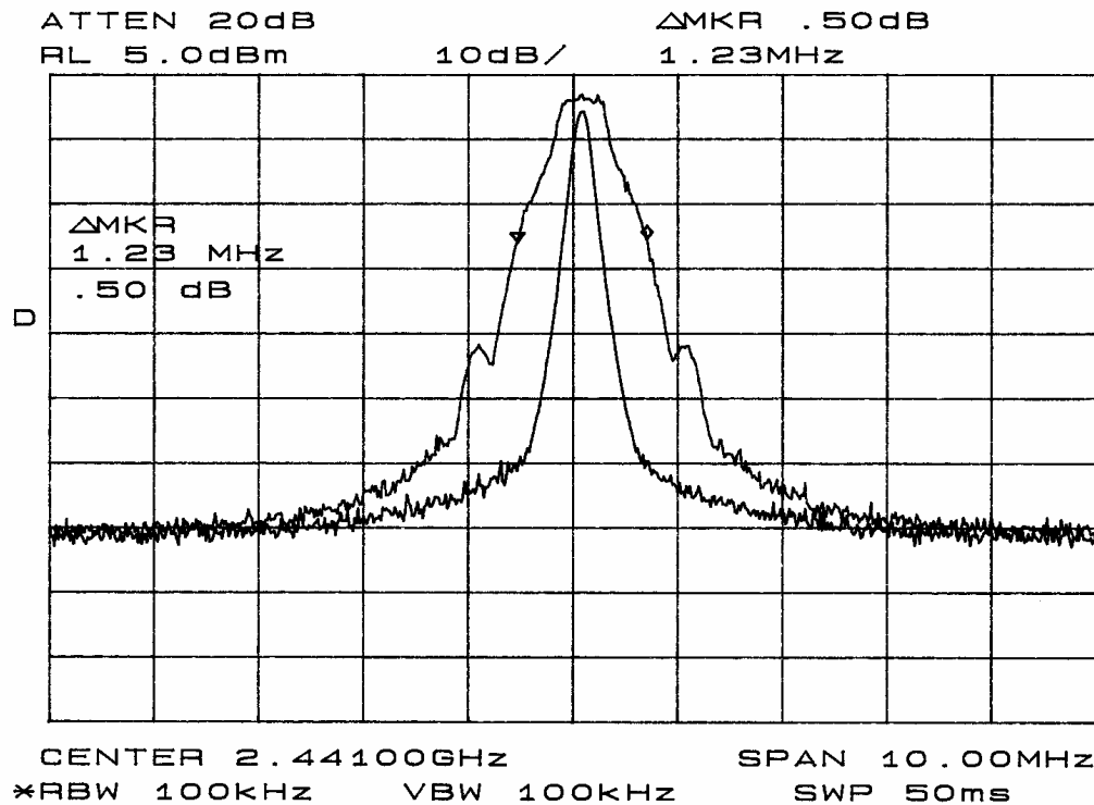
Figure twenty-six Occupied Bandwidth
