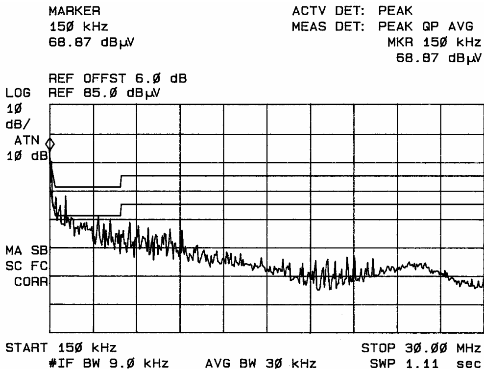
Figure one Conducted emissions of EUT line 1 (Jet)
