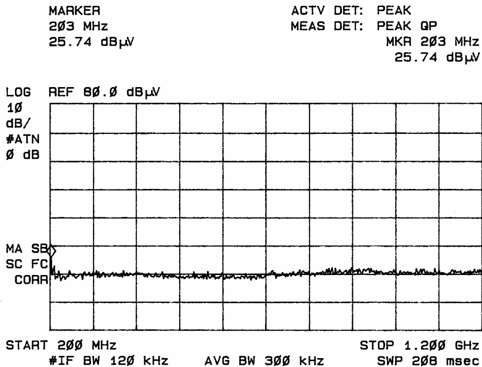
Figure nineteen Radiated Emissions @ 1 Meter in Screen Room
