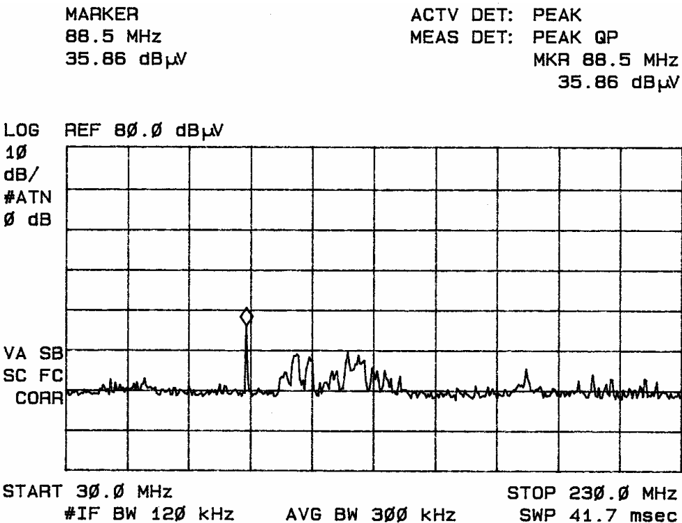
Figure eighteen Radiated Emissions @ 1 Meter in Screen Room
