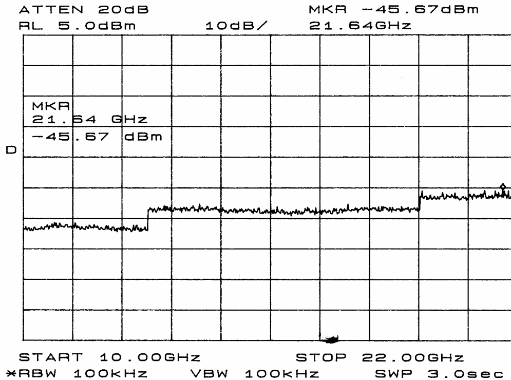
Figure twenty-three Power output measured at temporary antenna terminal
