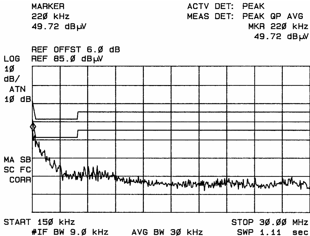
Figure seven Conducted emissions of EUT line 1 (CPU)
