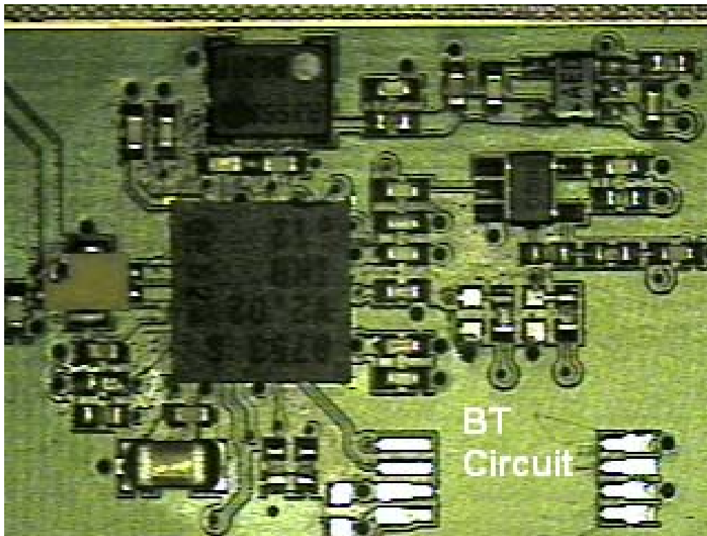
Transmitter board.
