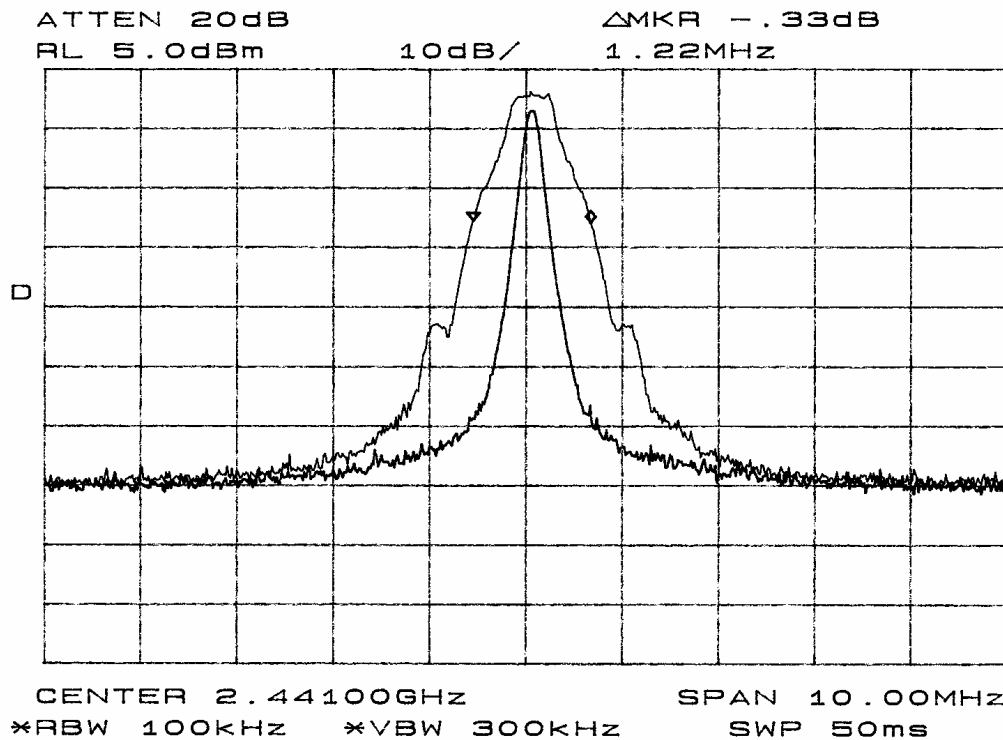
Figure sixteen Occupied bandwidth
