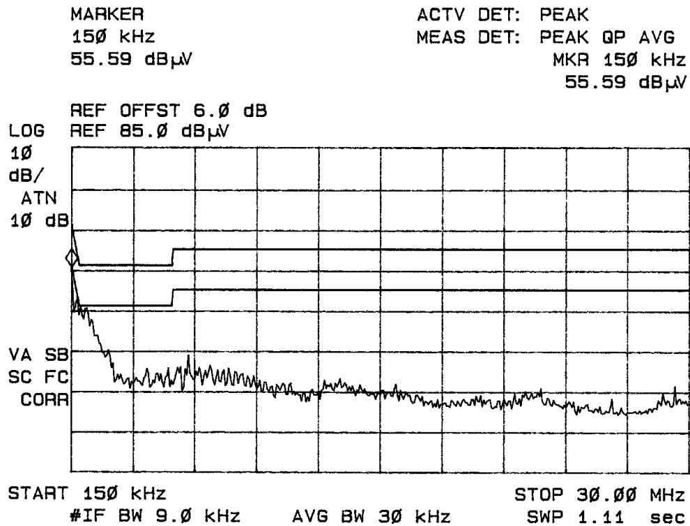
Figure four Conducted emissions of CPU and EUT line 2
