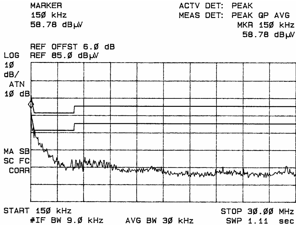
Figure three Conducted emissions of CPU and EUT line 1
