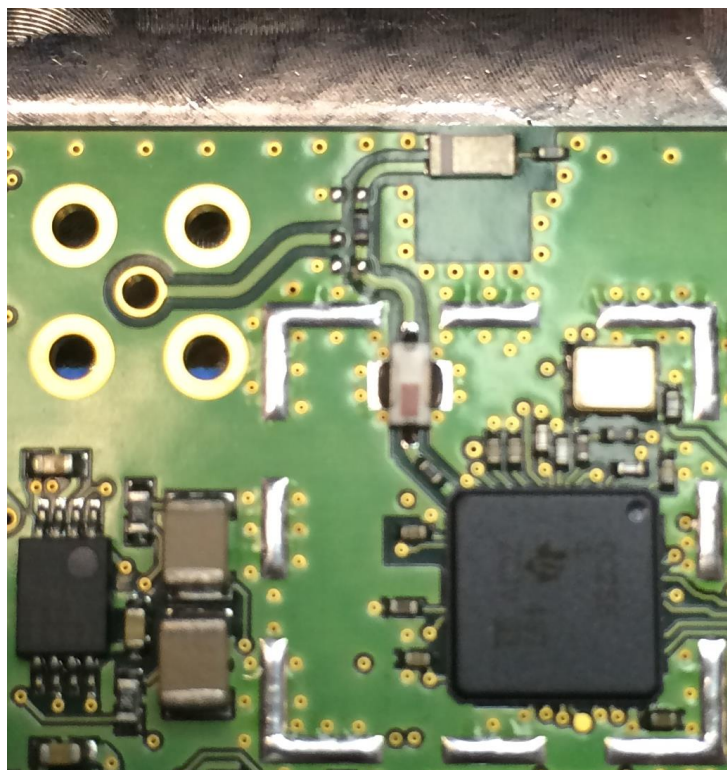
GMA 350c/350Hc/350Hc Traffic Transceiver Circuitry
