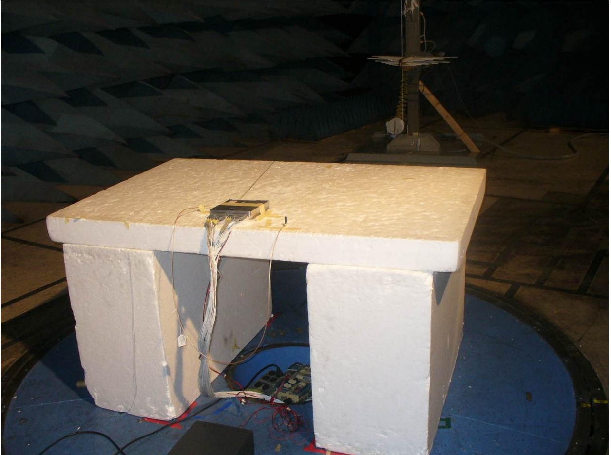
Figure 5: Radiated Emissions – Back View (GMN-00831) 200 MHz – 1 GHz
