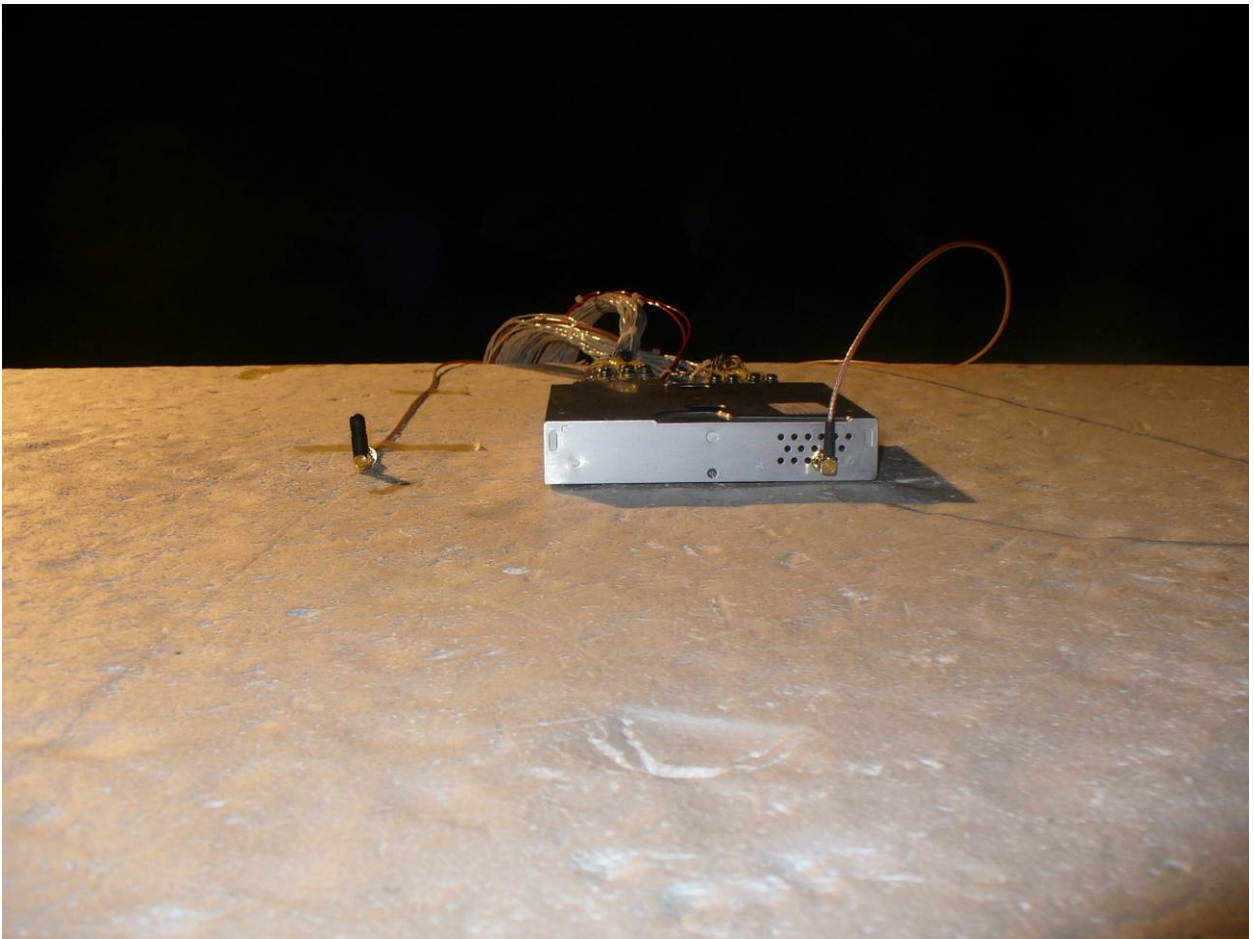
Figure 1: Radiated Emissions – Front View (GMN-00831)
