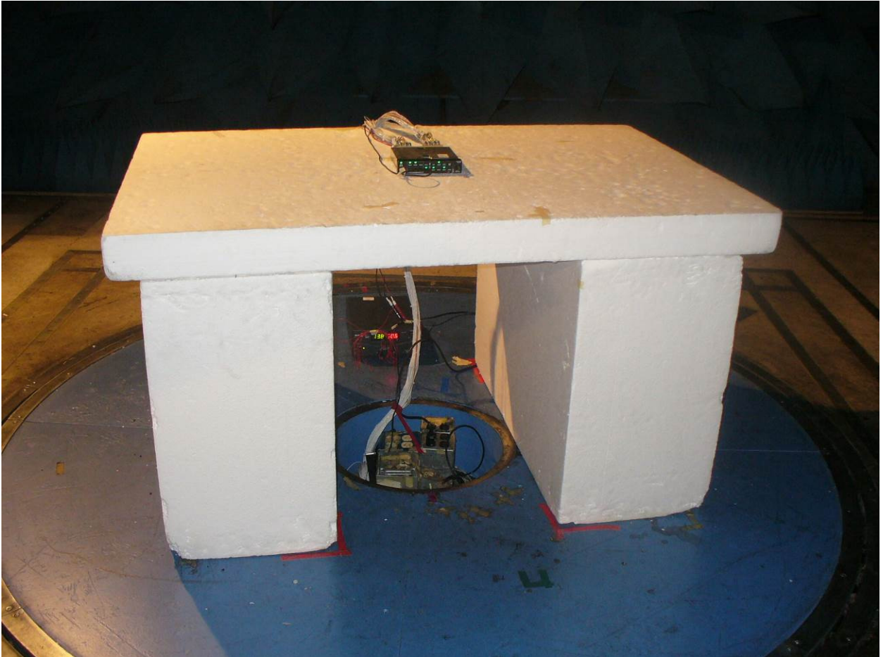
Figure 7: Radiated Emissions – Back View (GMN-00871) below 1GHz
