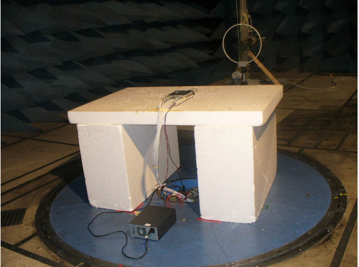
Figure 8: Radiated Emissions – Back View (GMN-00871) below 30 MHz
