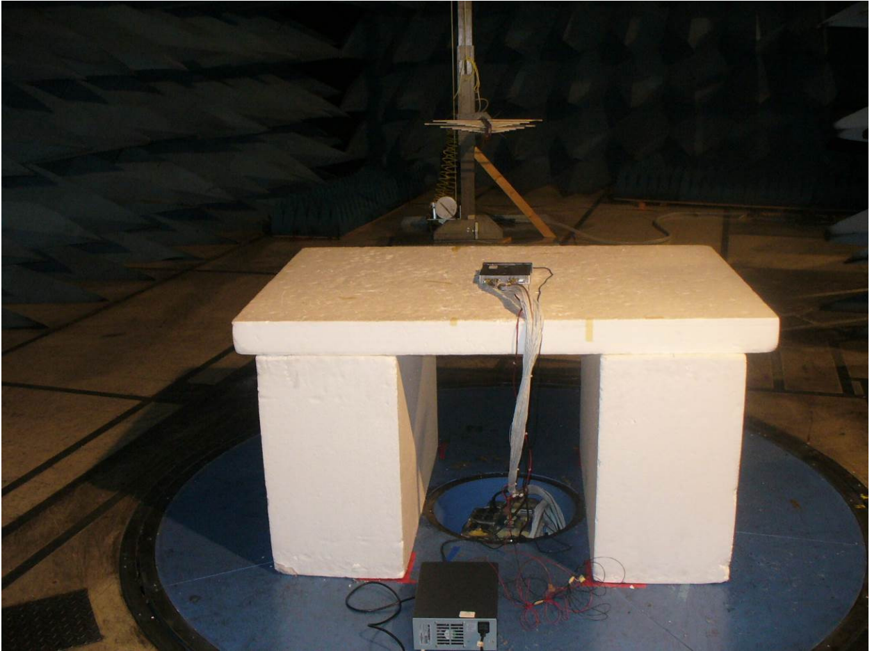
Figure 10: Radiated Emissions – Back View (GMN-00871) 200MHz - 1GHz
