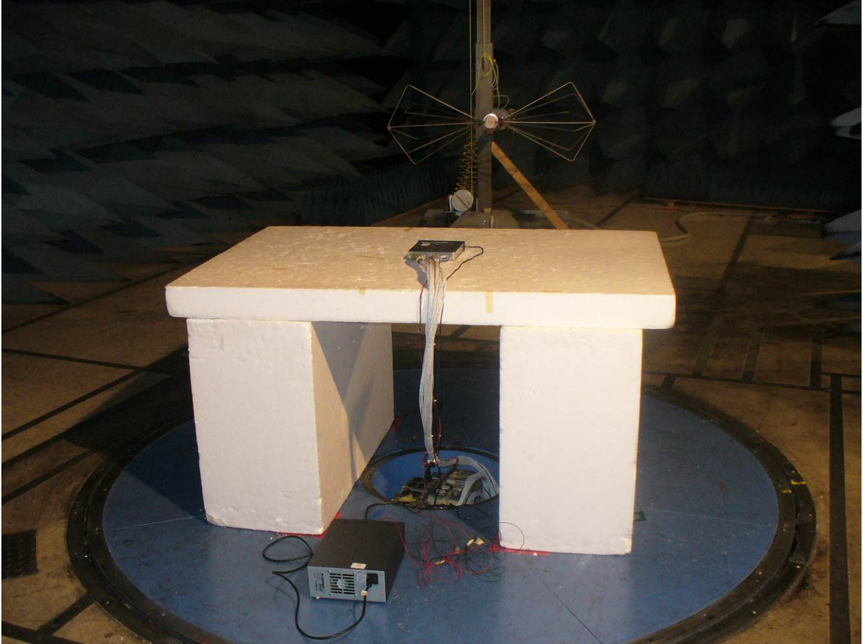
Figure 9: Radiated Emissions – Back View (GMN-00871) above 30 MHz – 200 MHz
