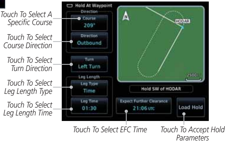
Figure 5-12 Entering Direct-To Hold Parameters
