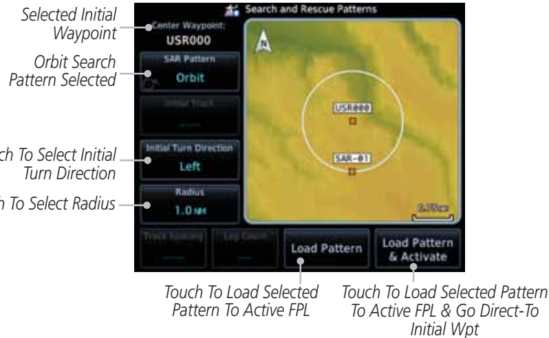
Figure 4-34 Search and Rescue Orbit Pattern Page
