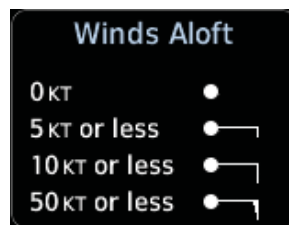
Figure 12-37 Winds Aloft Legend
