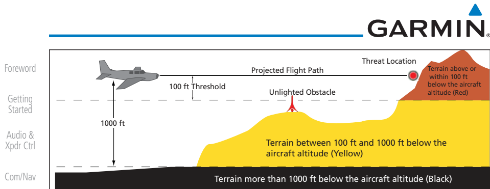
Figure 11-6 Terrain Altitude/Color Correlation for TAWS-B
