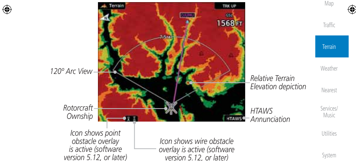
Figure 11-18 Terrain/HTAWS Page
