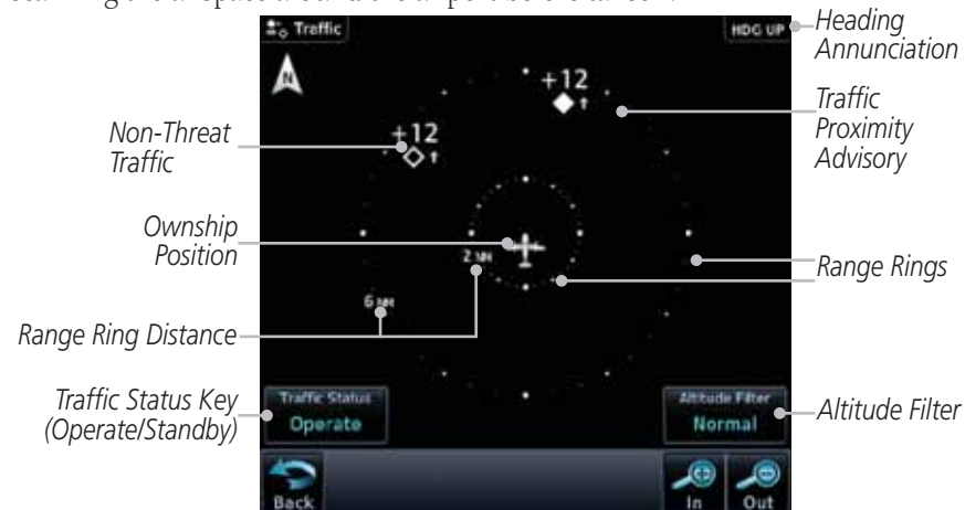
Figure 10-8 Traffic Page
