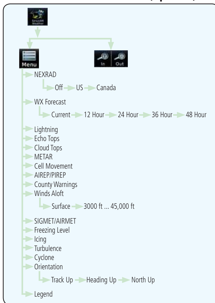
Figure 12-3 SiriusXM Weather Functional Diagram
