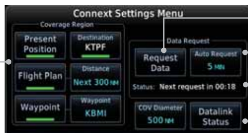
Figure 12-74 Connex Settings Menu
