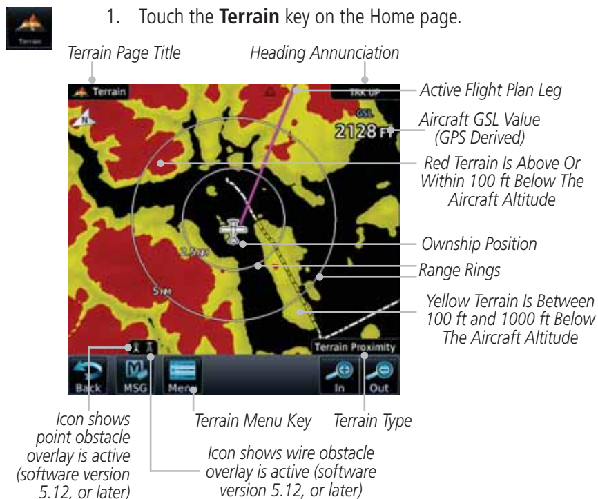
Figure 11-2 Terrain Page
