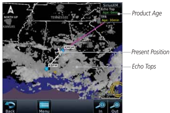
Figure 12-15 Echo Tops
