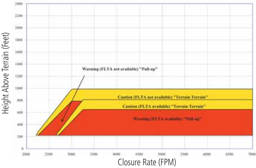
Figure 11-37 Excessive Closure Rate Alert Criteria (Flaps in Landing Configuration)
