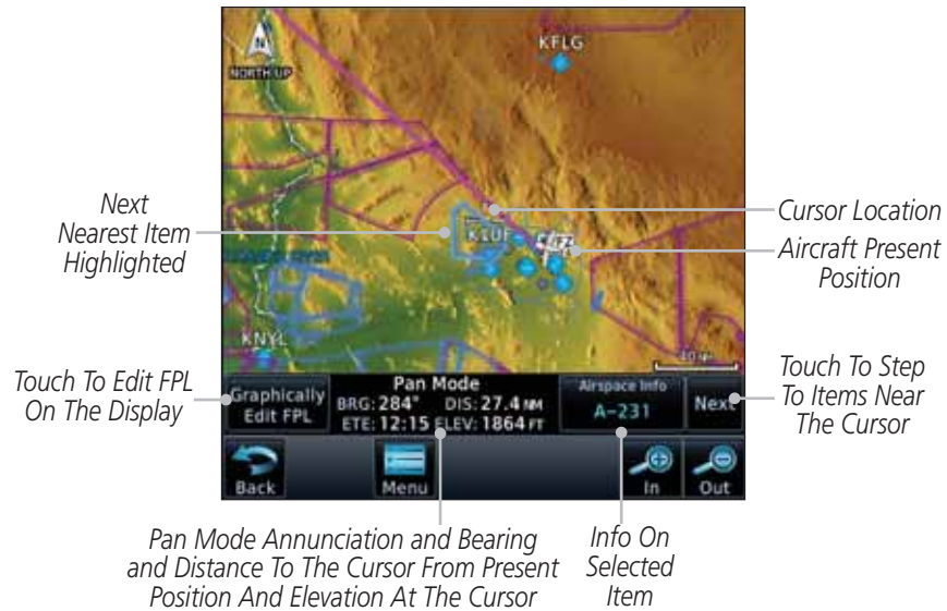
Figure 9-33 Map Panning With Next Airspace Shown
