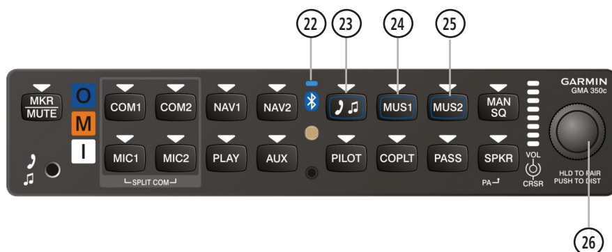
GMA 350c (Bluetooth) Controls
