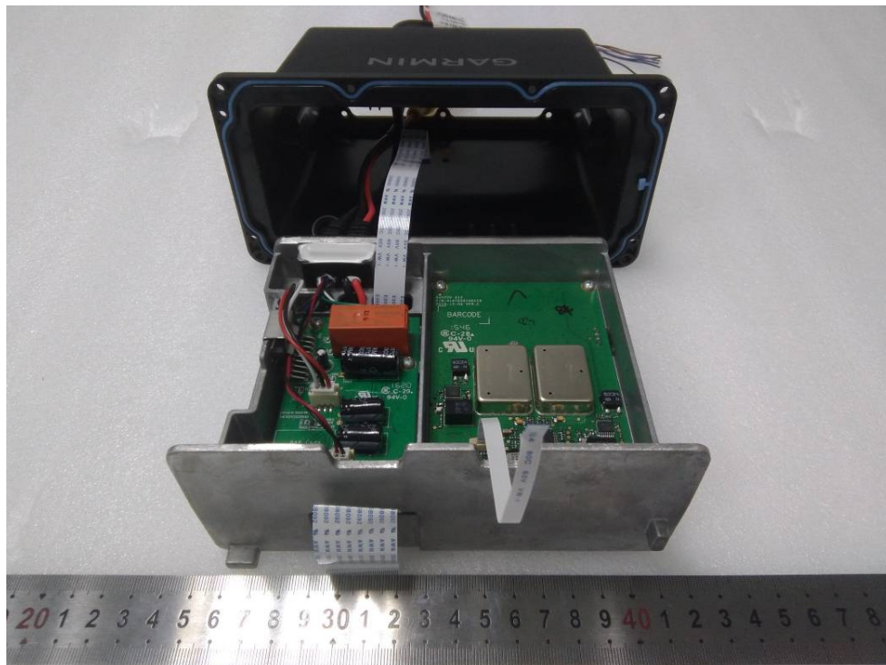
EUT – Cover off View 4
