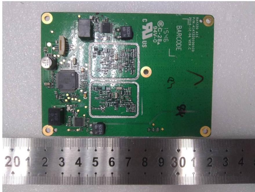
EUT – Main Board Top 3 Shilding off View
