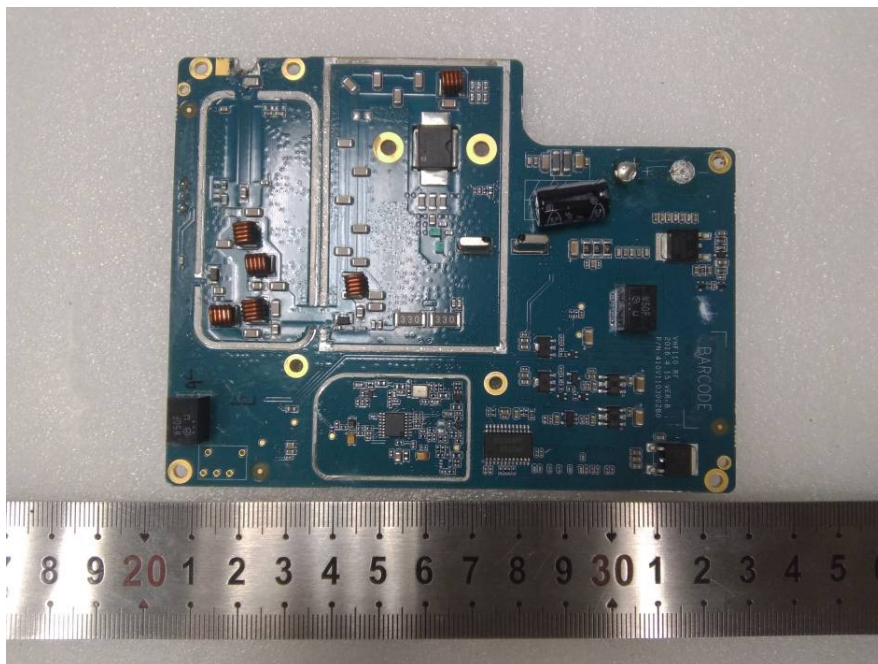
EUT – Main Board Bottom 5 Shilding off View
