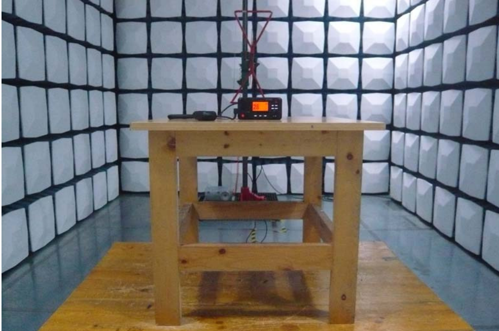
Transmitting Radiated Emissions (Below 1 GHz)
