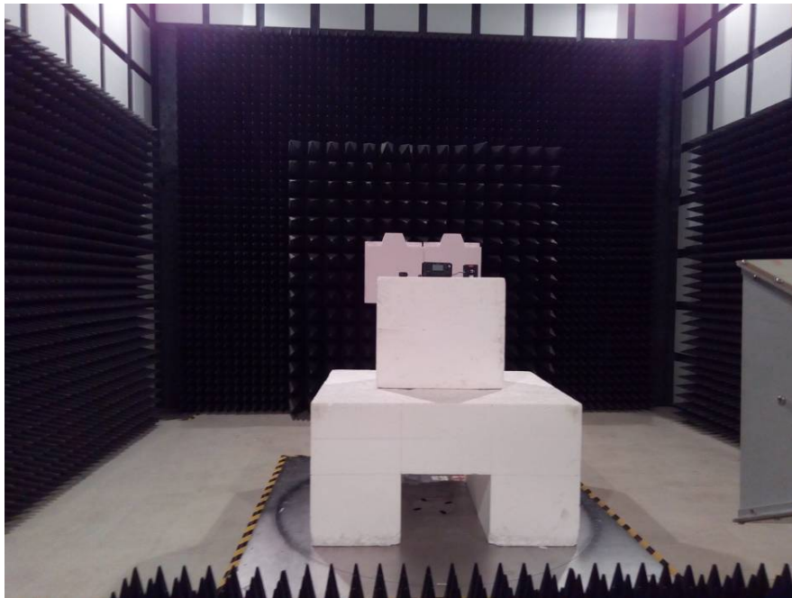
Transmitting Radiated Emissions Tested View (Above 1 GHz)
