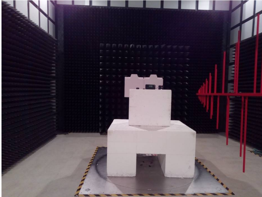
Transmitting Radiated Emissions Tested View (Below 1 GHz)
