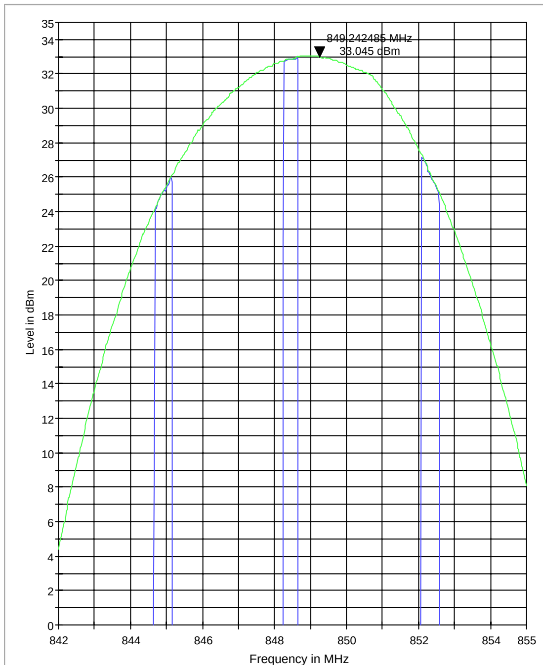
ERP 850 H
