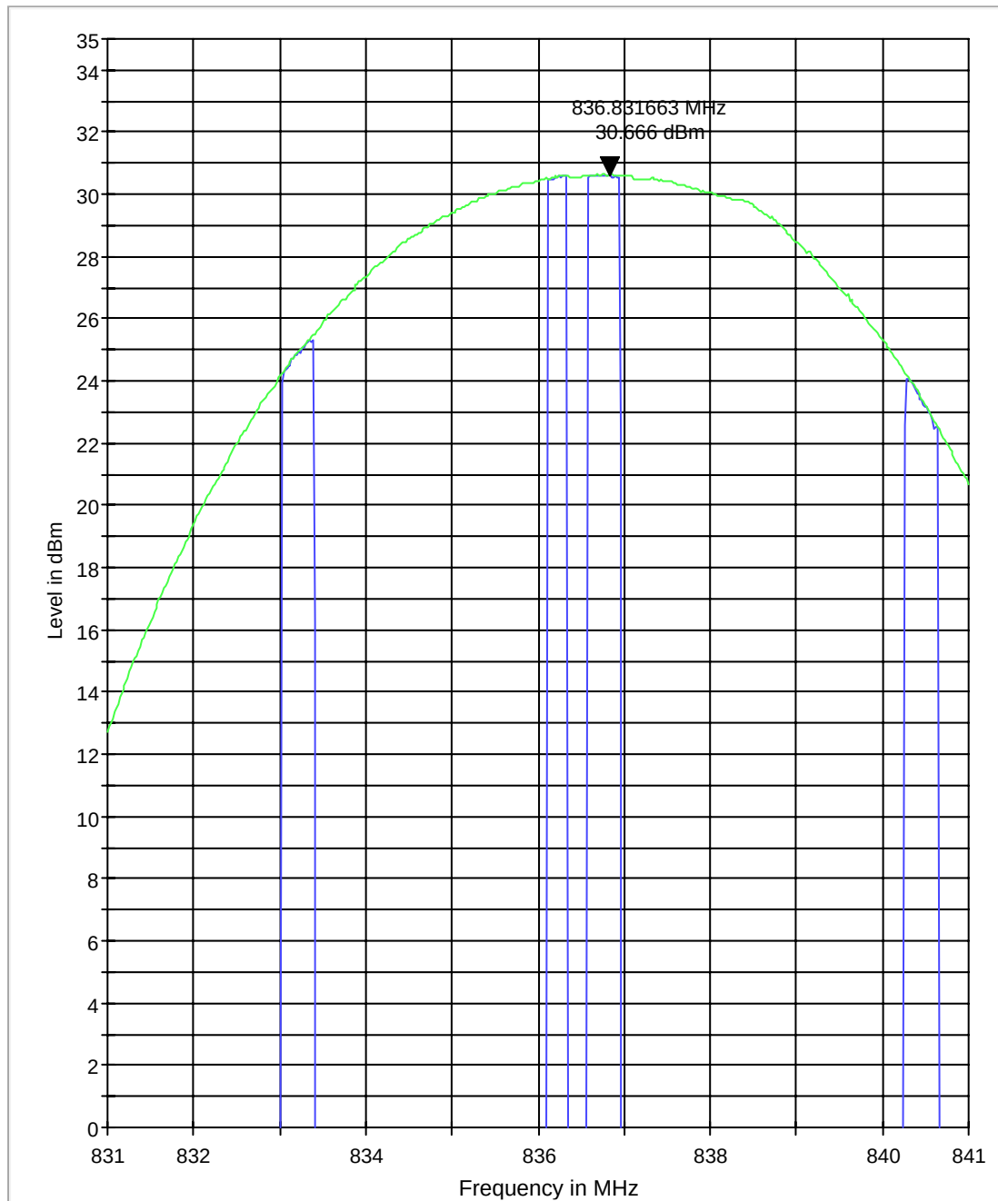
ERP 850 M
