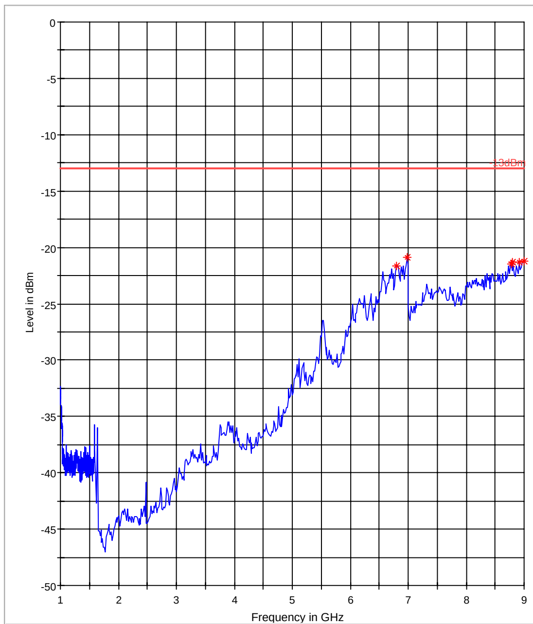
FCC 22 1-9GHz
