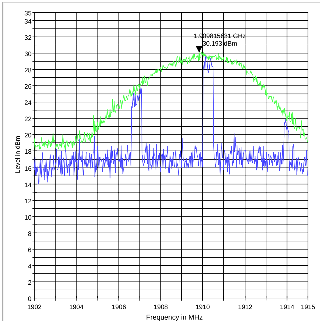
EIRP 1900 H
