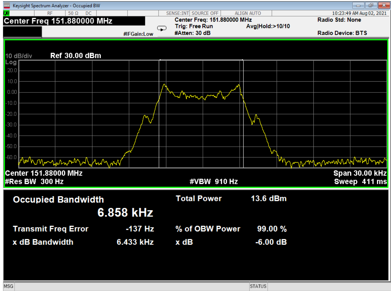
Figure 10 - Bandwidth, 151.880 MHz
