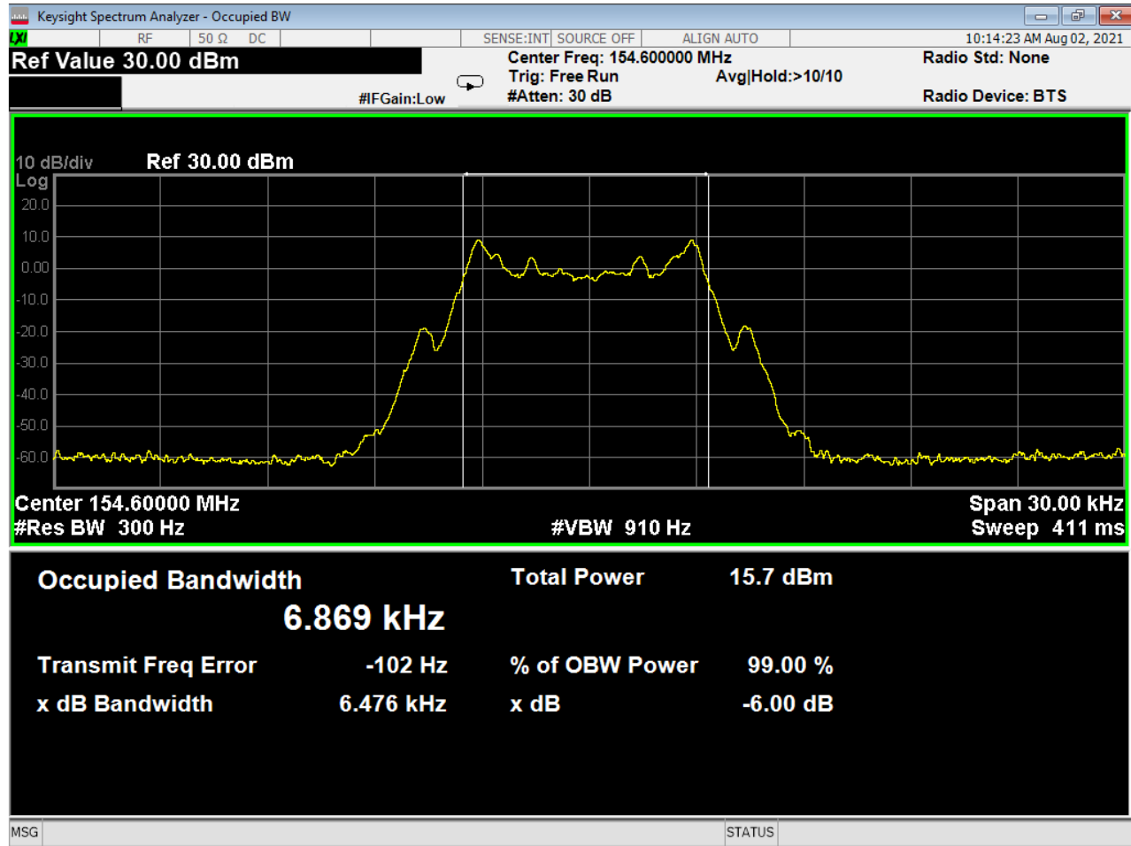
Figure 13 - Bandwidth, 154.600 MHz
