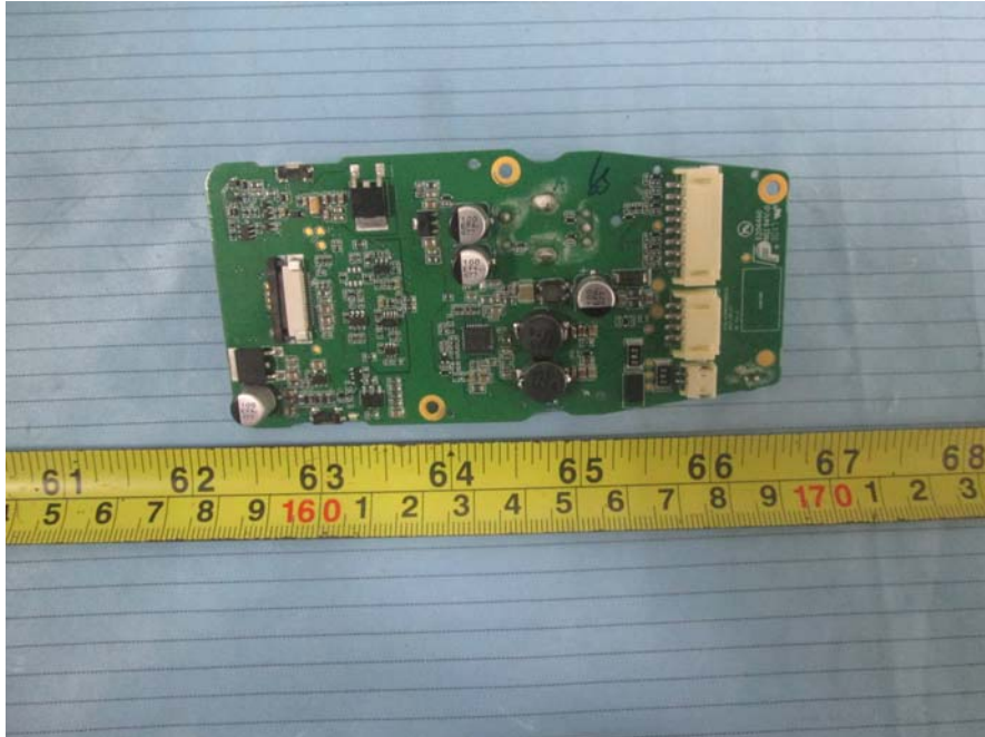
EUT (Handset) – Main Board Bottom View
