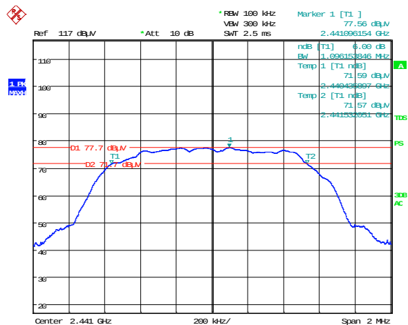
Figure 8.1-8: 6 dB bandwidth on mid channel
