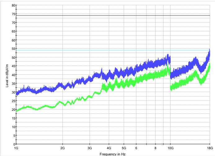
Figure 8.3-6: Radiated spurious emissions for BT, high channel – 1 to 18 GHz
