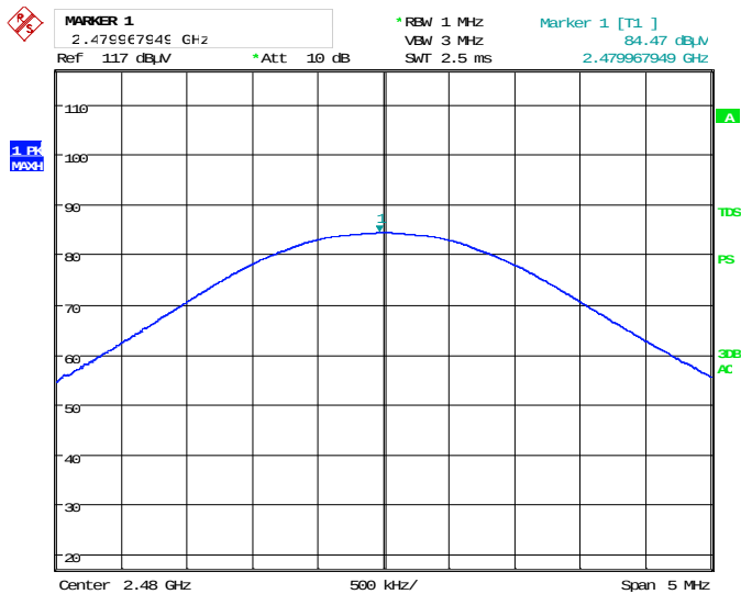
Figure 8.2-6: Output power on high channel
