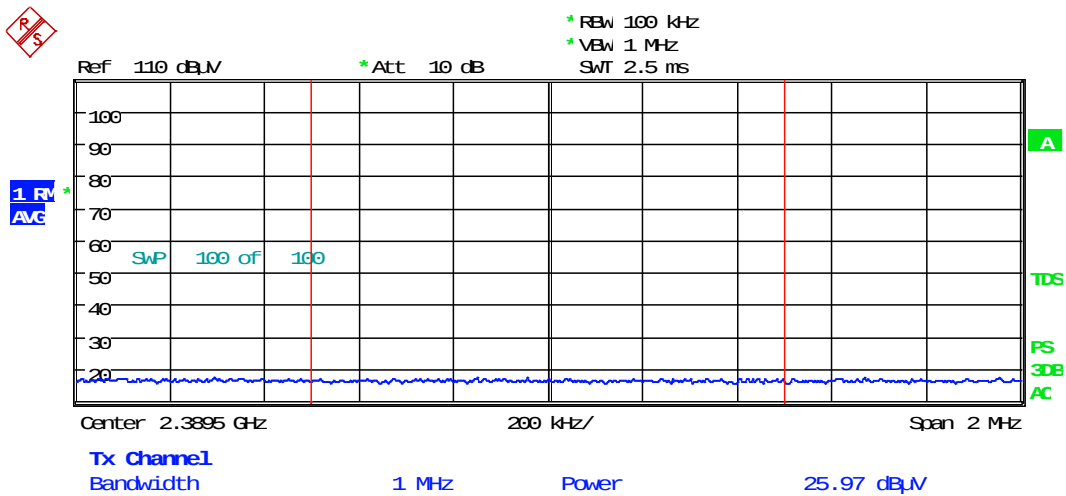
Figure 8.3-15: Radiated spurious (out-of-band) emissions Lower band edge emission, low channel_Avg
