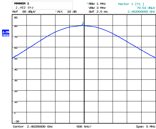
Figure 8.2-1: Output power on low channel
