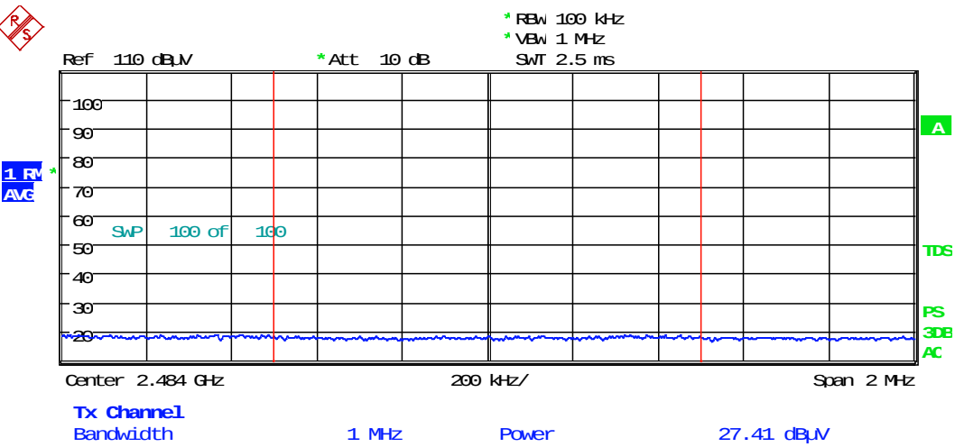
Figure 8.3-16: Radiated spurious (out-of-band) emissions Upper band edge emission -Avg
