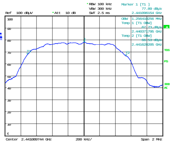
Figure 8.1-5: 99% bandwidth on mid channel
