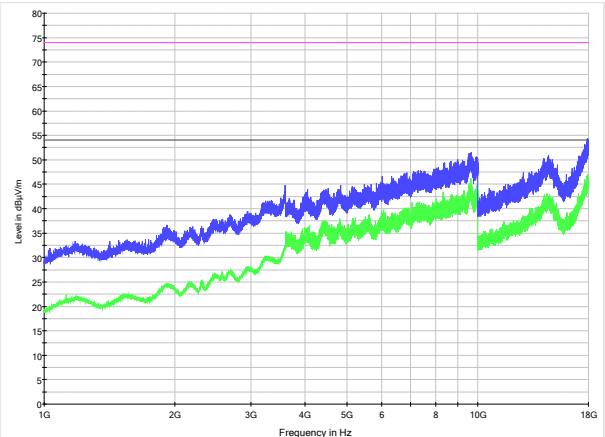
Figure 8.3-5: Radiated spurious emissions for BT, mid channel – 1 to 18 GHz
