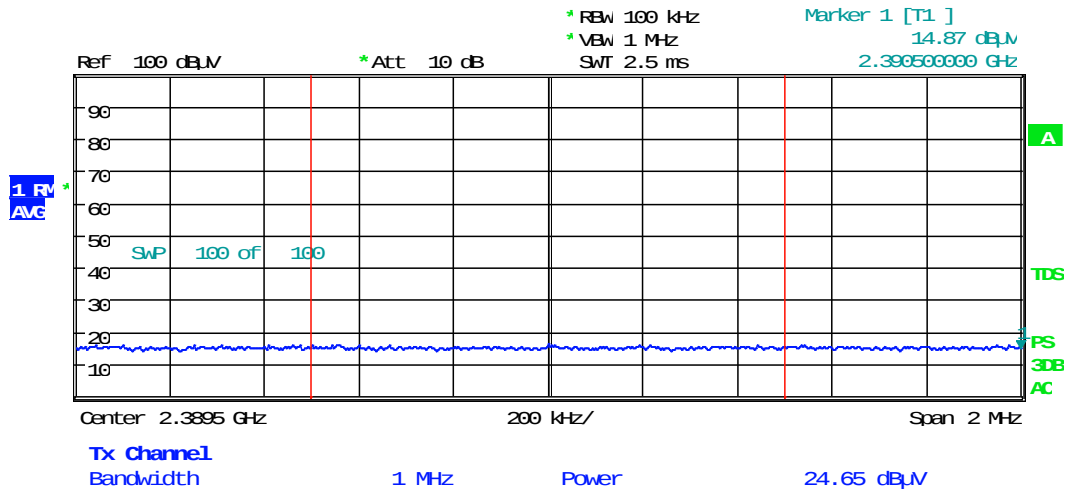
Figure 8.3-9: Radiated spurious (out-of-band) emissions Lower band edge emission, low channel_Avg
