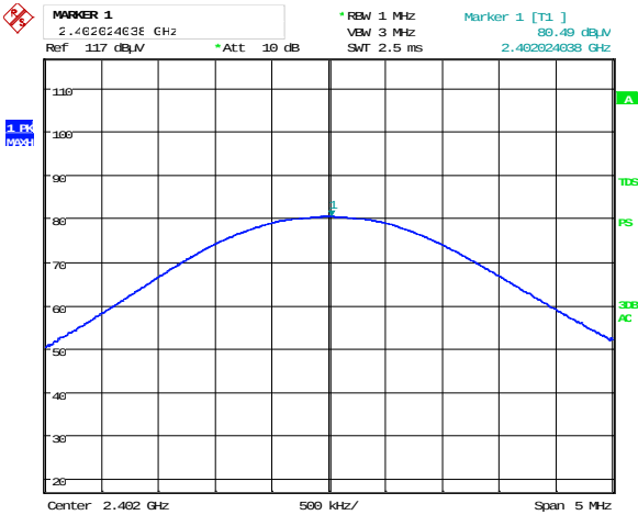
Figure 8.2-4: Output power on low channel
