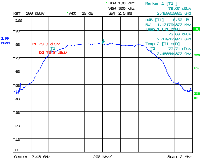
Figure 8.1-3: 6 dB bandwidth on high channel
