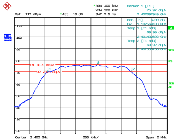
Figure 8.1-7: 6 dB bandwidth on low channel
