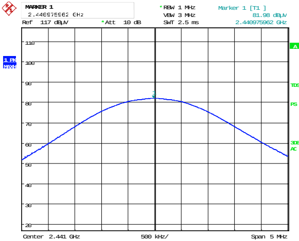
Figure 8.2-5: Output power on mid channel
