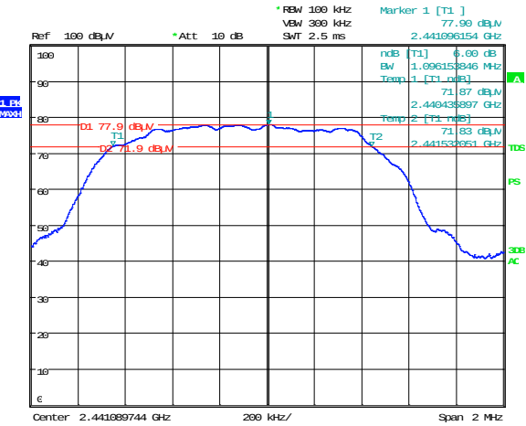
Figure 8.1-2: 6 dB bandwidth on mid channel
