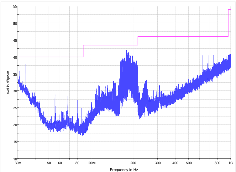
Figure 8.3-3: Radiated spurious (out-of-band) emissions, high channel, 30 to 1000 MHz
