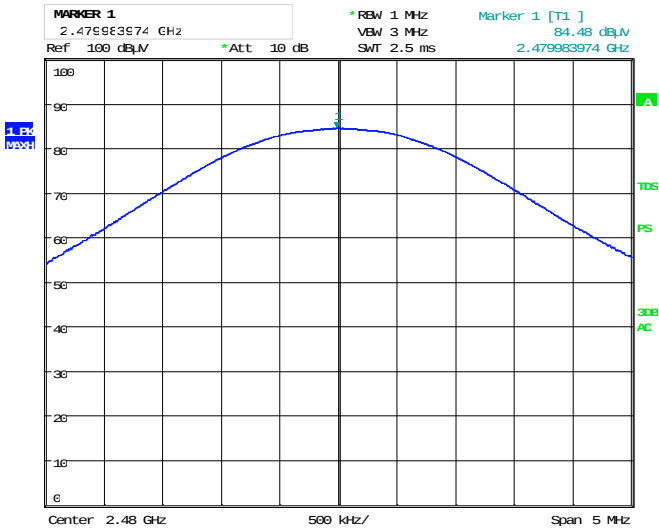
Figure 8.2-3: Output power on high channel
