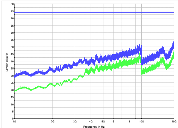
Figure 8.3-4: Radiated spurious emissions for BT, low channel – 1 to 18 GHz
