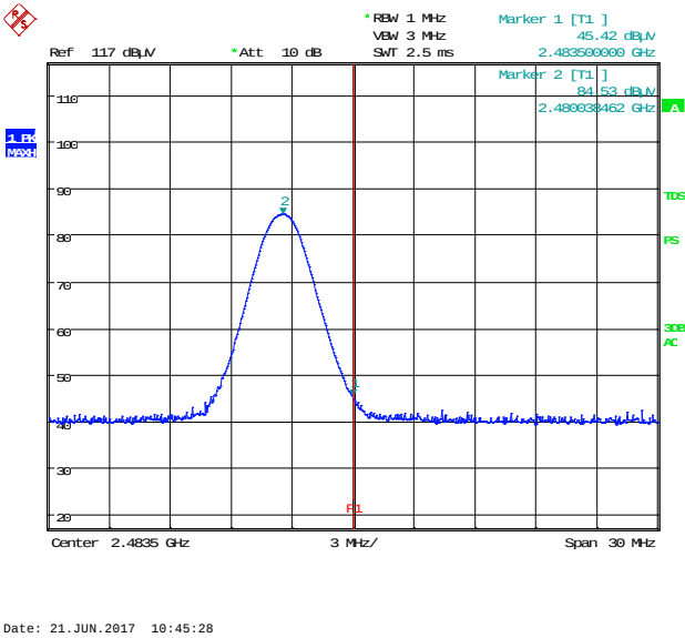
Figure 8.3-14: Conducted spurious (out-of-band) emissions upper band, high channel
