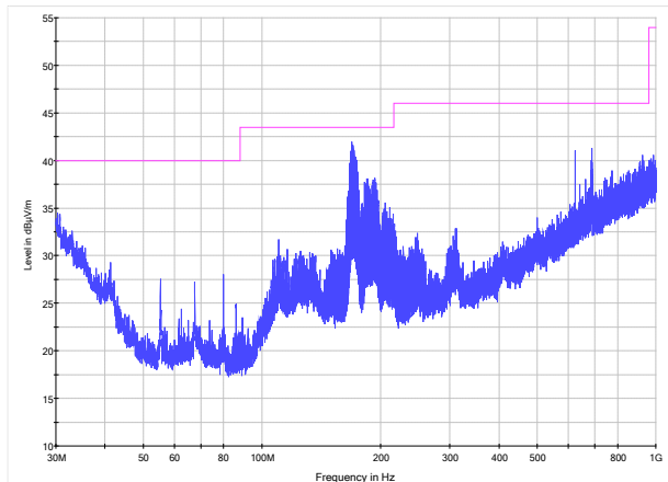
Figure 8.3-1: Radiated spurious (out-of-band) emissions, low channel, 30 to 1000 MHz
