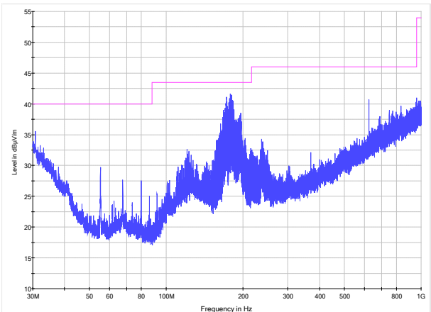
Figure 8.3-2: Radiated spurious (out-of-band) emissions, mid channel, 30 to 1000 MHz
