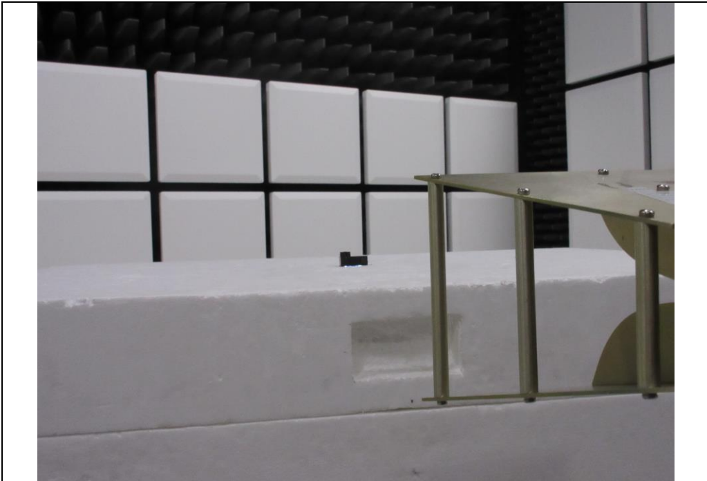
RF Radiated #4
