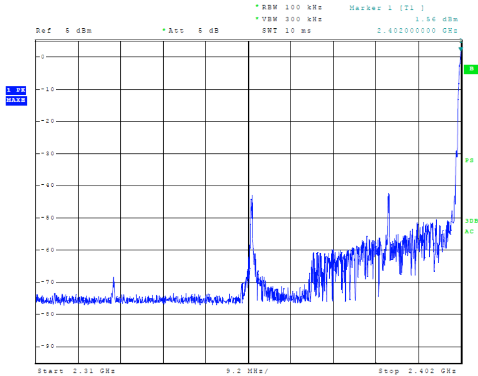
Figure 17 Plot of Transmitter Emissions (Low Band Edge, Mode 2)
