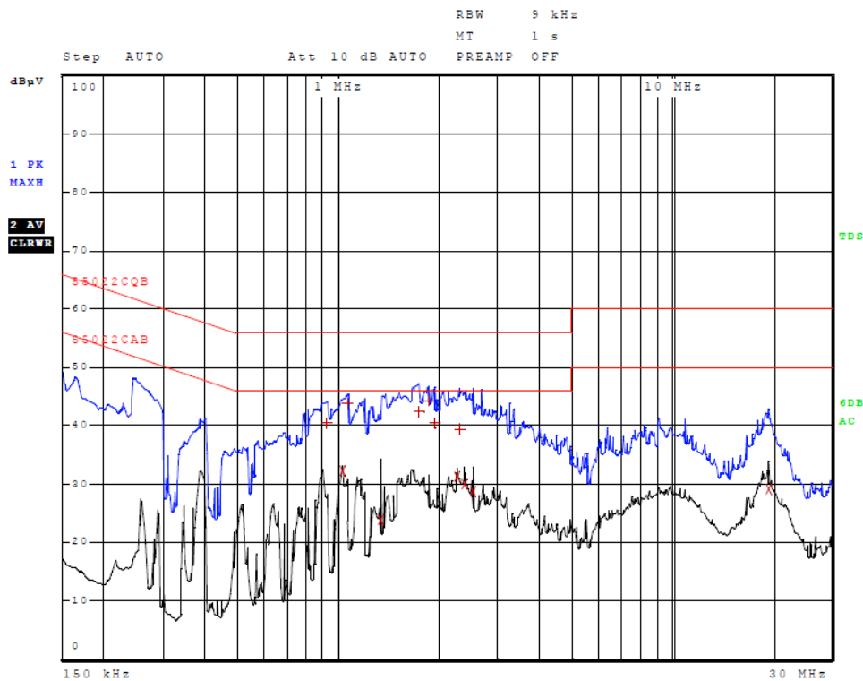
Figure 10 AC Line Conducted emissions of EUT line 2 (EUT-USB-CPU AC Adapter)
