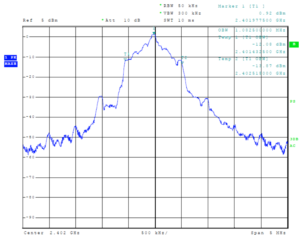
Figure 16 Plot of Transmitter Emissions (2402-2480 MHz, 99% Occupied Bandwidth, Mode 2)
