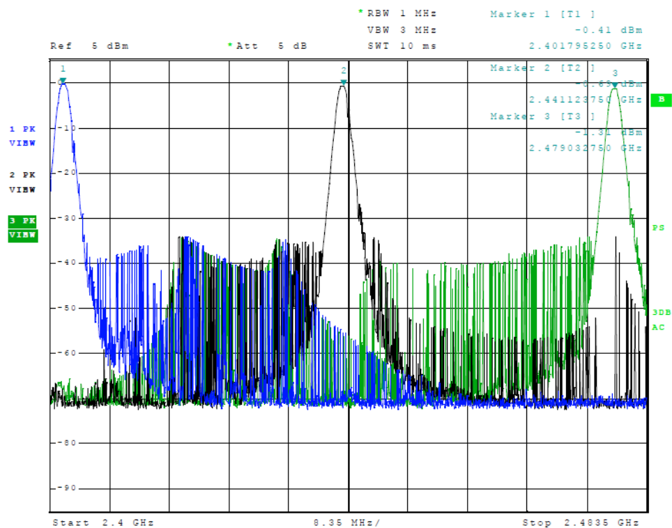
Figure 11 Plot of Transmitter Emissions (In 2402-2479 MHz Band, Mode 1)
