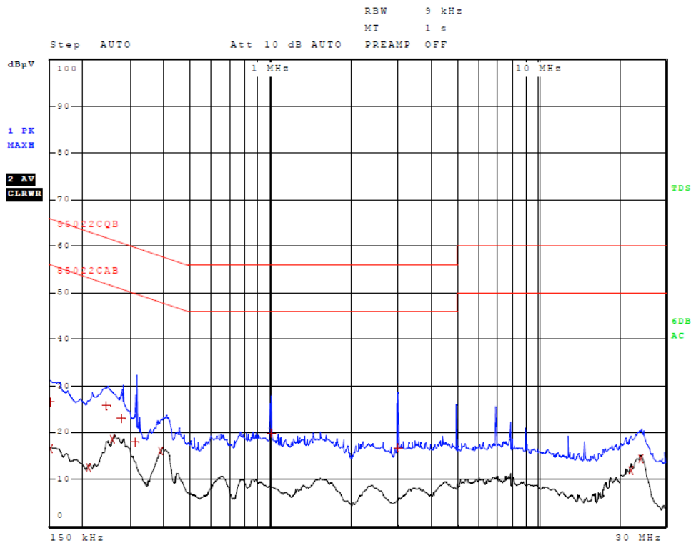
Figure 6 AC Line Conducted emissions of EUT line 2 (EUT AC Adapter 326-00086-01)
