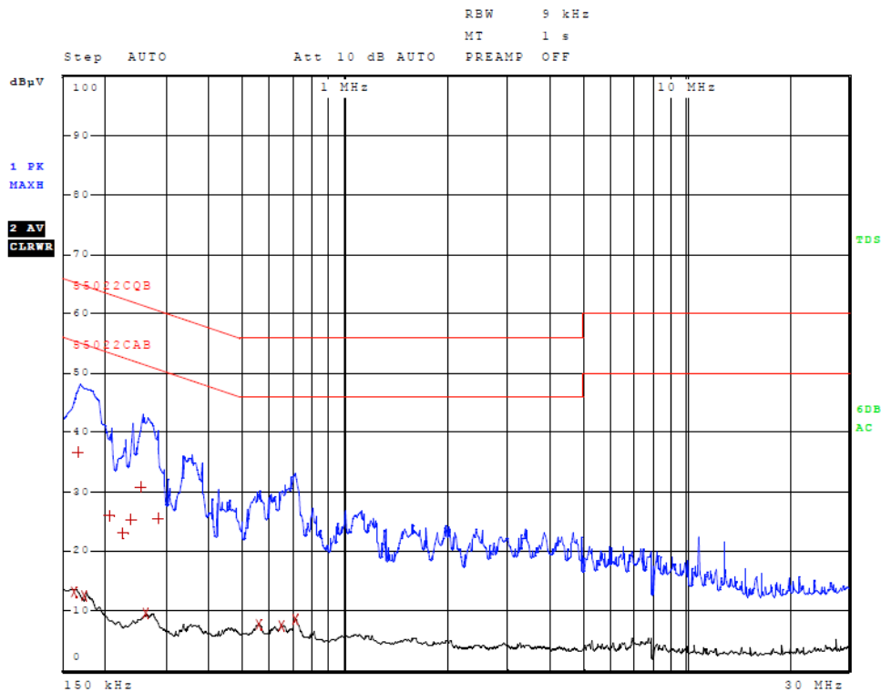
Figure 8 AC Line Conducted emissions of EUT line 2 (EUT AC Adapter 326-00087-00)
