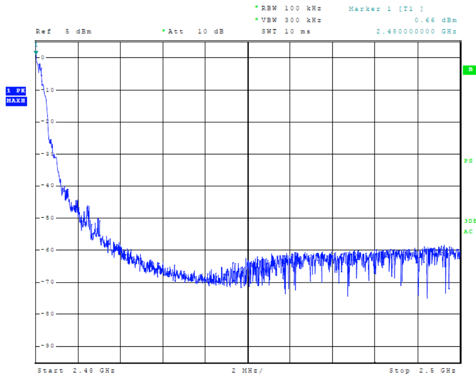
Figure 18 Plot of Transmitter Emissions (High Band Edge, Mode 1)
