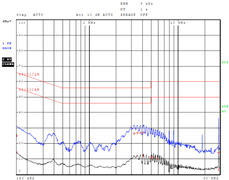
Figure 2 AC Line Conducted emissions of EUT line 2 (EUT AC Adapter SCB055600P)
