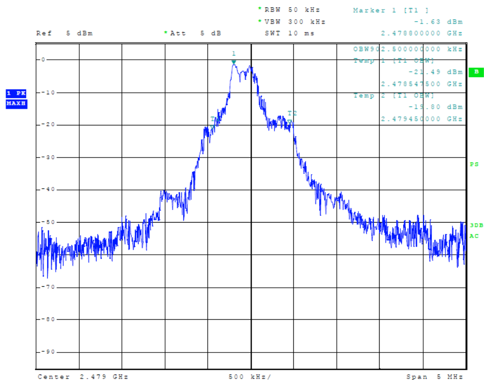
Figure 12 Plot of Transmitter Emissions (2402-2479 MHz, 99% Occupied Bandwidth, Mode 1)
