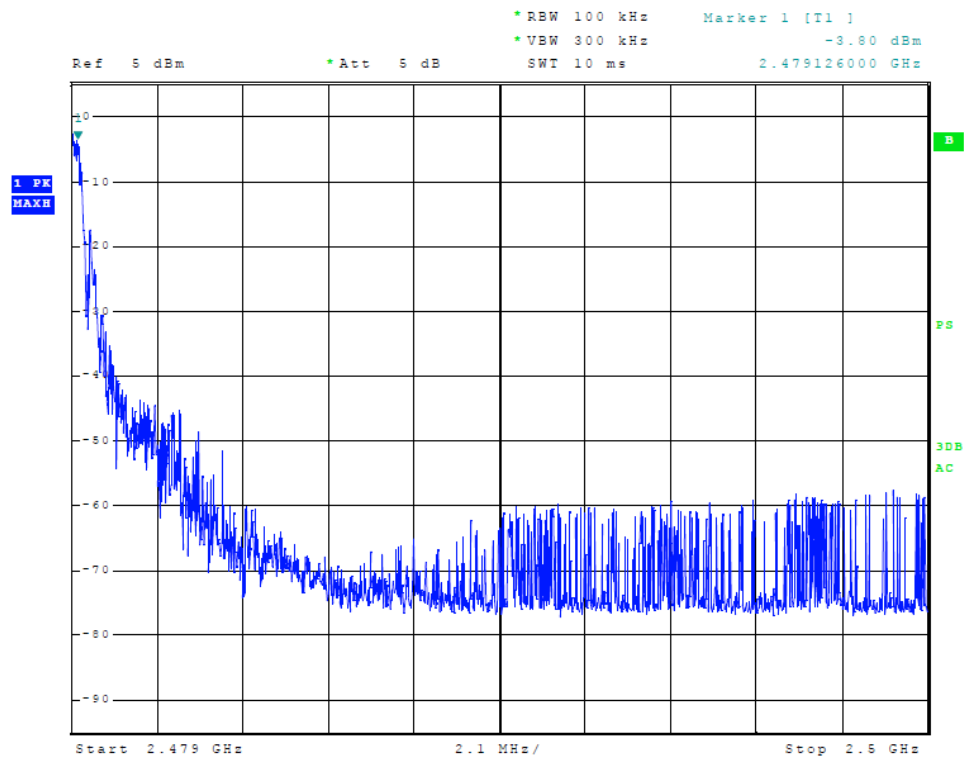
Figure 14 Plot of Transmitter Emissions (High Band Edge, Mode 1)
