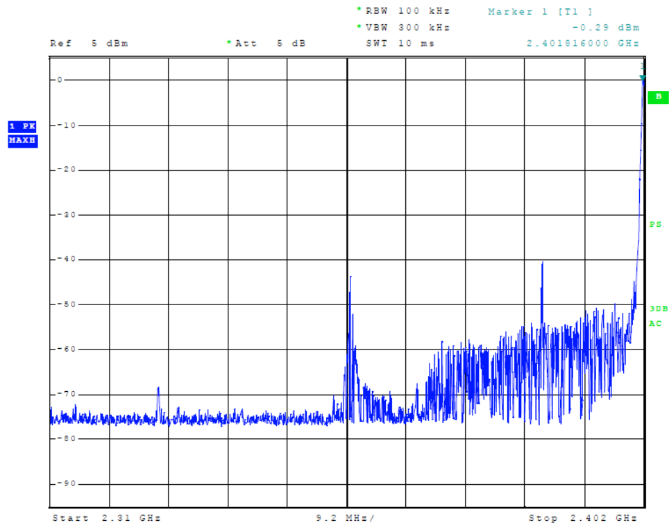
Figure 13 Plot of Transmitter Emissions (Low Band Edge, Mode 1)
