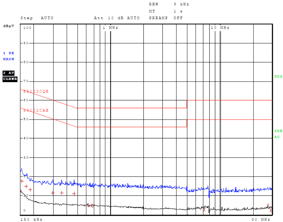
Figure 3 AC Line Conducted emissions of EUT line 1 (EUT AC Adapter 326-00072-00)
