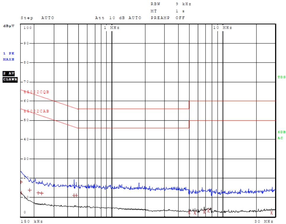
Figure 7 AC Line Conducted emissions of EUT line 1 (EUT AC Adapter 326-00087-00)
