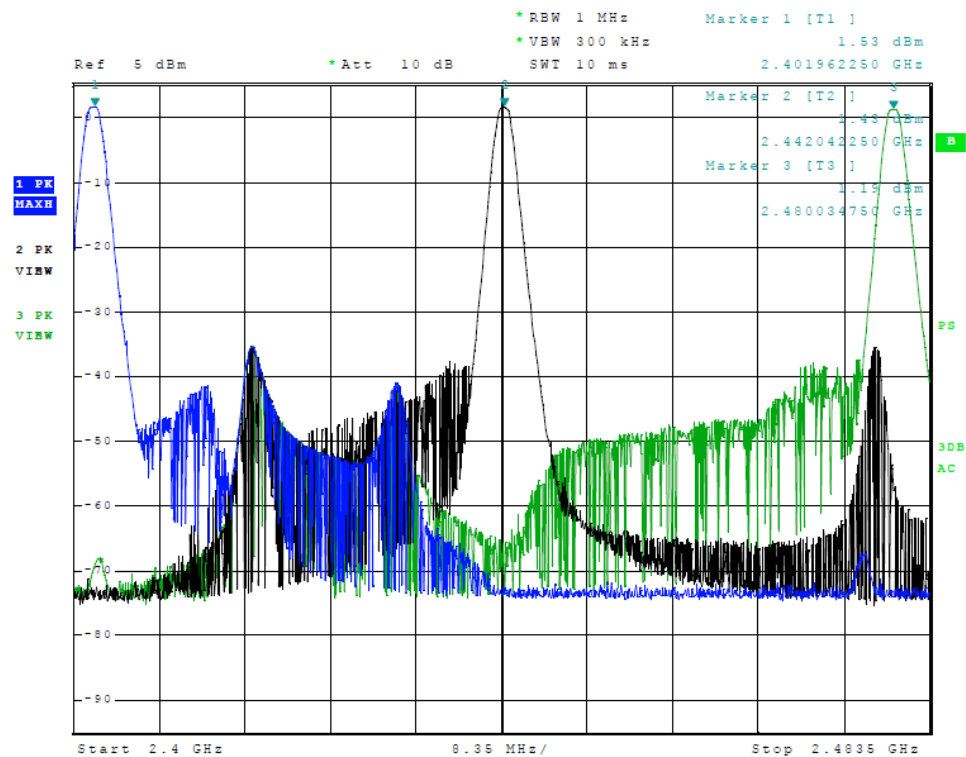
Figure 15 Plot of Transmitter Emissions (In 2402-2480 MHz Band, Mode 2)
