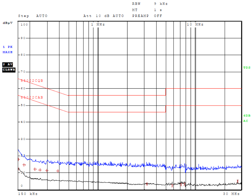
Figure 1 AC Line Conducted emissions of EUT line 1 (EUT AC Adapter SCB055600P)
