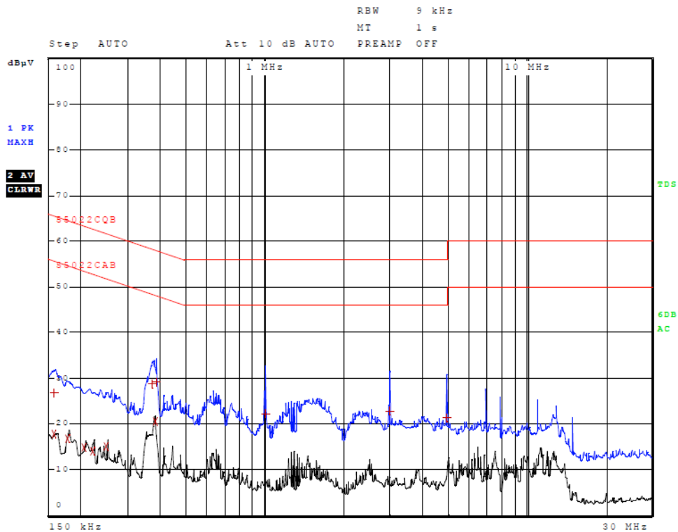
Figure 4 AC Line Conducted emissions of EUT line 2 (EUT AC Adapter 326-00072-00)
