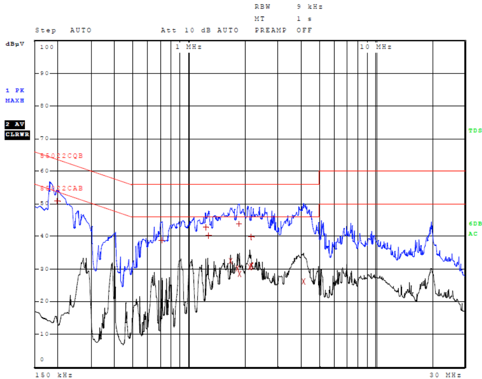
Figure 9 AC Line Conducted emissions of EUT line 1 (EUT-USB-CPU AC Adapter)
