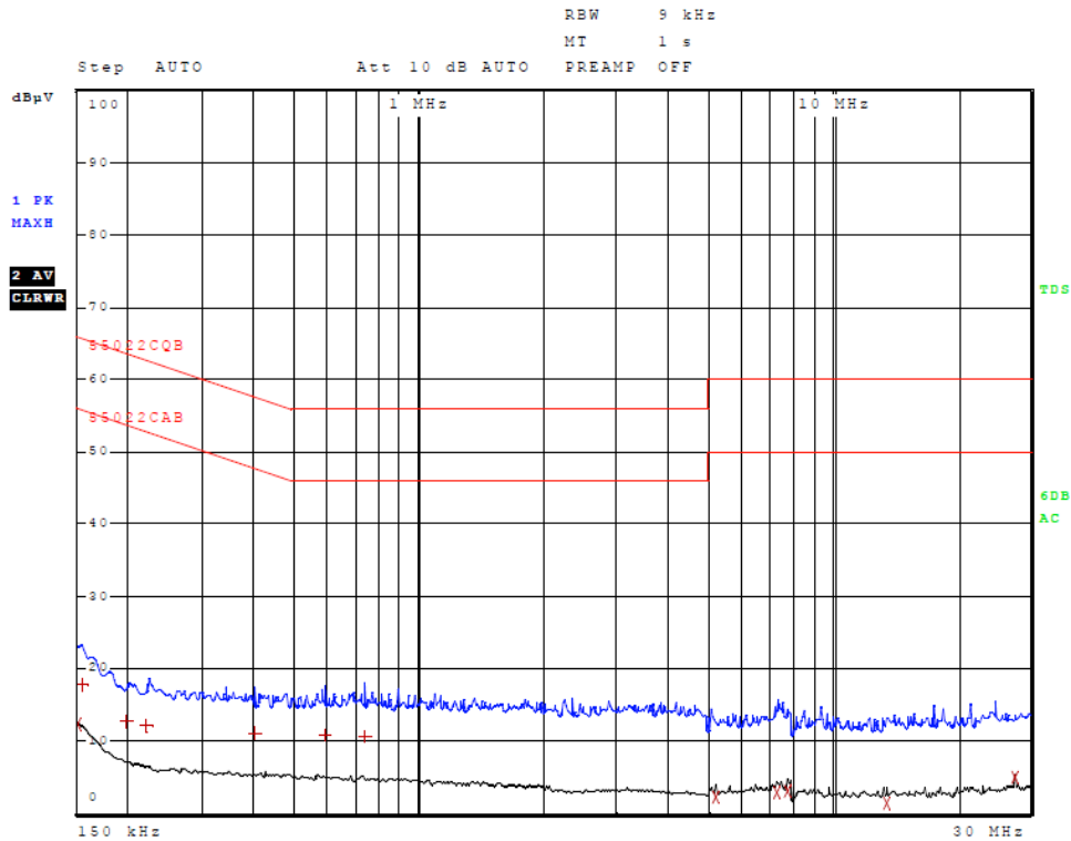
Figure 5 AC Line Conducted emissions of EUT line 1 (EUT AC Adapter 326-00086-01)
