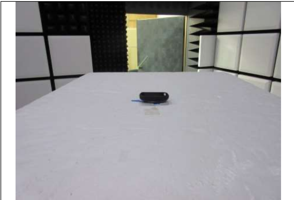
RF Radiated #4
