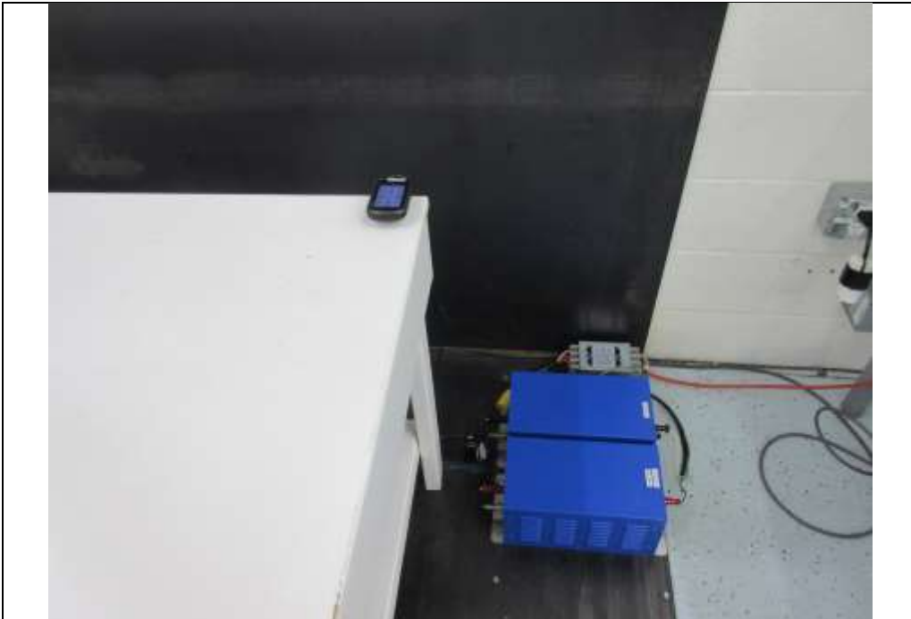
A/C Powerline Conduction #2
