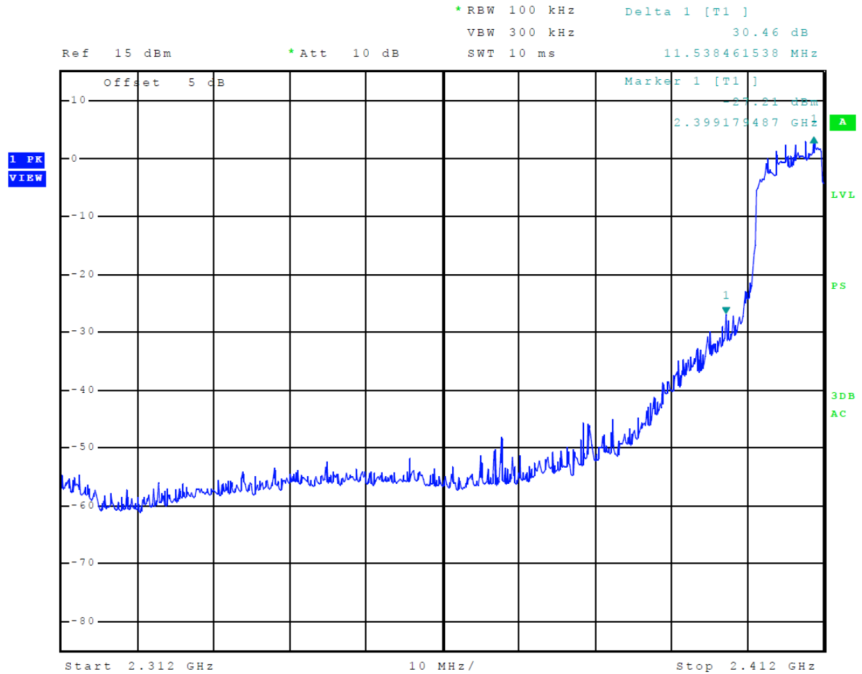
Figure 12 Plot of Transmitter Emissions Low Band Edge (Mode 7 802.11n)
