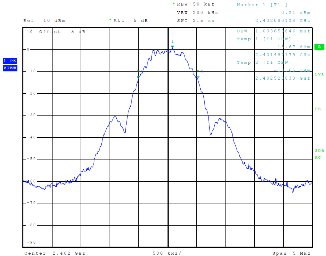
Figure 24 Plot of 99% Occupied Bandwidth (Mode 4 BLE (GMSK))
