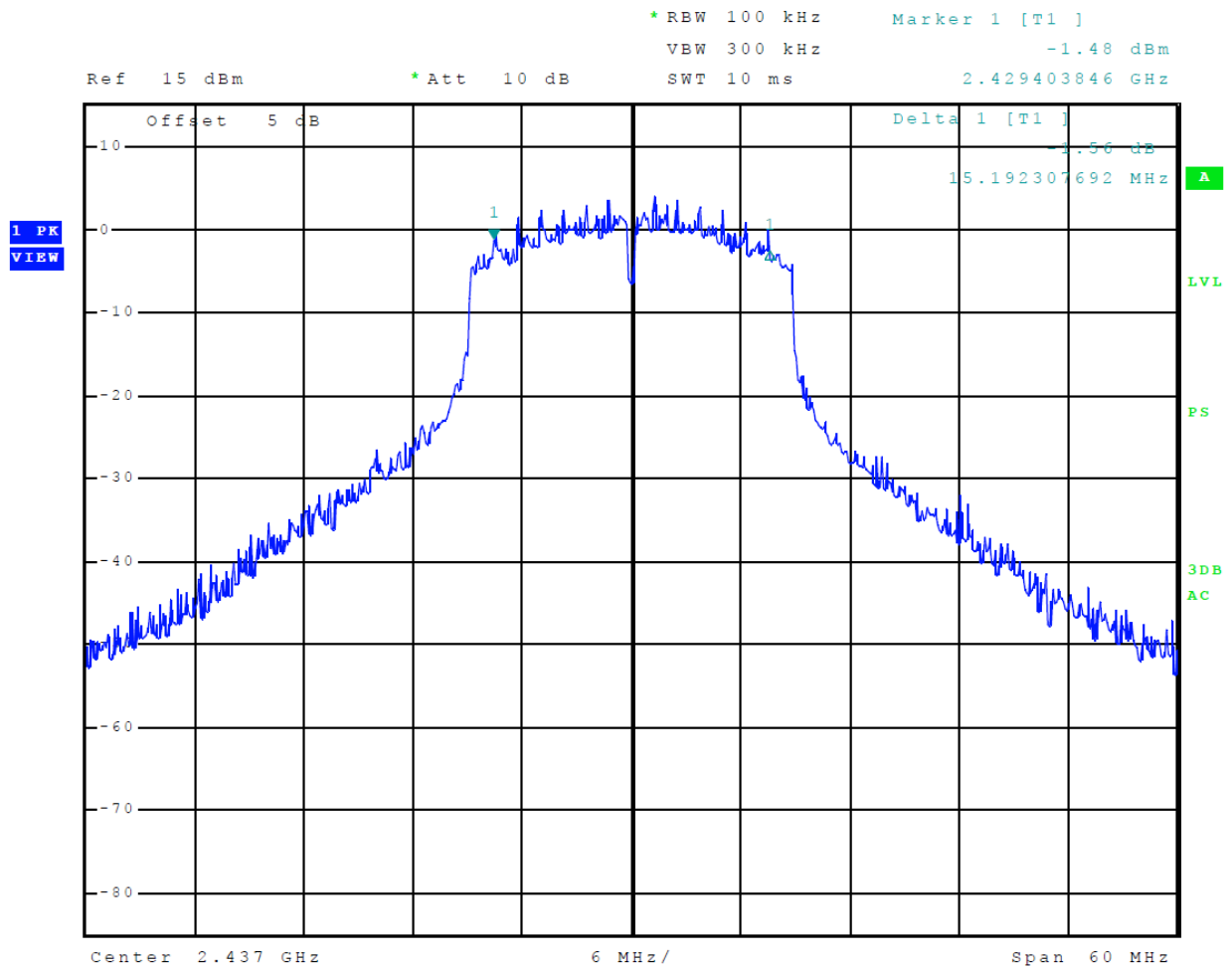
Figure 29 Plot of 6-dB Occupied Bandwidth (Mode 7 802.11n)
