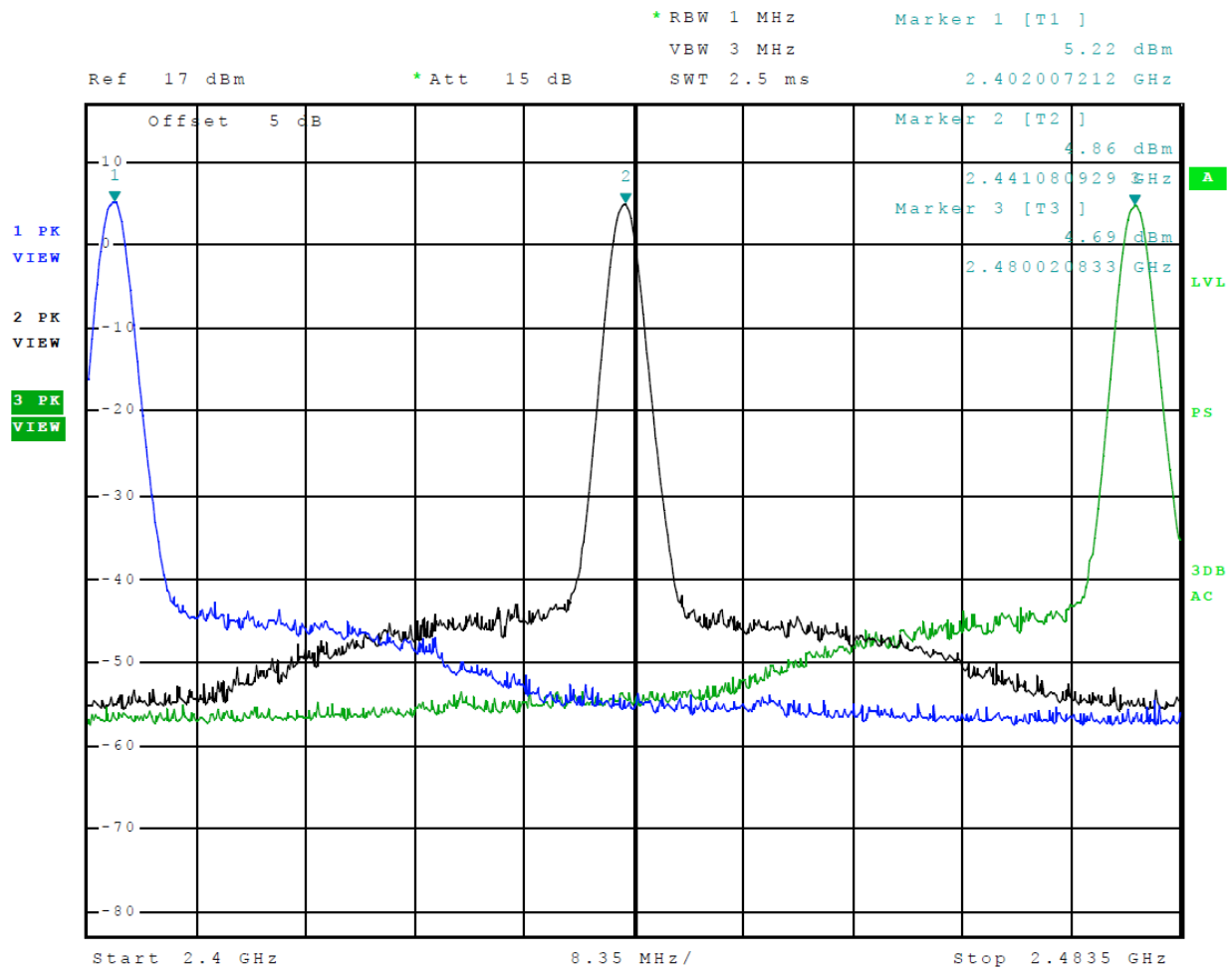
Figure 2 Plot of Transmitter Operation in 2402-2480 MHz (Mode 3 3EDR (8DPSK))
