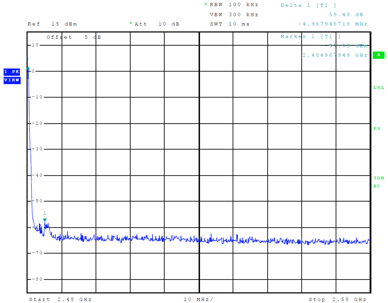
Figure 15 Plot of Transmitter Emissions High Band Edge (Mode 4 BLE (GMSK))
