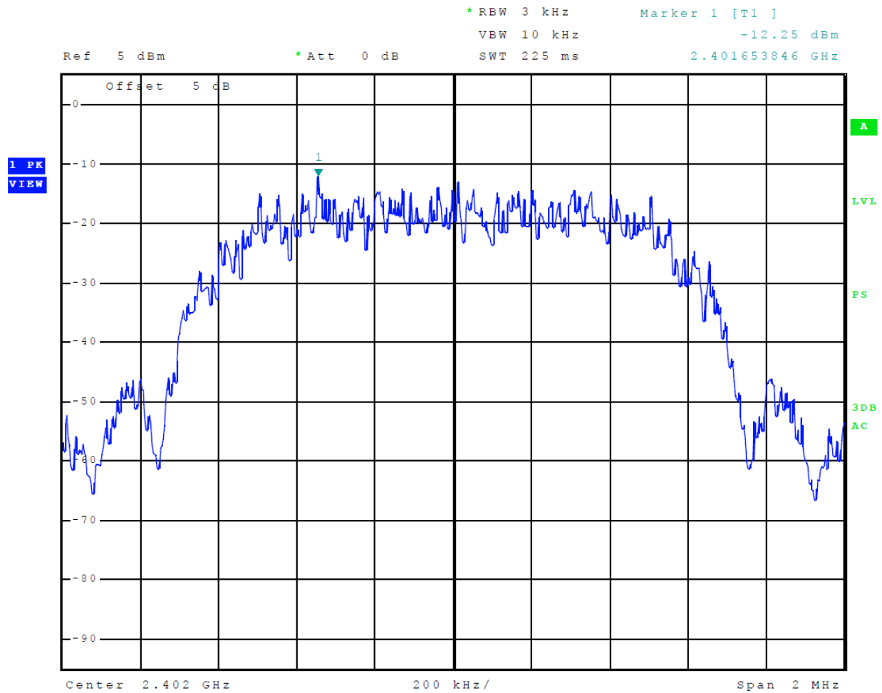
Figure 31 Plot of Transmitter Power Spectral Density (Mode 2 2EDR (PI/4 DQPSK))
