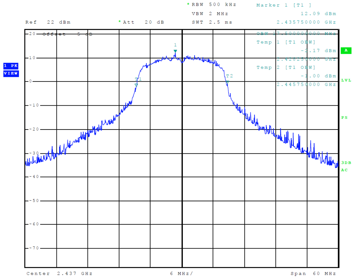
Figure 28 Plot of 99% Occupied Bandwidth (Mode 6 802.11g)
