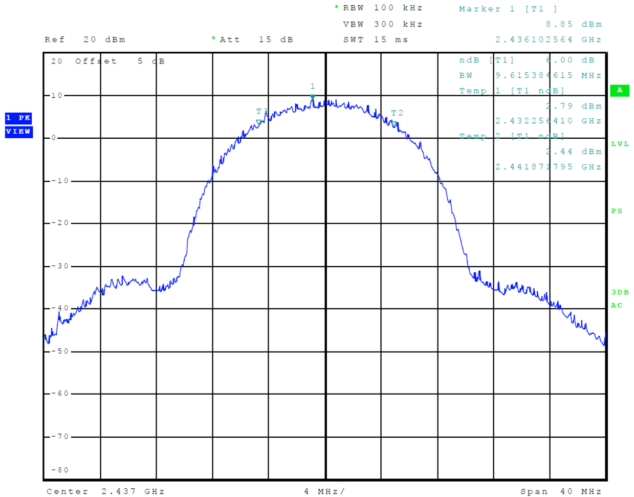
Figure 25 Plot of 6-dB Occupied Bandwidth (Mode 5 802.11b)
