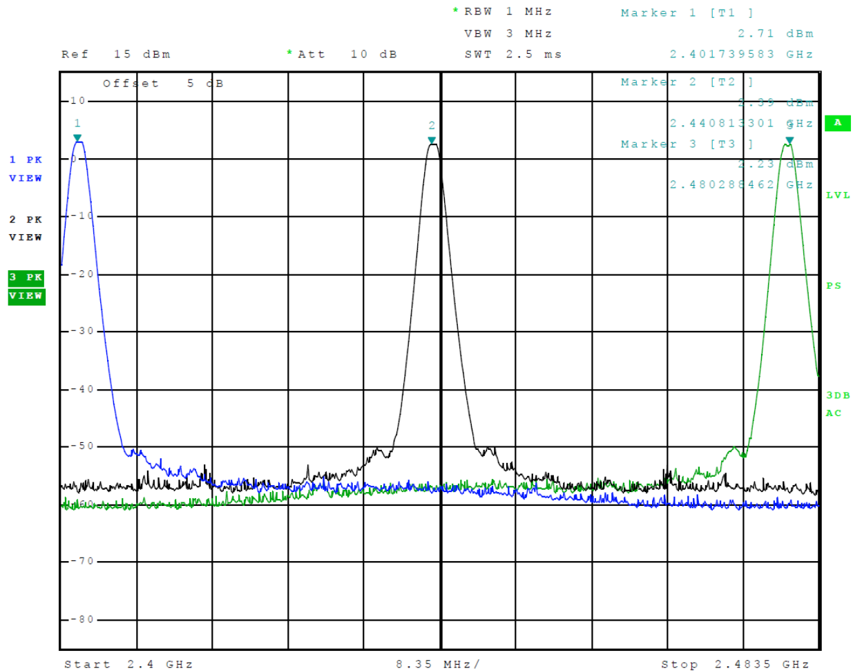
Figure 3 Plot of Transmitter Operation in 2402-2480 MHz (Mode 4 BLE (GMSK))
