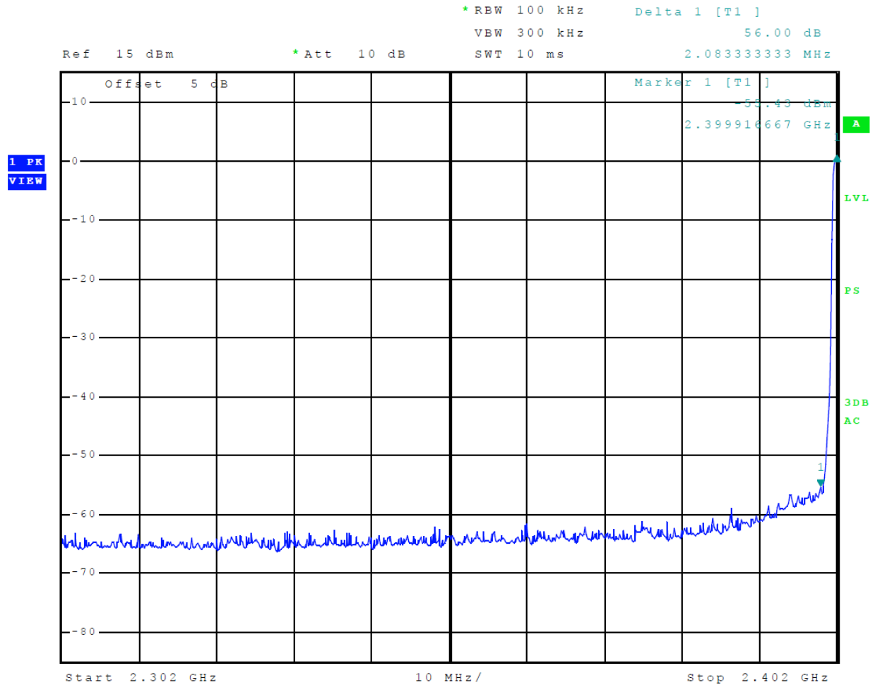
Figure 7 Plot of Transmitter Emissions Low Band Edge (Mode 2 2EDR (PI/4 DQPSK))
