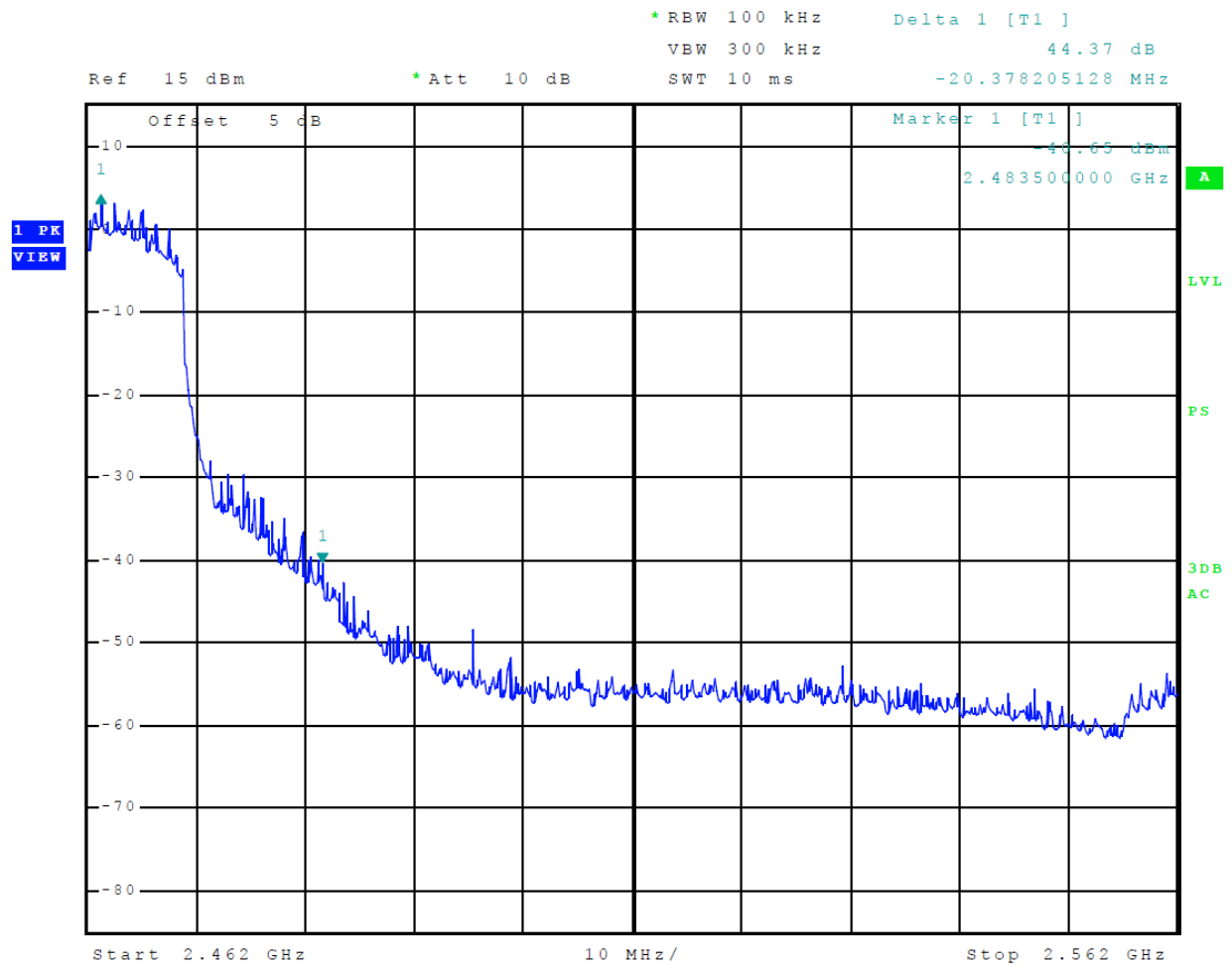
Figure 18 Plot of Transmitter Emissions High Band Edge (Mode 7 802.11n)
