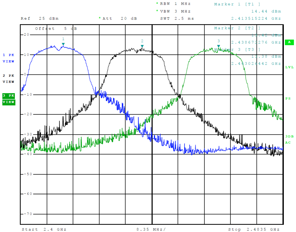
Figure 6 Plot of Transmitter Operation in 2412-2462 MHz (Mode 7 802.11n)
