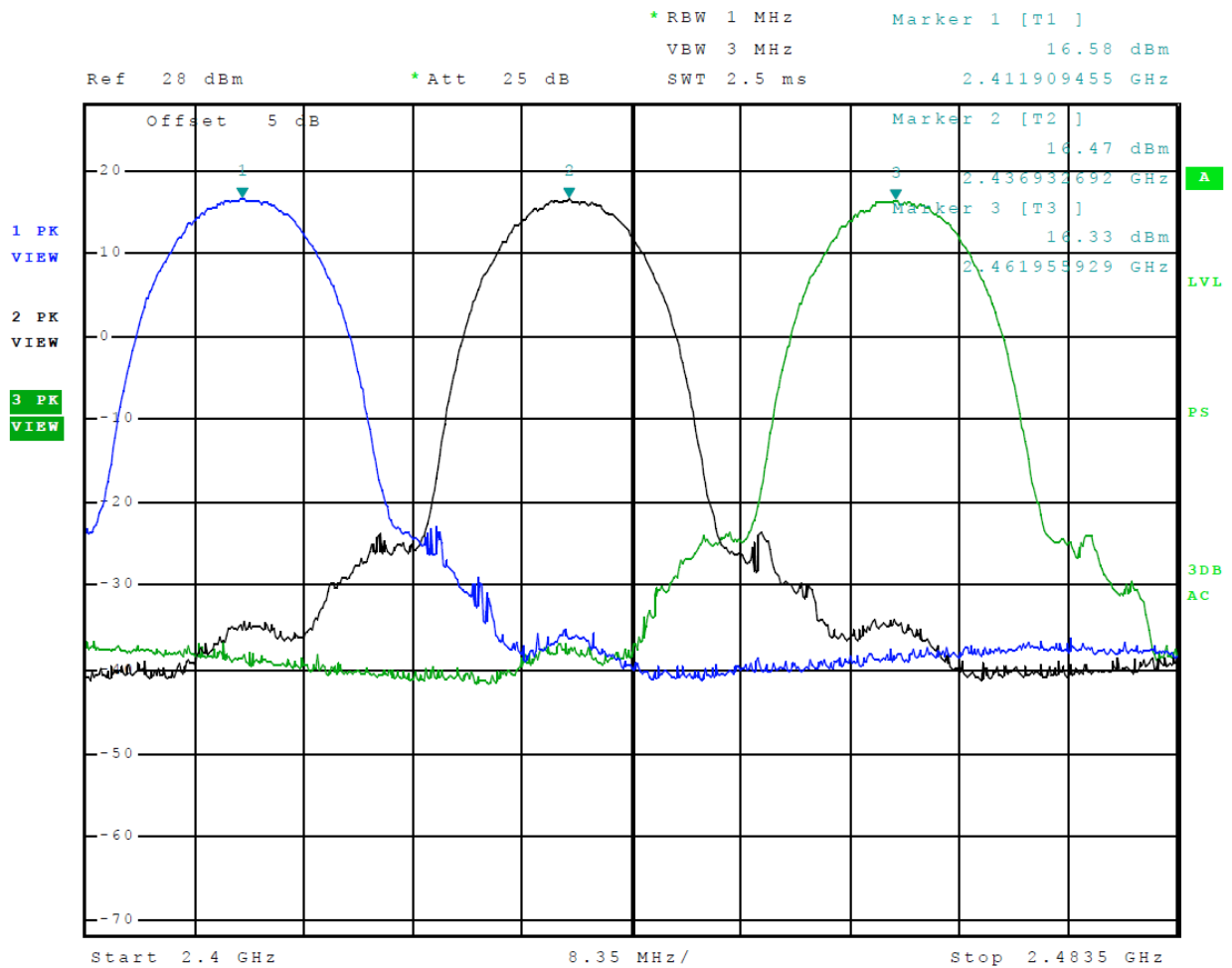
Figure 4 Plot of Transmitter Operation in 2412-2462 MHz (Mode 5 802.11b)
