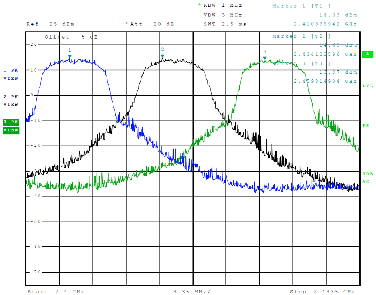
Figure 5 Plot of Transmitter Operation in 2412-2462 MHz (Mode 6 802.11g)
