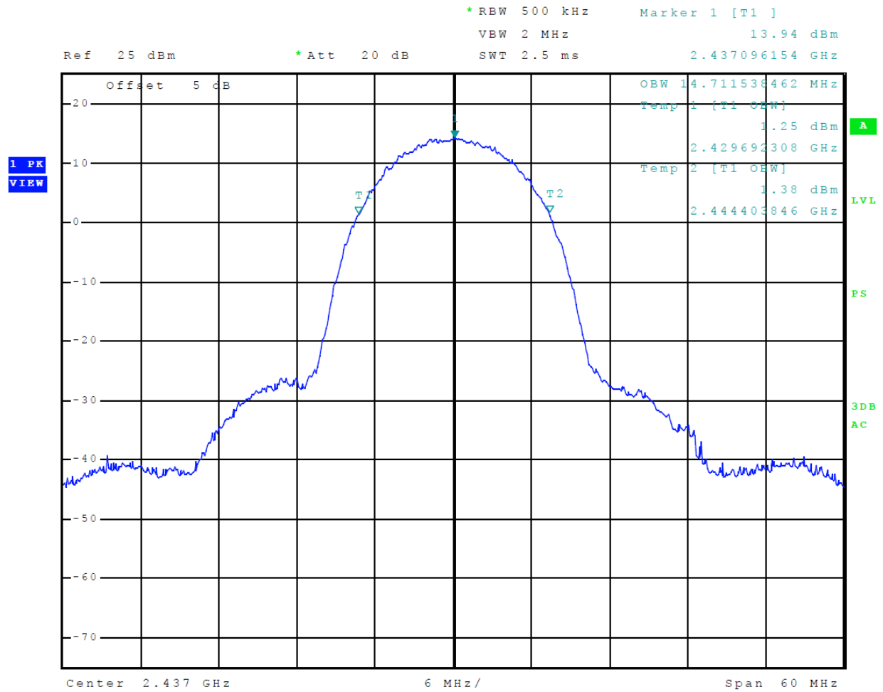
Figure 26 Plot of 99% Occupied Bandwidth (Mode 5 802.11b)
