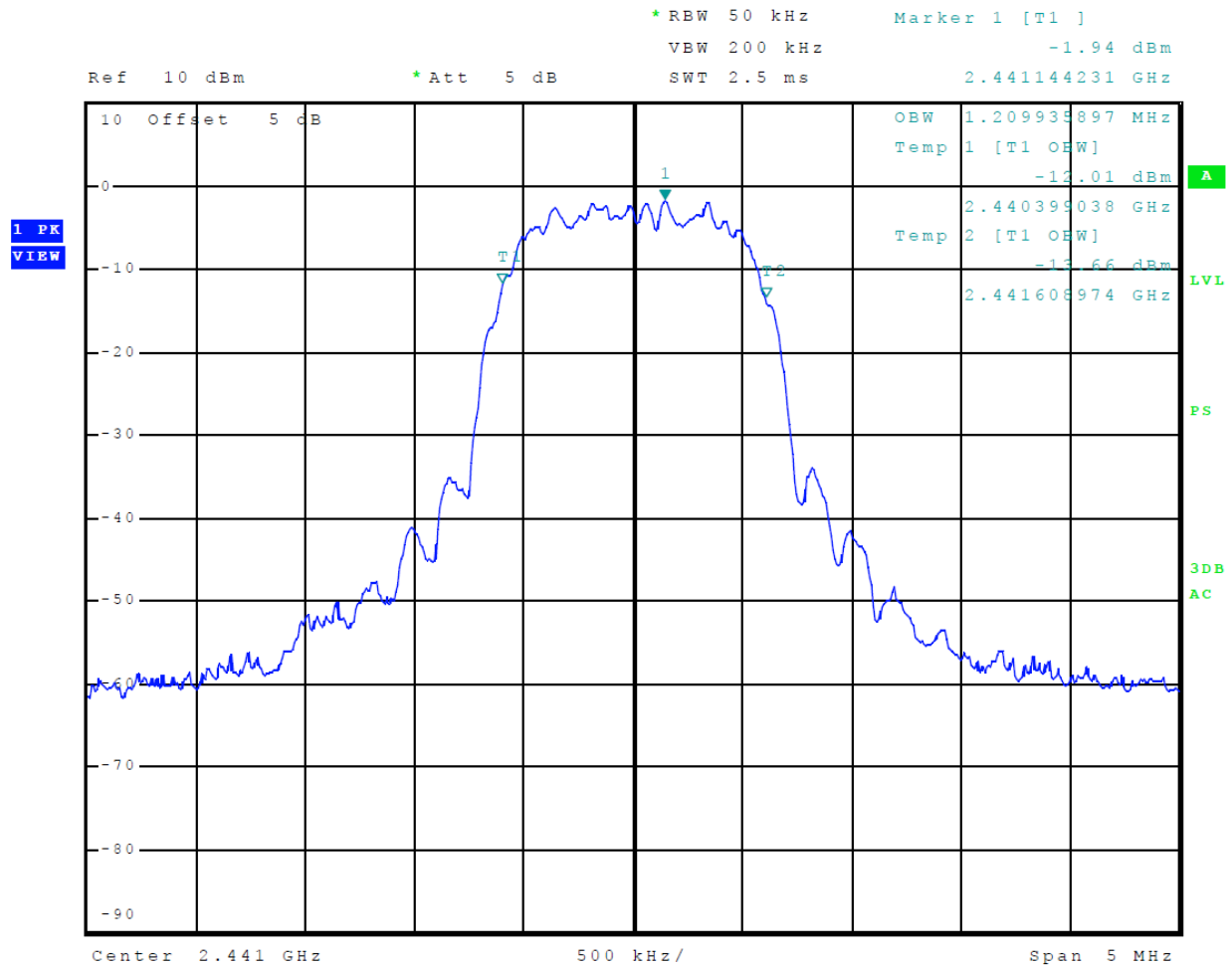
Figure 20 Plot of 99% Occupied Bandwidth (Mode 2 2EDR (PI/4 DQPSK))
