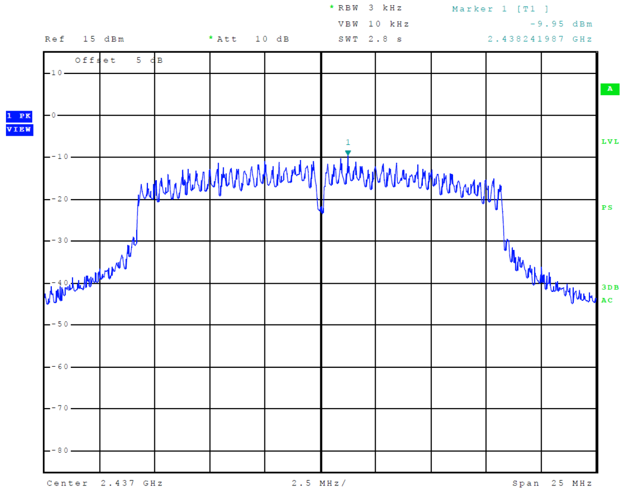
Figure 35 Plot of Transmitter Power Spectral Density (Mode 6 802.11g)
