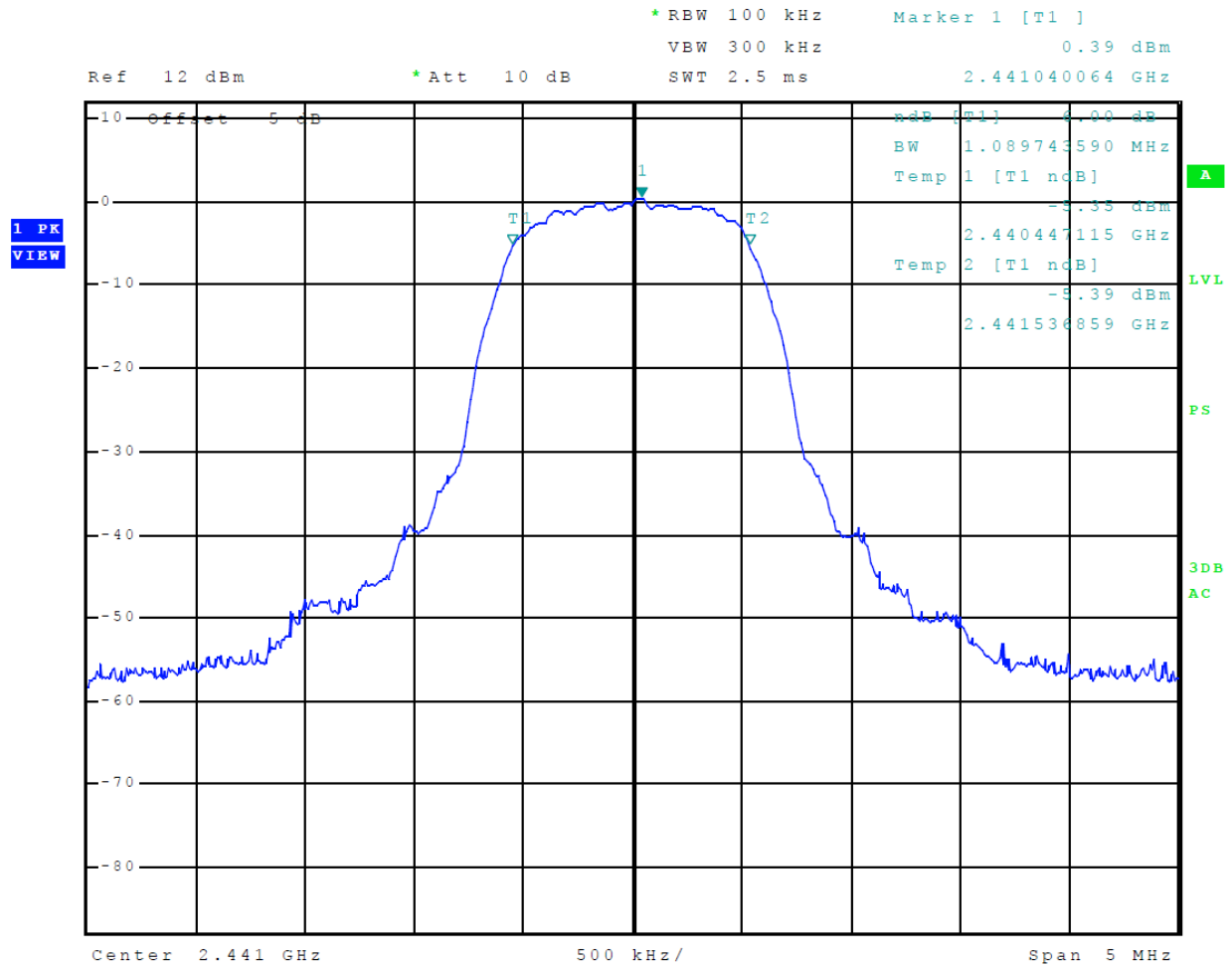
Figure 19 Plot of 6-dB Occupied Bandwidth (Mode 2 2EDR (PI/4 DQPSK))
