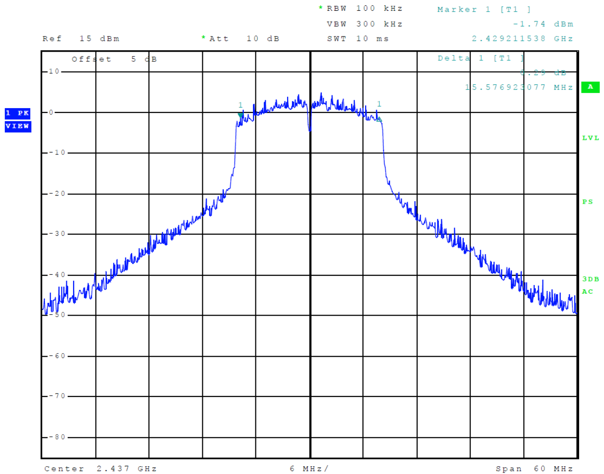
Figure 27 Plot of 6-dB Occupied Bandwidth (Mode 6 802.11g)
