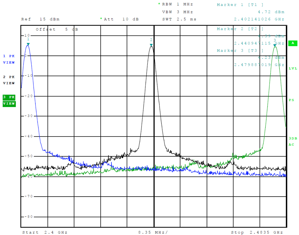
Figure 1 Plot of Transmitter Operation in 2402-2480 MHz (Mode 2 2EDR (PI/4 DQPSK))
