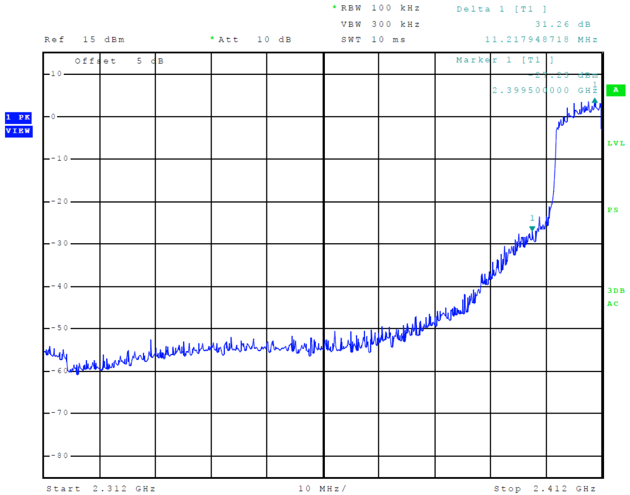
Figure 11 Plot of Transmitter Emissions Low Band Edge (Mode 6 802.11g)
