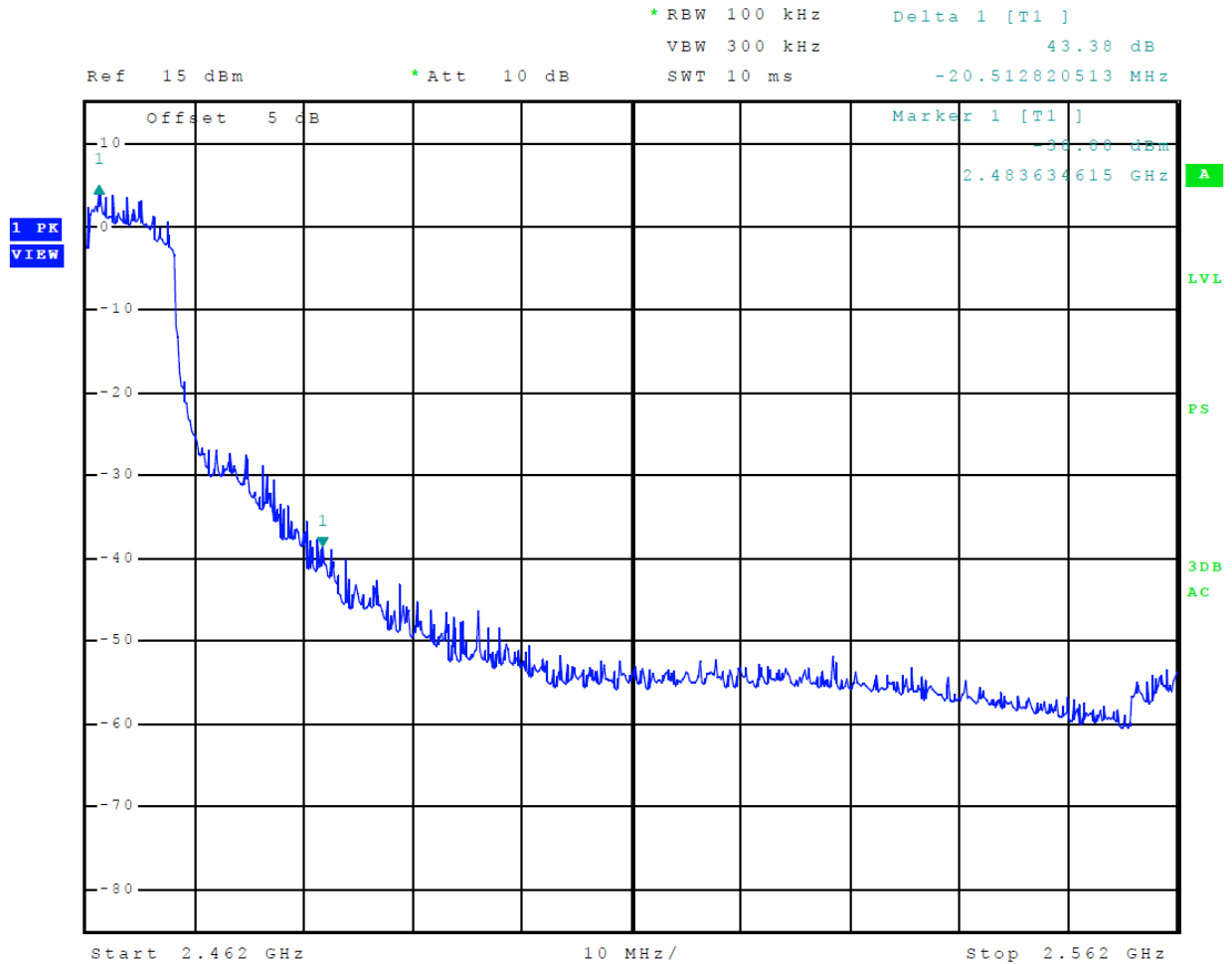
Figure 17 Plot of Transmitter Emissions High Band Edge (Mode 6 802.11g)
