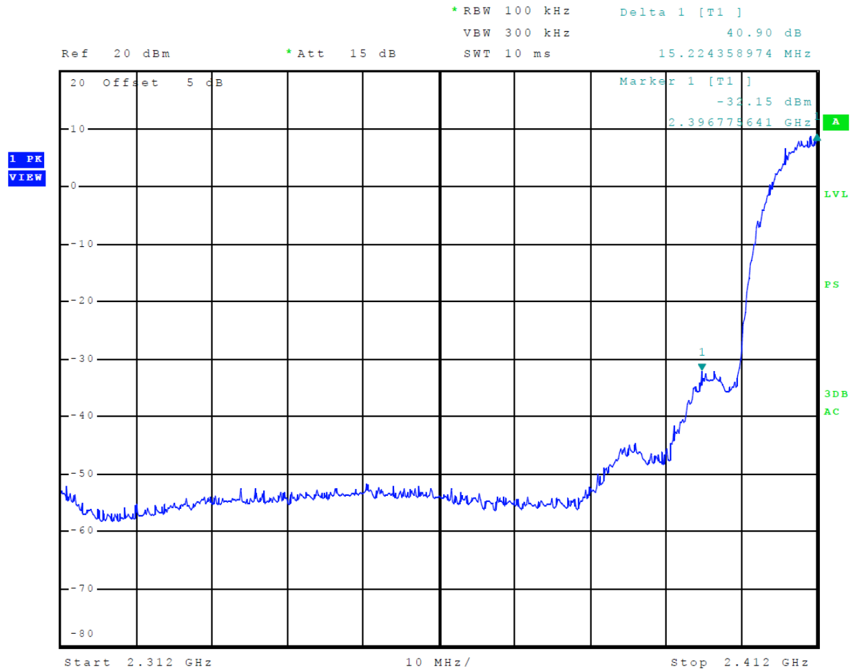
Figure 10 Plot of Transmitter Emissions Low Band Edge (Mode 5 802.11b)
