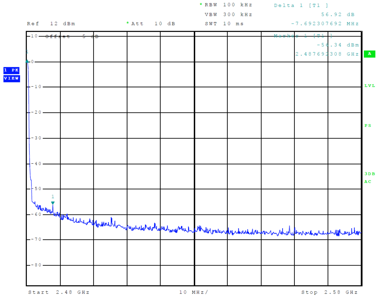
Figure 14 Plot of Transmitter Emissions High Band Edge (Mode 3 3EDR (8DPSK))
