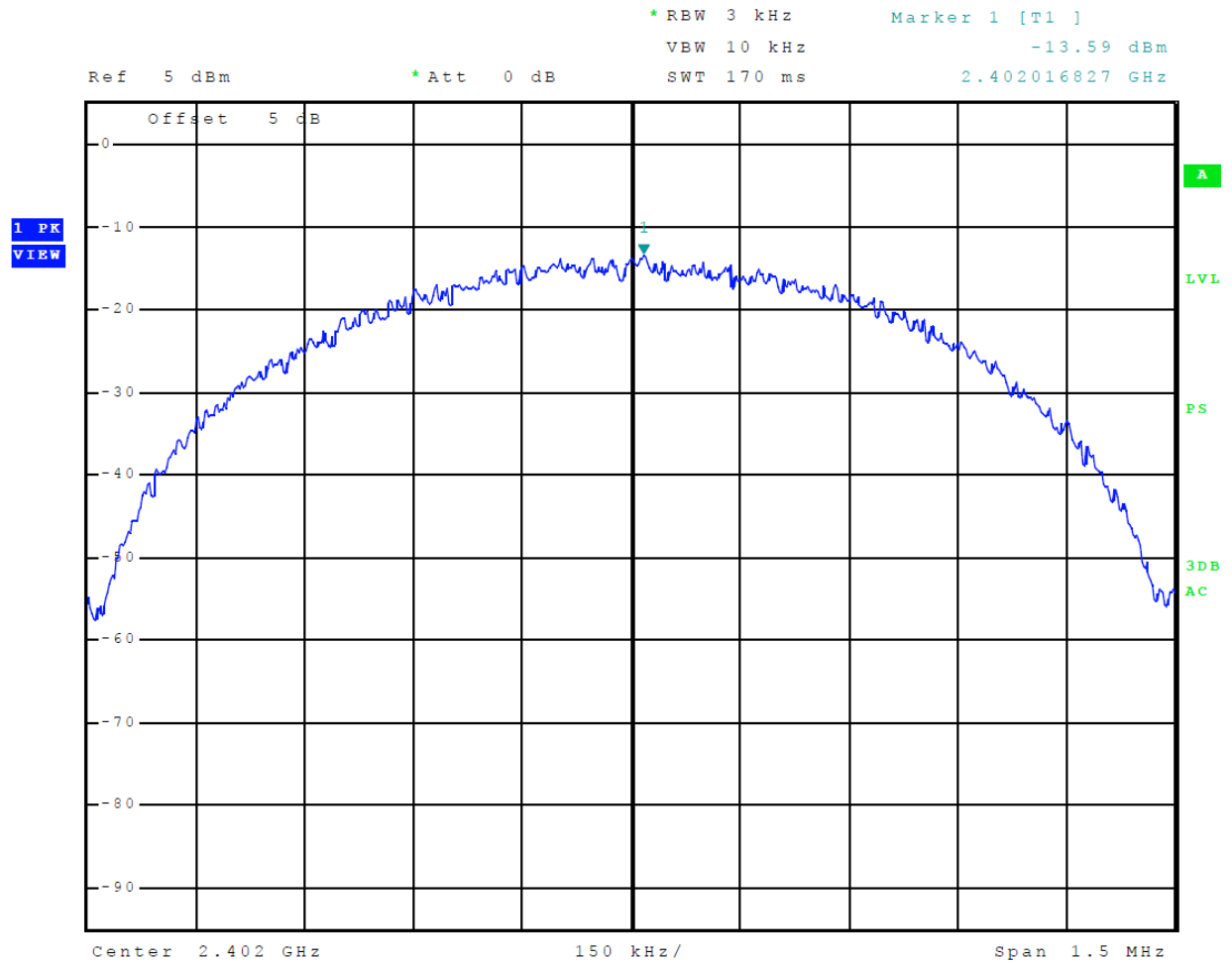
Figure 33 Plot of Transmitter Power Spectral Density (Mode 4 BLE (GMSK))
