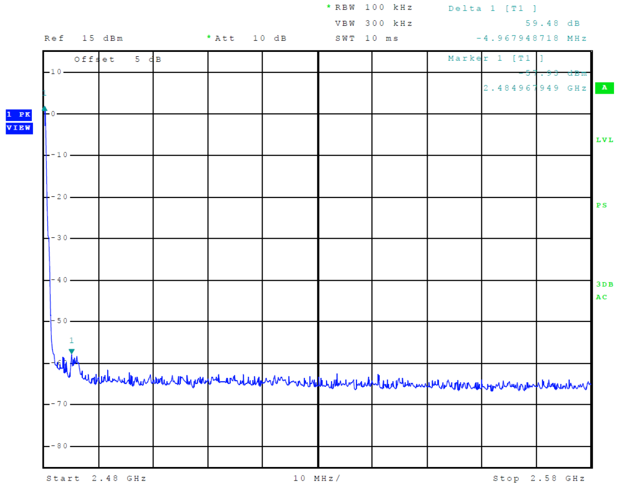
Figure 16 Plot of Transmitter Emissions High Band Edge (Mode 5 802.11b)
