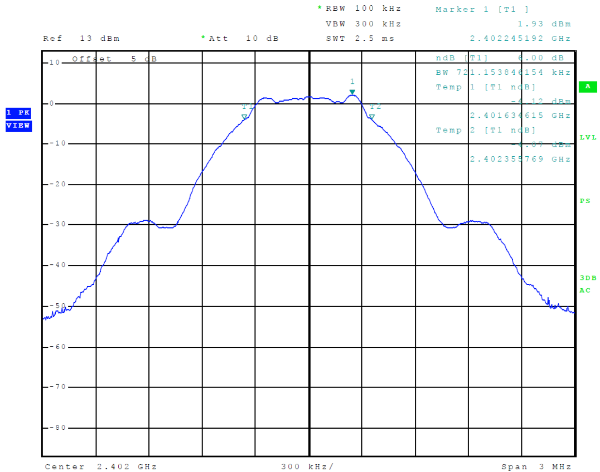
Figure 23 Plot of 6-dB Occupied Bandwidth (Mode 4 BLE (GMSK))
