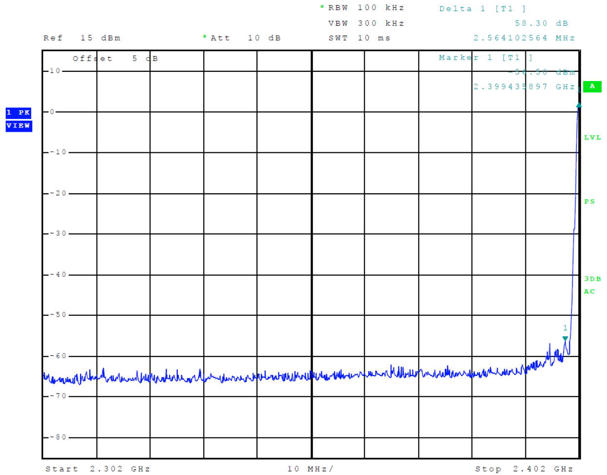
Figure 9 Plot of Transmitter Emissions Low Band Edge (Mode 4 BLE (GMSK))
