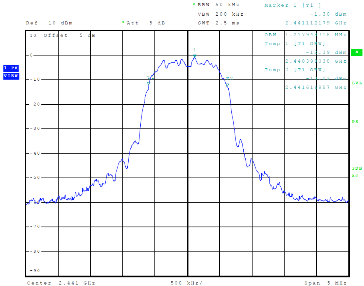
Figure 22 Plot of 99% Occupied Bandwidth (Mode 3 3EDR (8DPSK))
