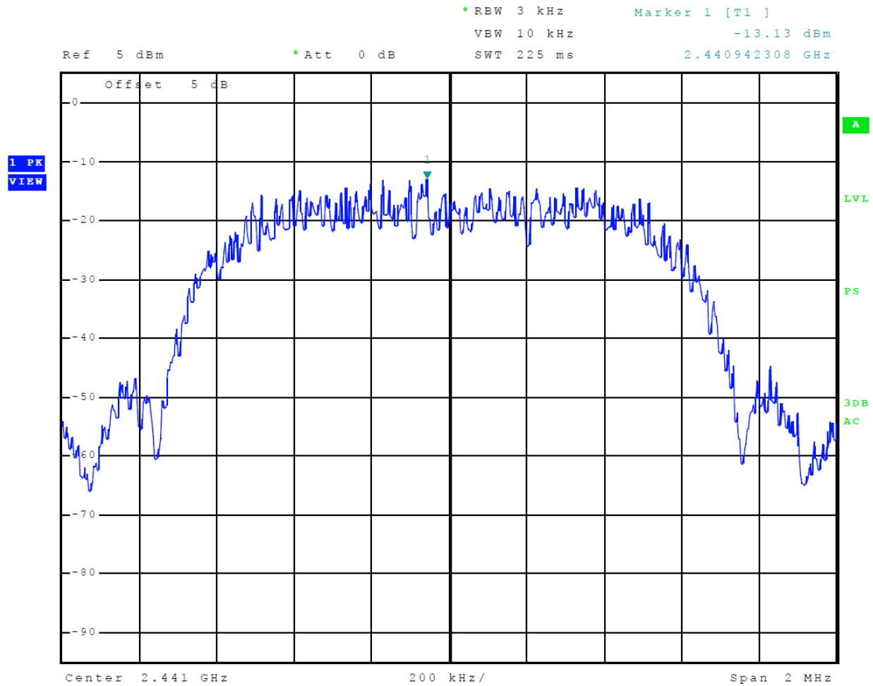
Figure 32 Plot of Transmitter Power Spectral Density (Mode 3 3EDR (8DPSK))
