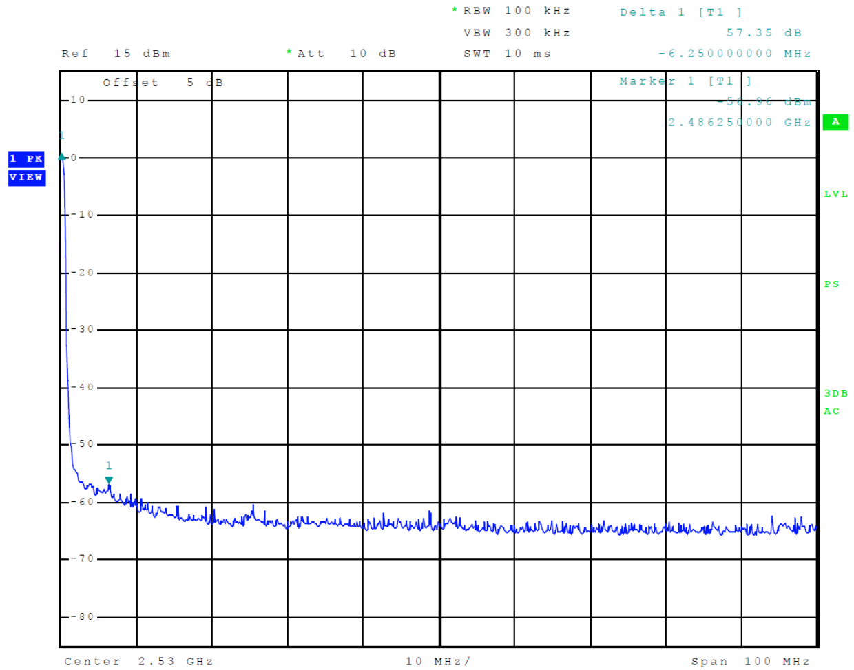
Figure 13 Plot of Transmitter Emissions High Band Edge (Mode 2 2EDR (PI/4 DQPSK))
