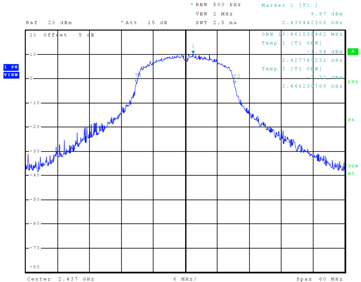
Figure 30 Plot of 99% Occupied Bandwidth (Mode 7 802.11n)
