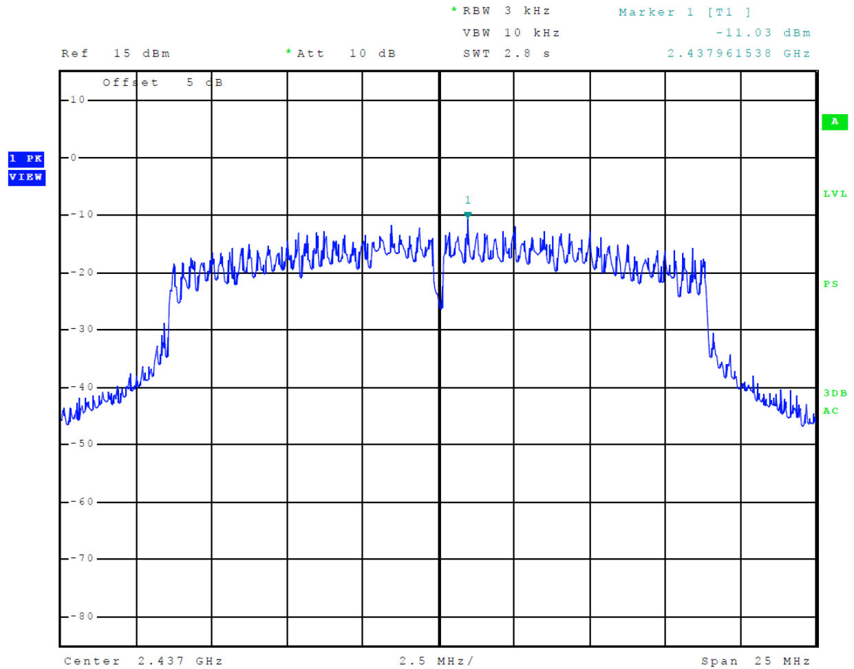
Figure 36 Plot of Transmitter Power Spectral Density (Mode 7 802.11n)
