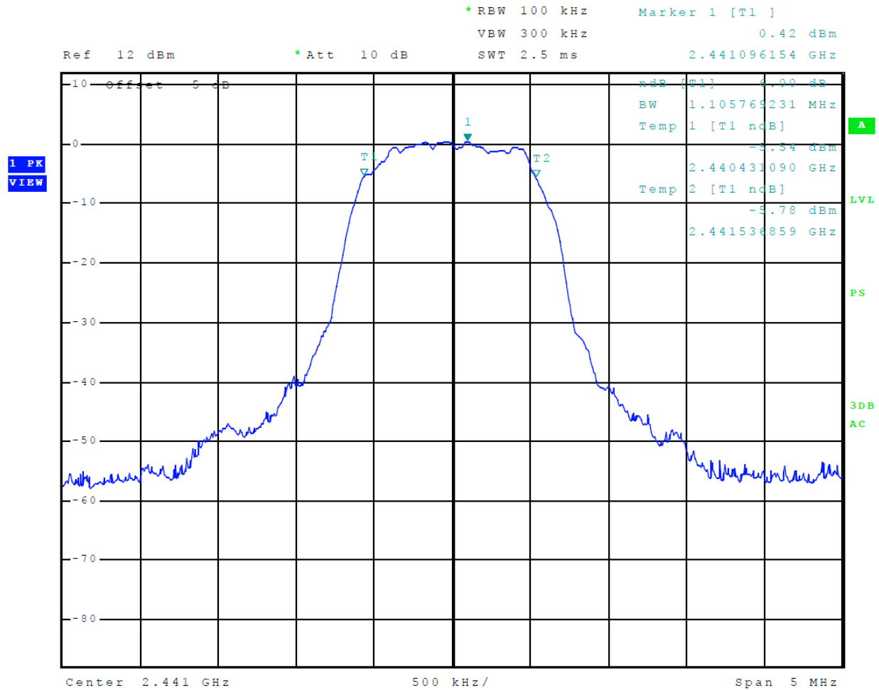
Figure 21 Plot of 6-dB Occupied Bandwidth (Mode 3 3EDR (8DPSK))
