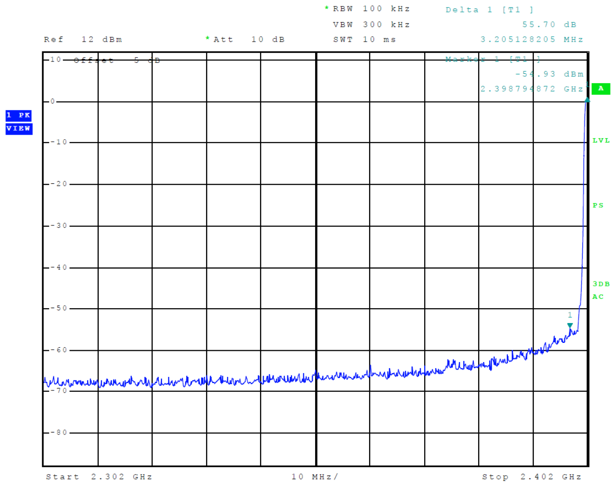
Figure 8 Plot of Transmitter Emissions Low Band Edge (Mode 3 3EDR (8DPSK))
