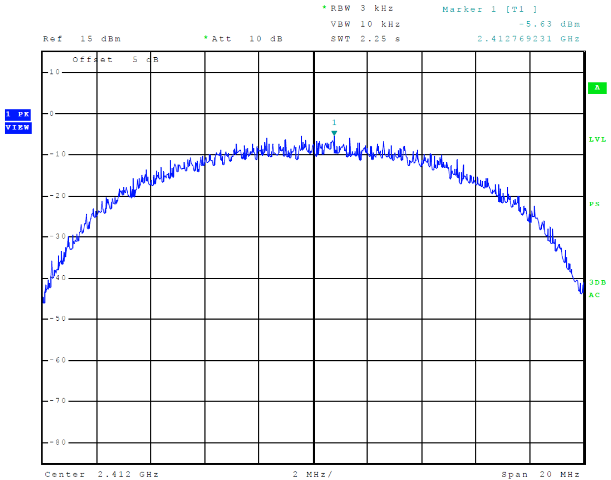
Figure 34 Plot of Transmitter Power Spectral Density (Mode 5 802.11b)
