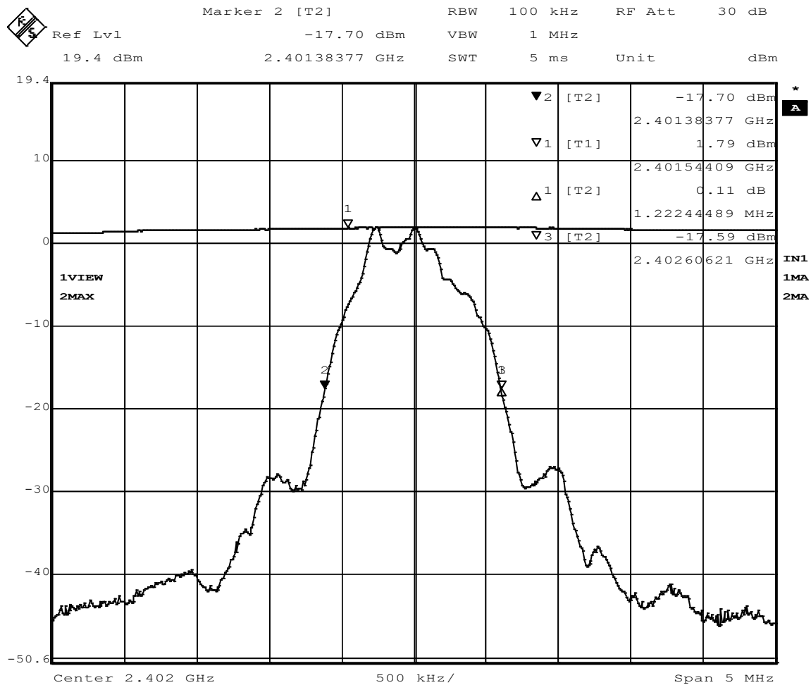
Figure 7 – Output Power
