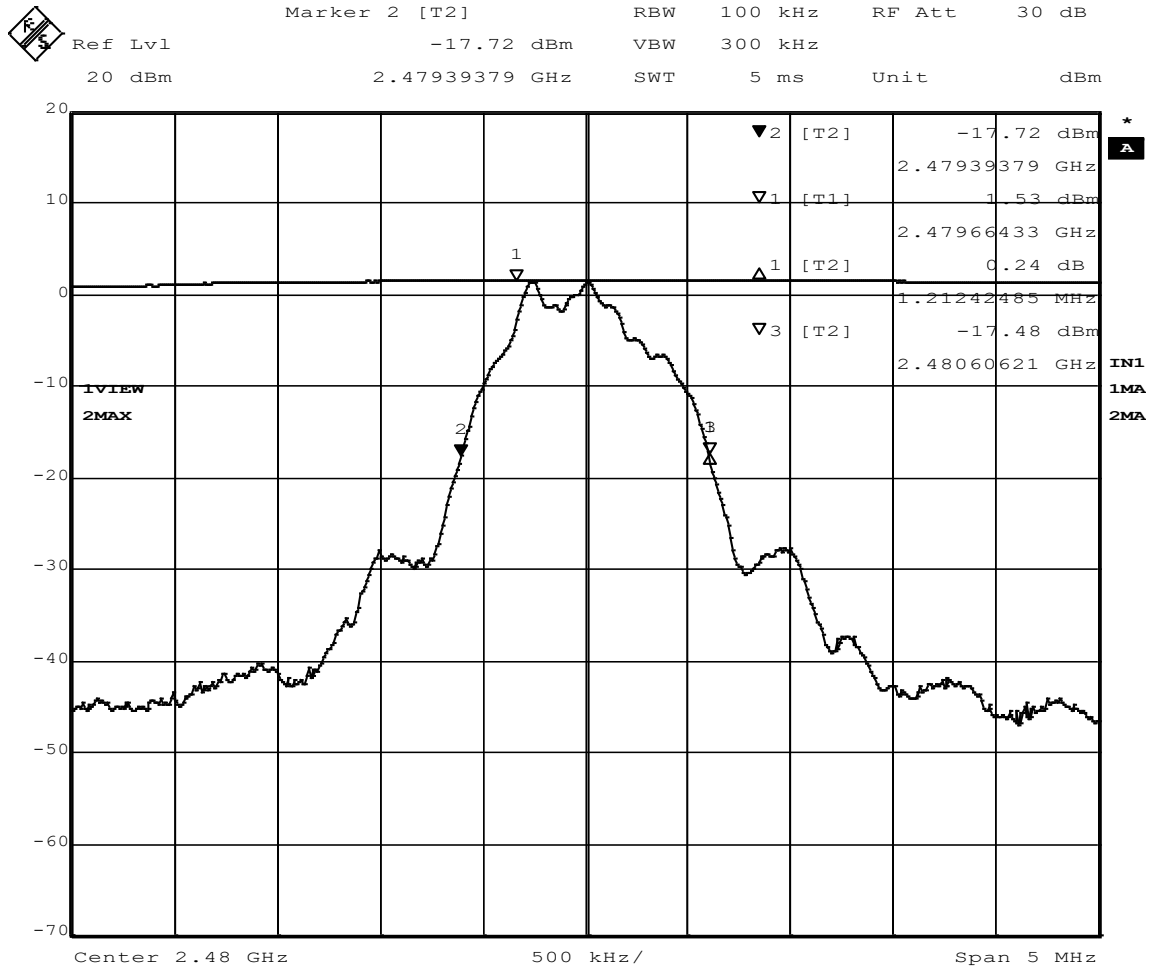
Figure 9 – Output Power
