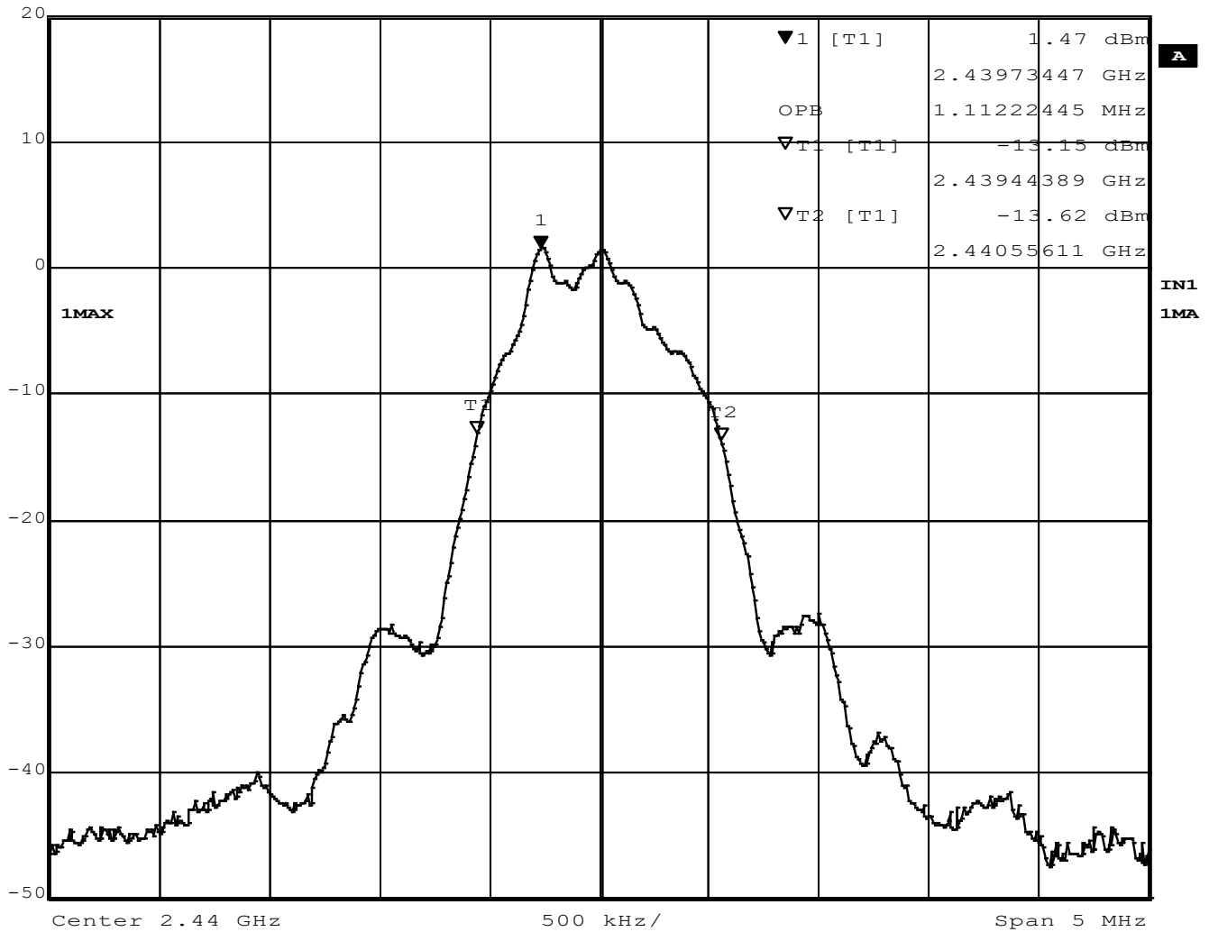
Figure 12 - Occupied Bandwidth, Mid Channel
