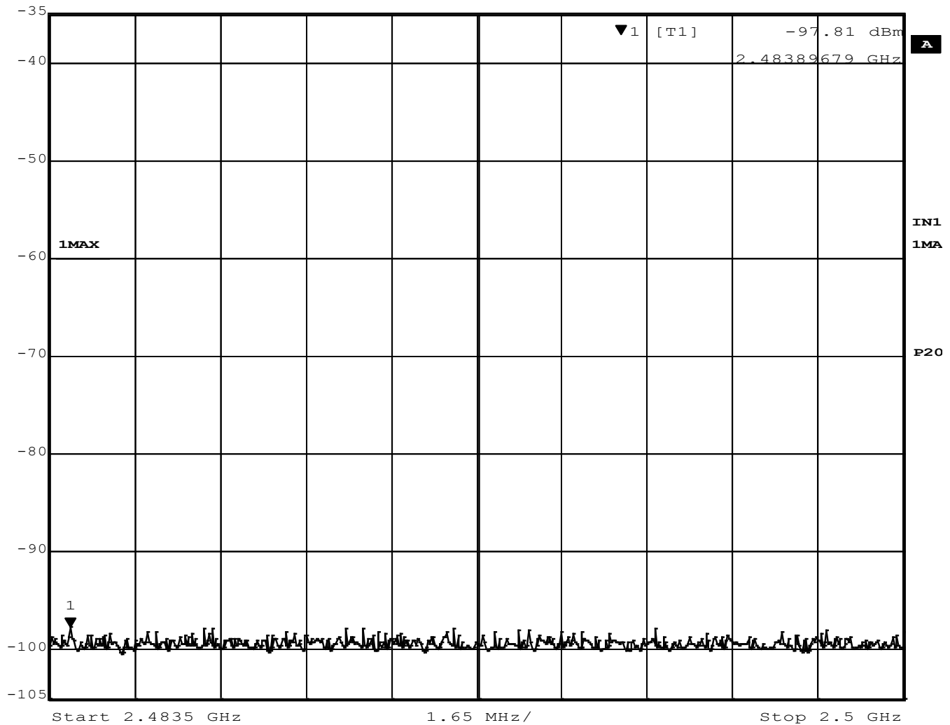
Figure 19 - Band-edge Measurement, High Channel, Restricted Frequency, Continuous Transmit
