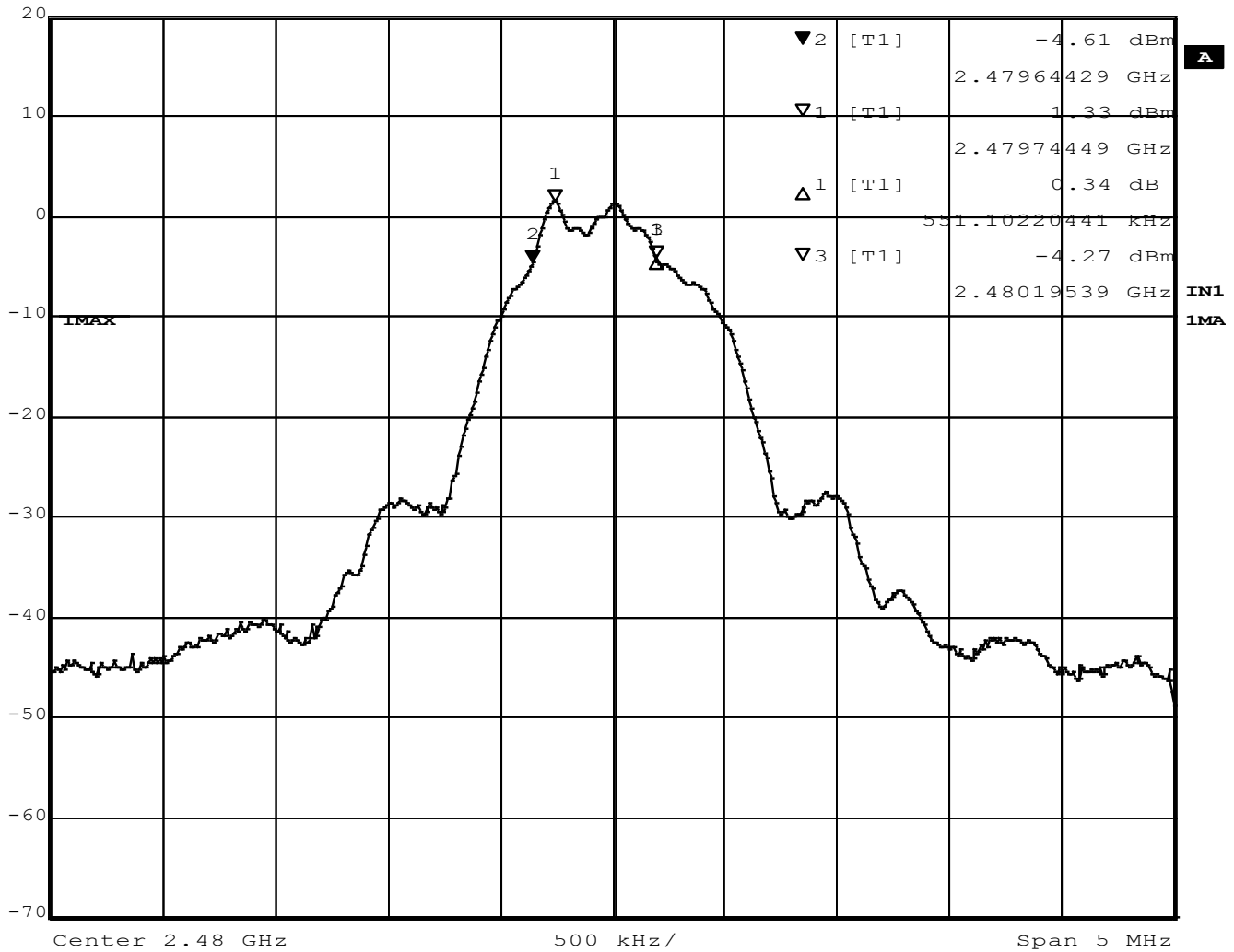
Figure 16 - 6dB Bandwidth, High Channel
