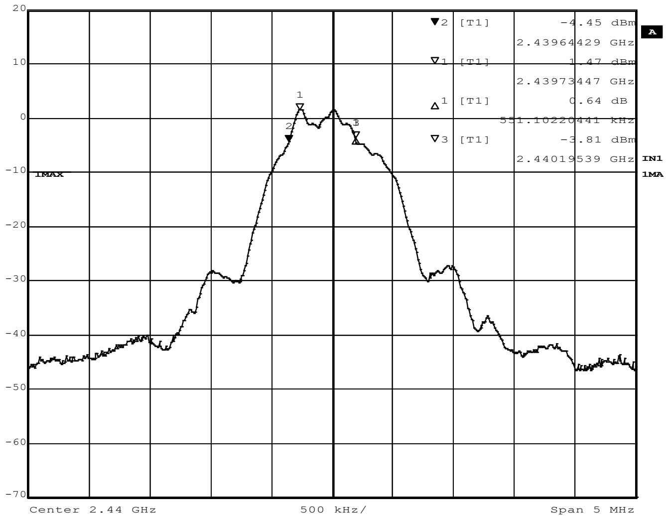
Figure 15 - 6dB Bandwidth, Mid Channel
