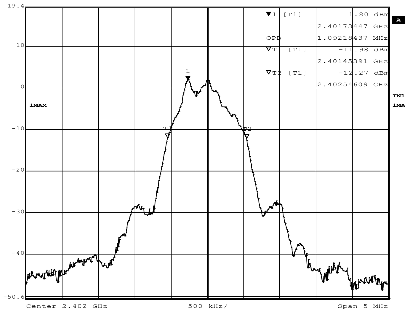
Figure 11 – Occupied Bandwidth, Low Channel
