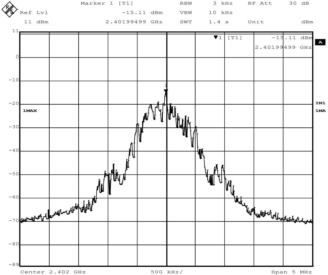
Figure 21 - Power Spectral Density, Low Channel
