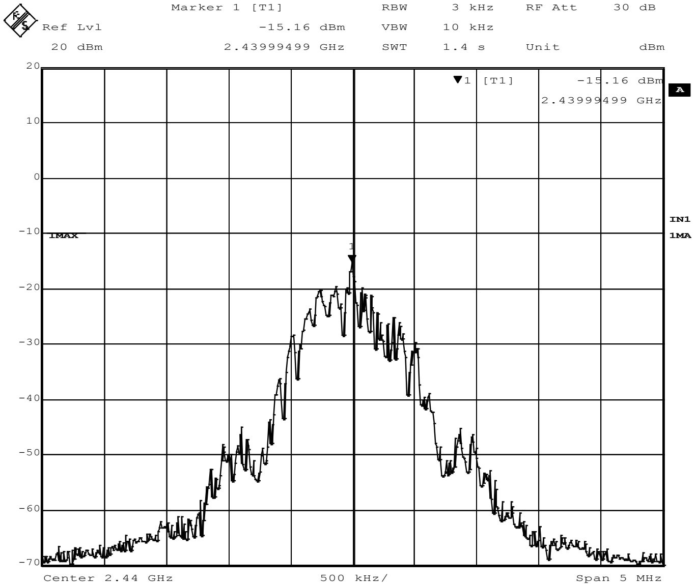
Figure 22 - Power Spectral Density, Mid Channel
