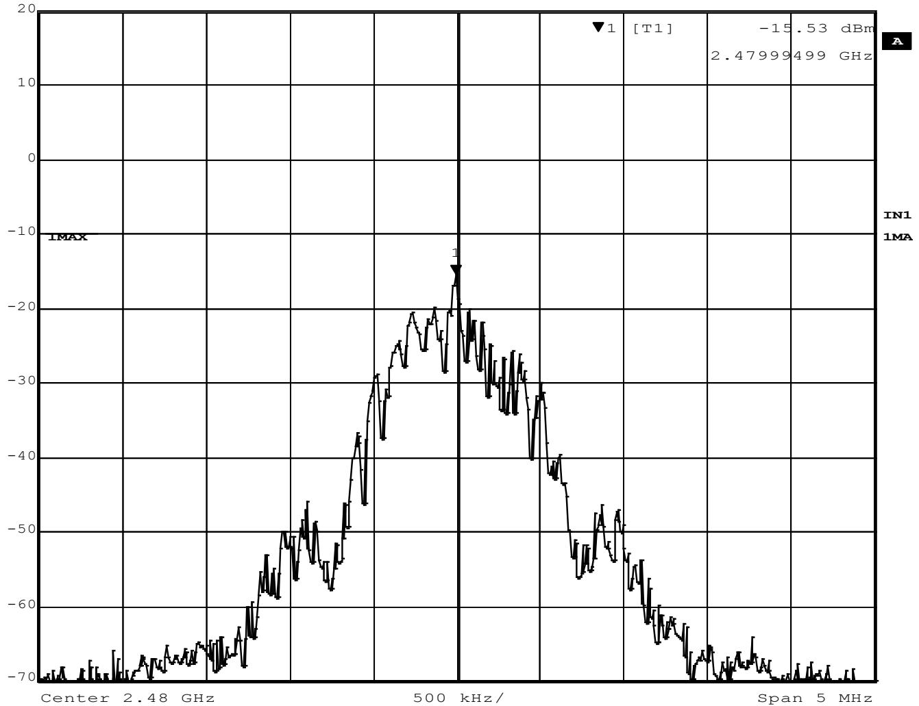
Figure 23 - Power Spectral Density, High Channel
