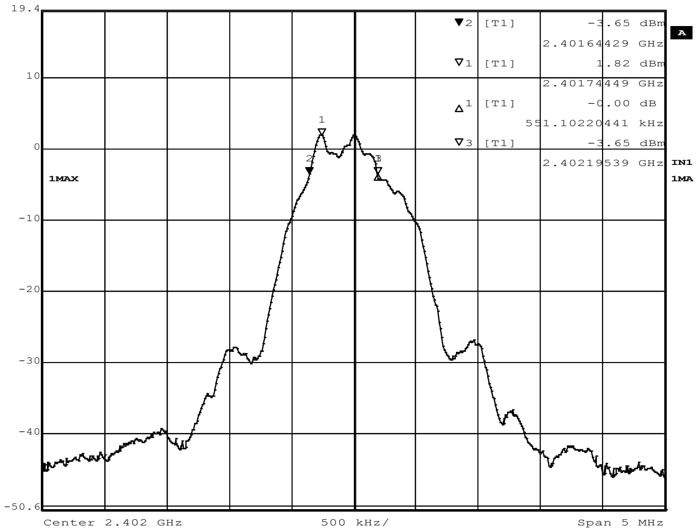
Figure 14 – 6dB Bandwidth, Low Channel
