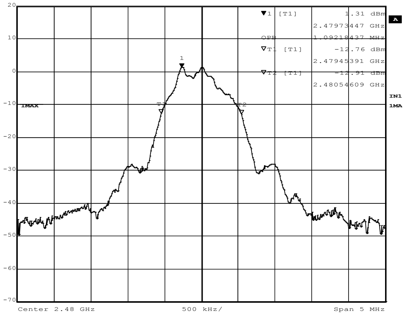
Figure 13 - Occupied Bandwidth, High Channel
