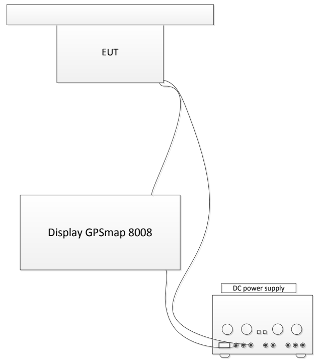
Figure 3.6-1: Setup diagram
