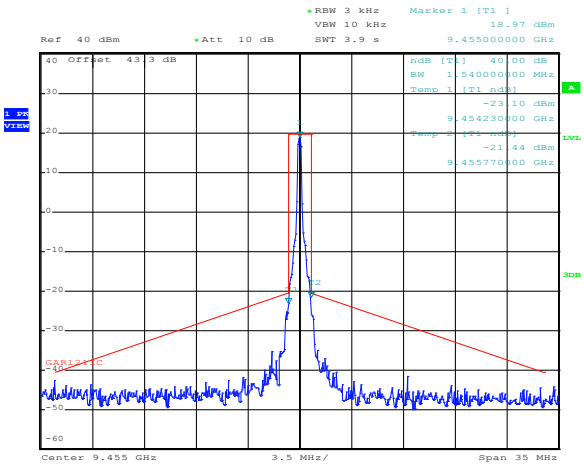
Figure 8.3-1: ISD Mask 1/16 nmi
