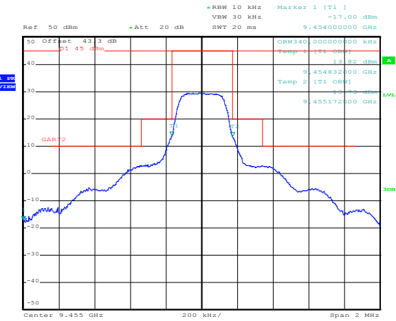
Figure 8.3-2: FCC mask 1/16 nmi
