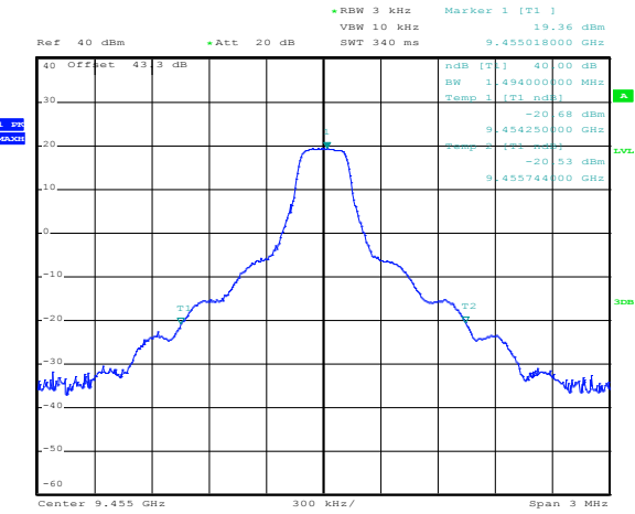
Figure 8.2-2: 40 dB bandwidth, 1/16 nmi
