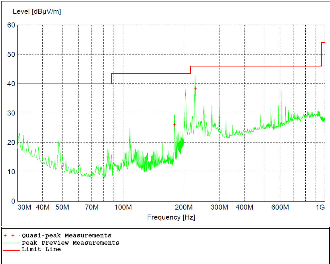
Figure 11 - Radiated Emissions Plot, High Channel
