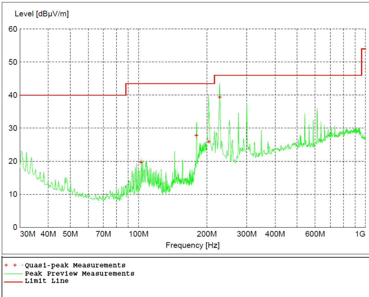
Figure 2 - Radiated Emissions Plot, Receive
