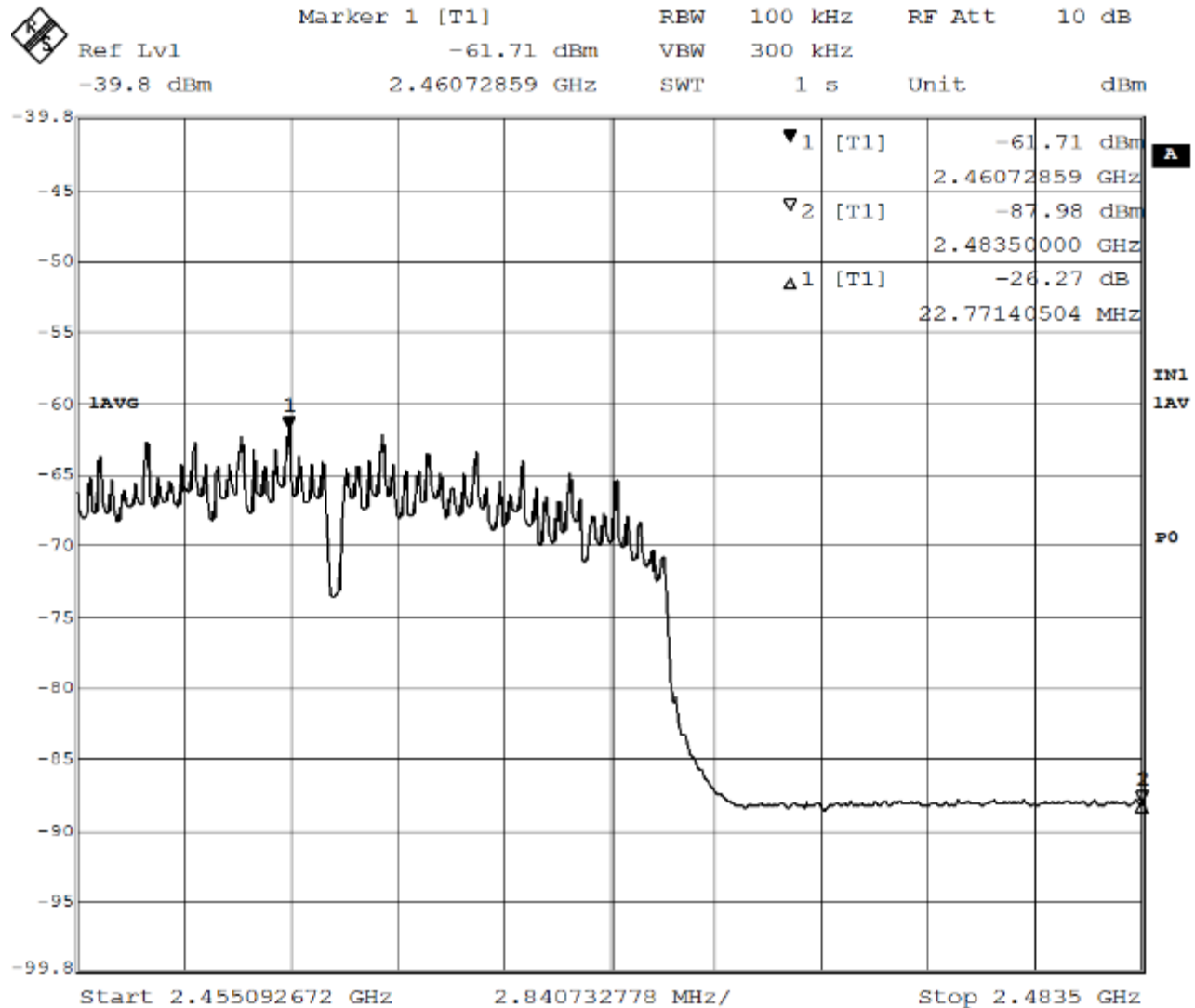
Figure 54 - Band-edge Measurement, High Channel, Fundamental, Average
