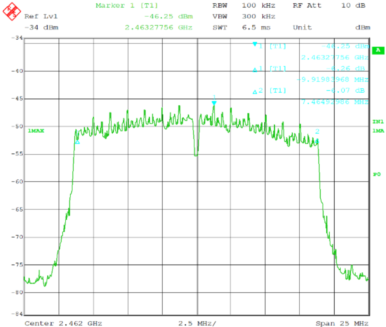
Figure 27 - 6dB Bandwidth, High Channel, 802.11g
