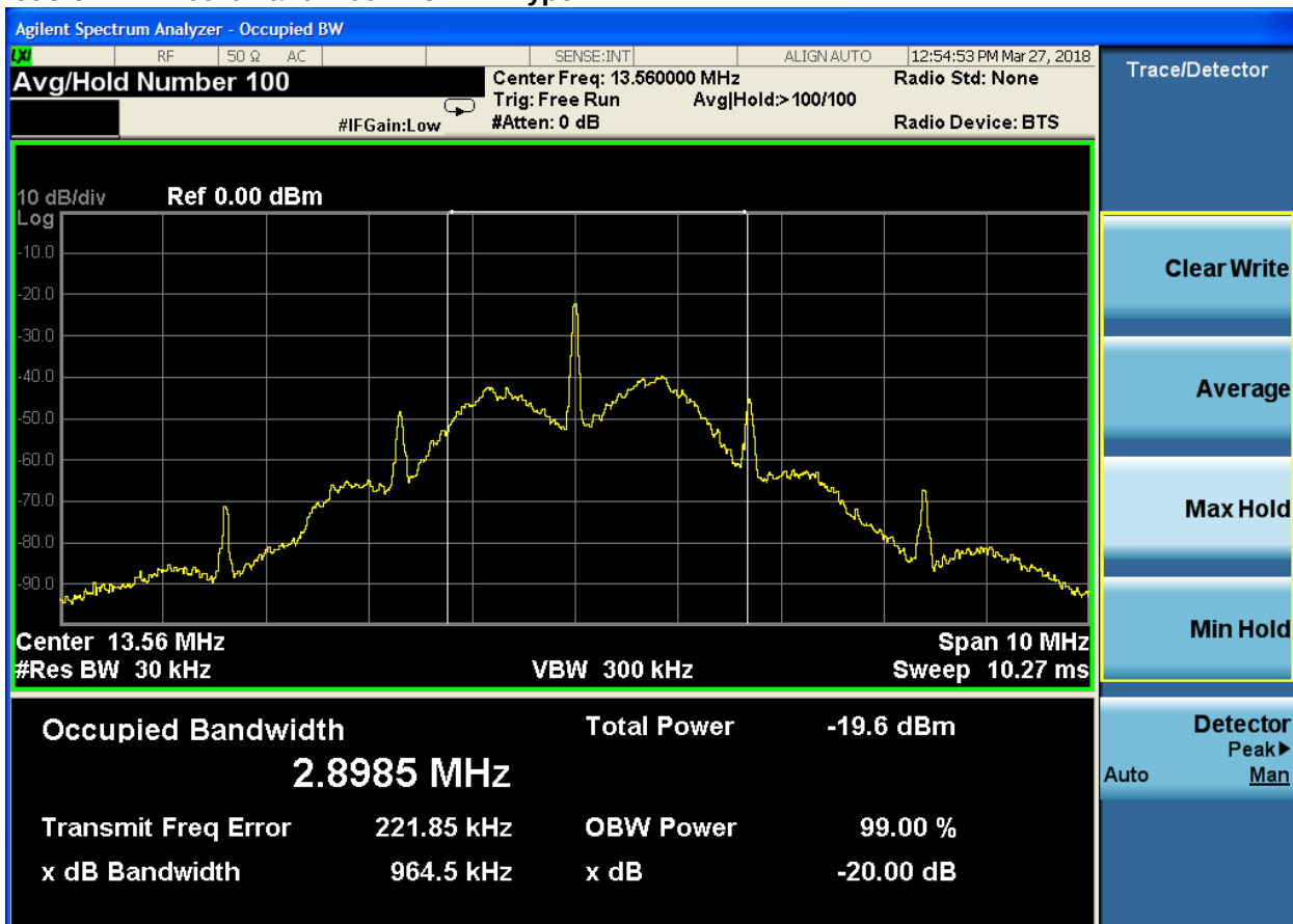
Plot 5-5: 99% Bandwidth – 3.2V – Type B
