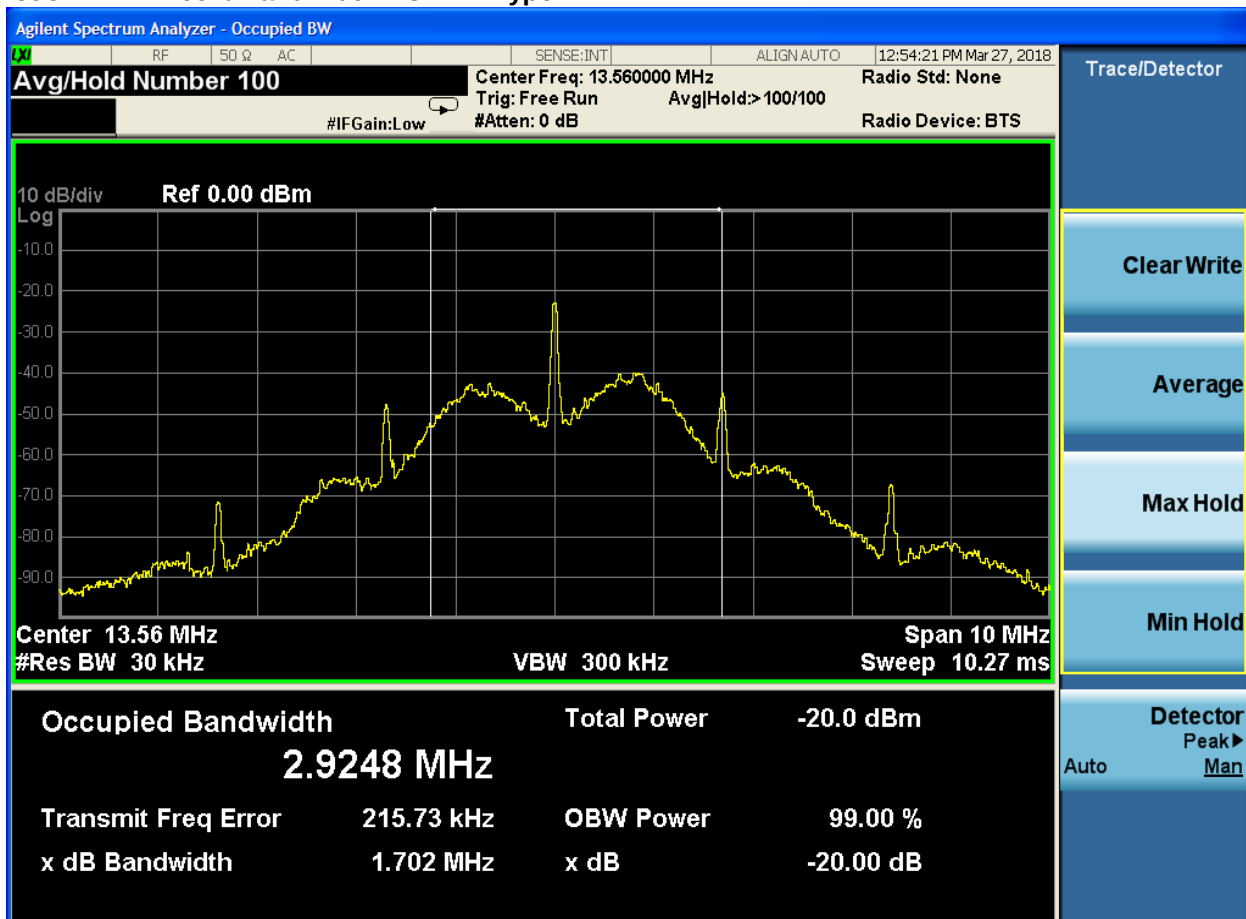
Plot 5-4: 99% Bandwidth – 3.2V – Type A
