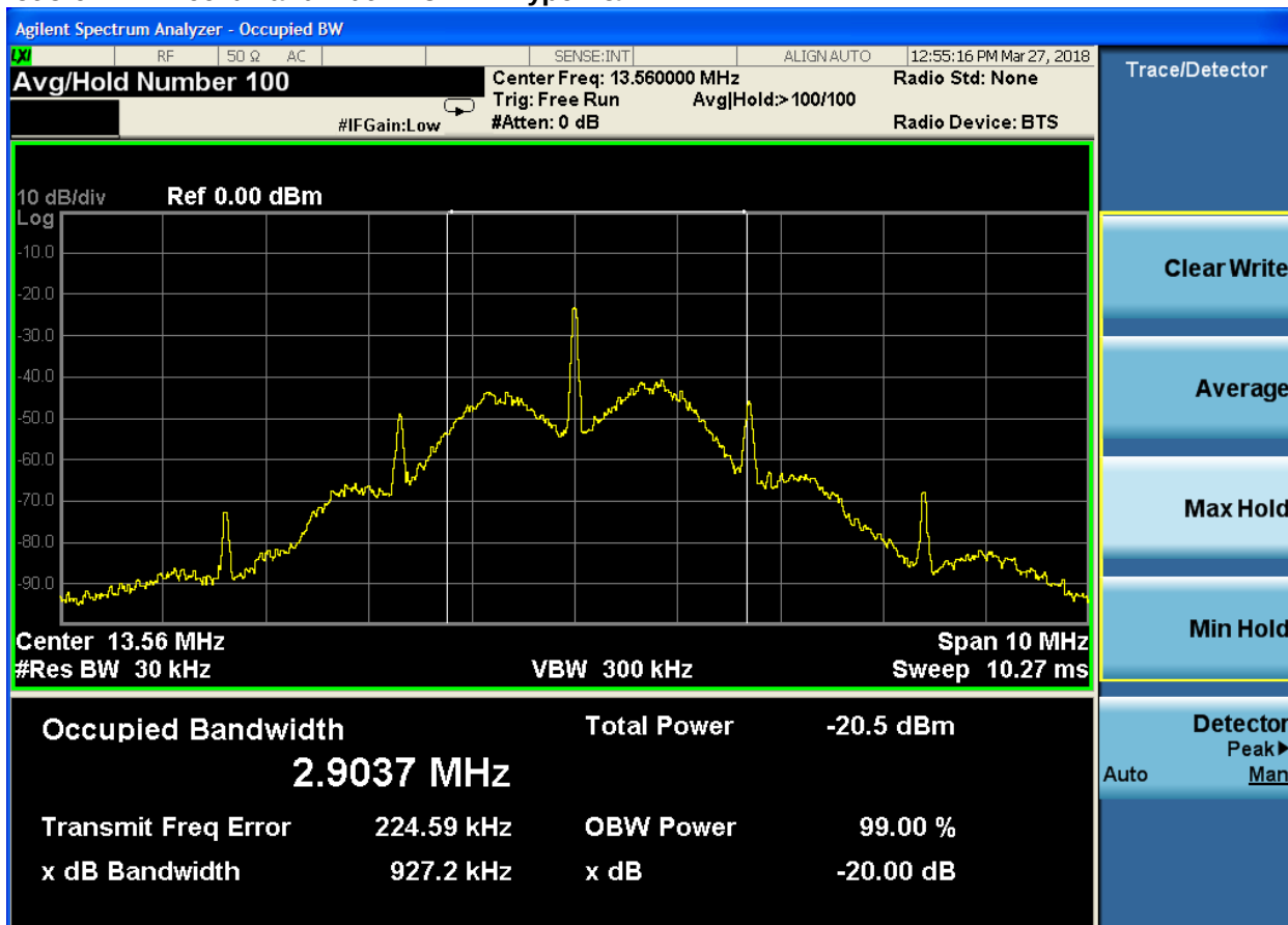
Plot 5-6: 99% Bandwidth – 3.2V – Type A&B
