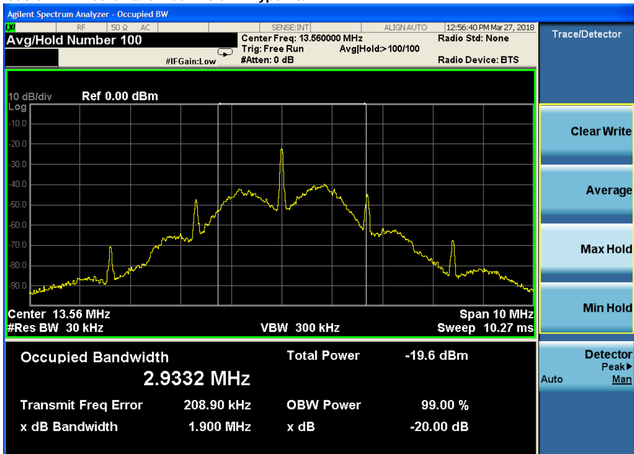
Plot 5-9: 99% Bandwidth – 3.9V – Type A&B
