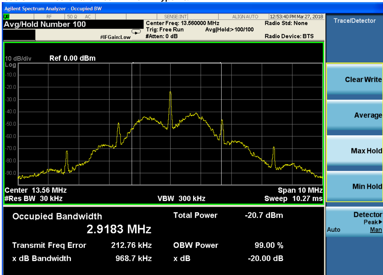
Plot 5-3: 99% Bandwidth – 4.75V – Type A&B
