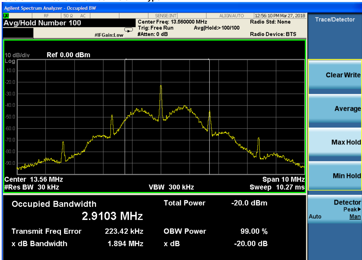
Plot 5-8: 99% Bandwidth – 3.9V – Type B
