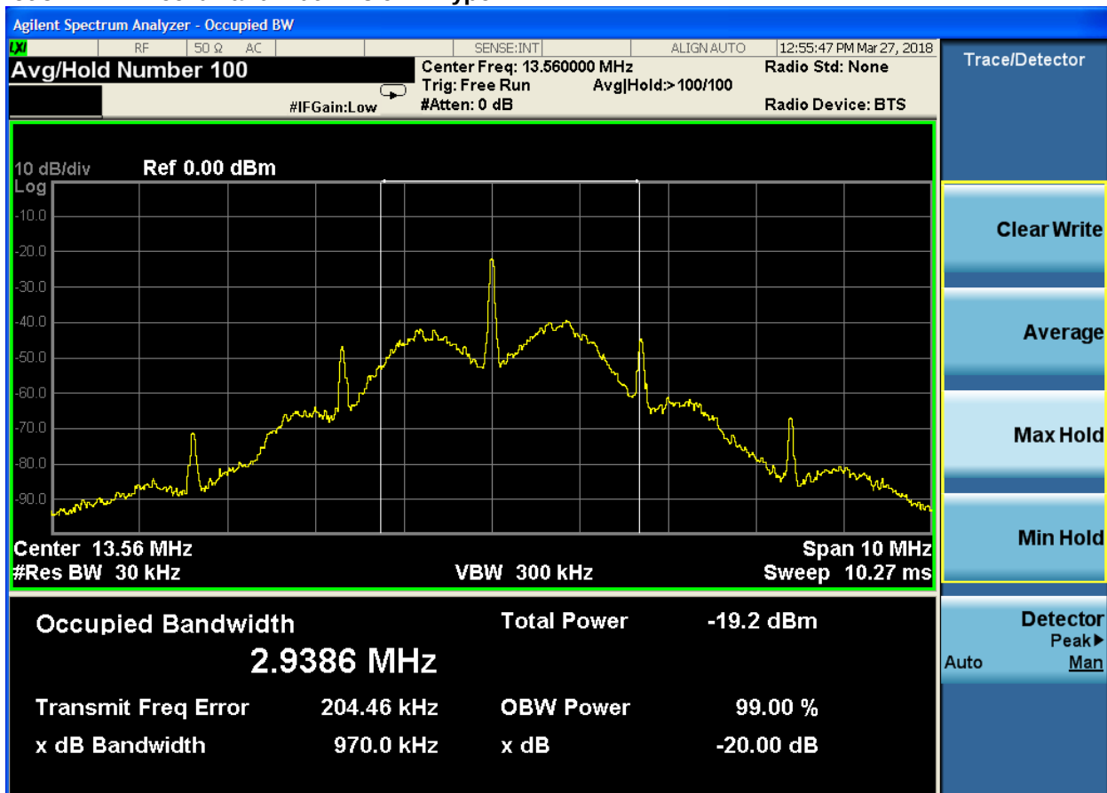
Plot 5-7: 99% Bandwidth – 3.9V – Type A
