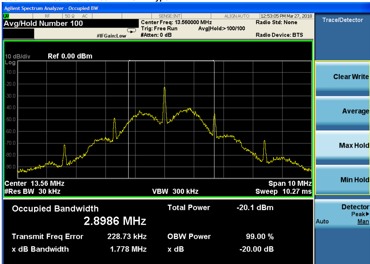
Plot 5-2: 99% Bandwidth – 4.75V – Type B
