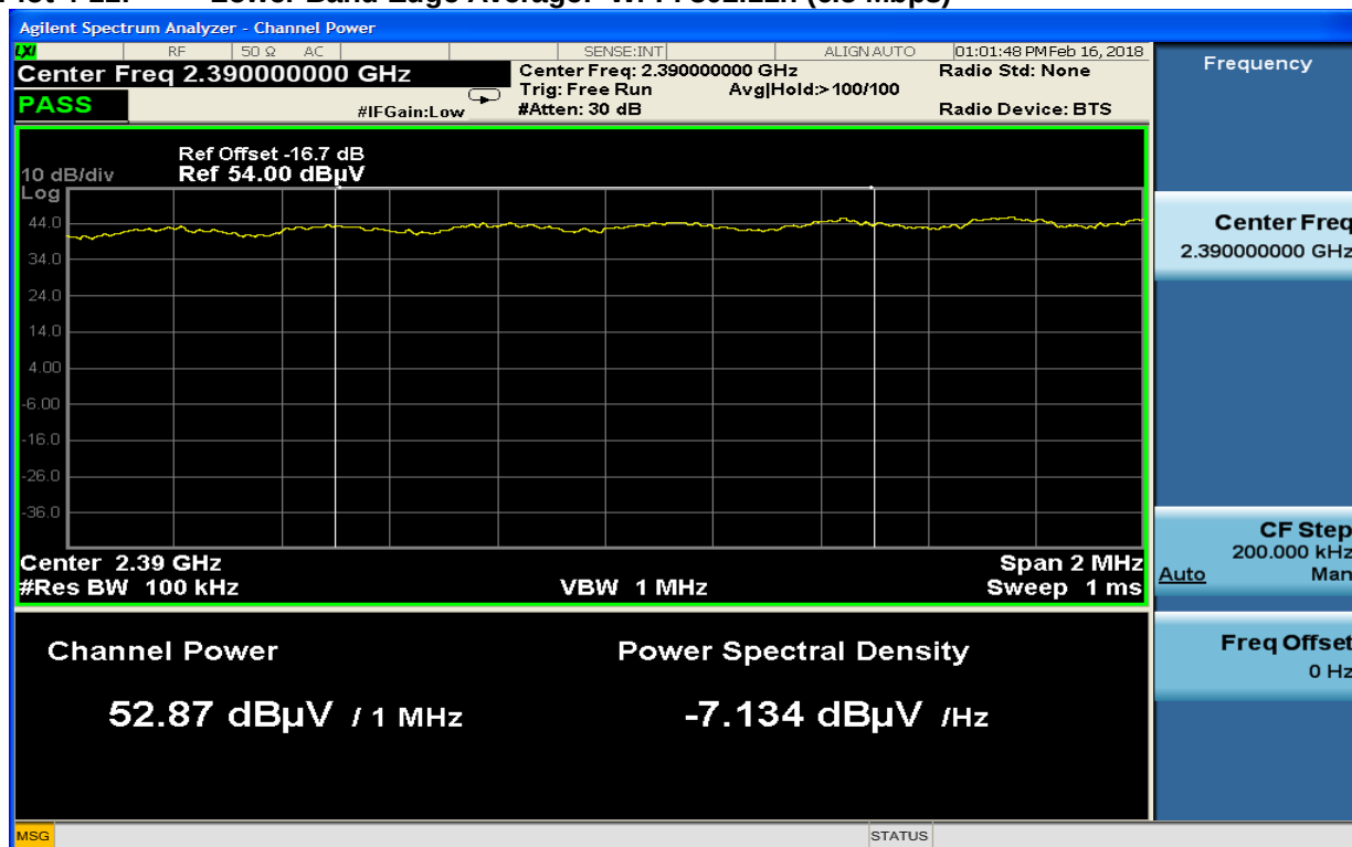
Plot 4-11: Lower Band Edge Average: Wi-Fi 802.11n (6.5 Mbps)
