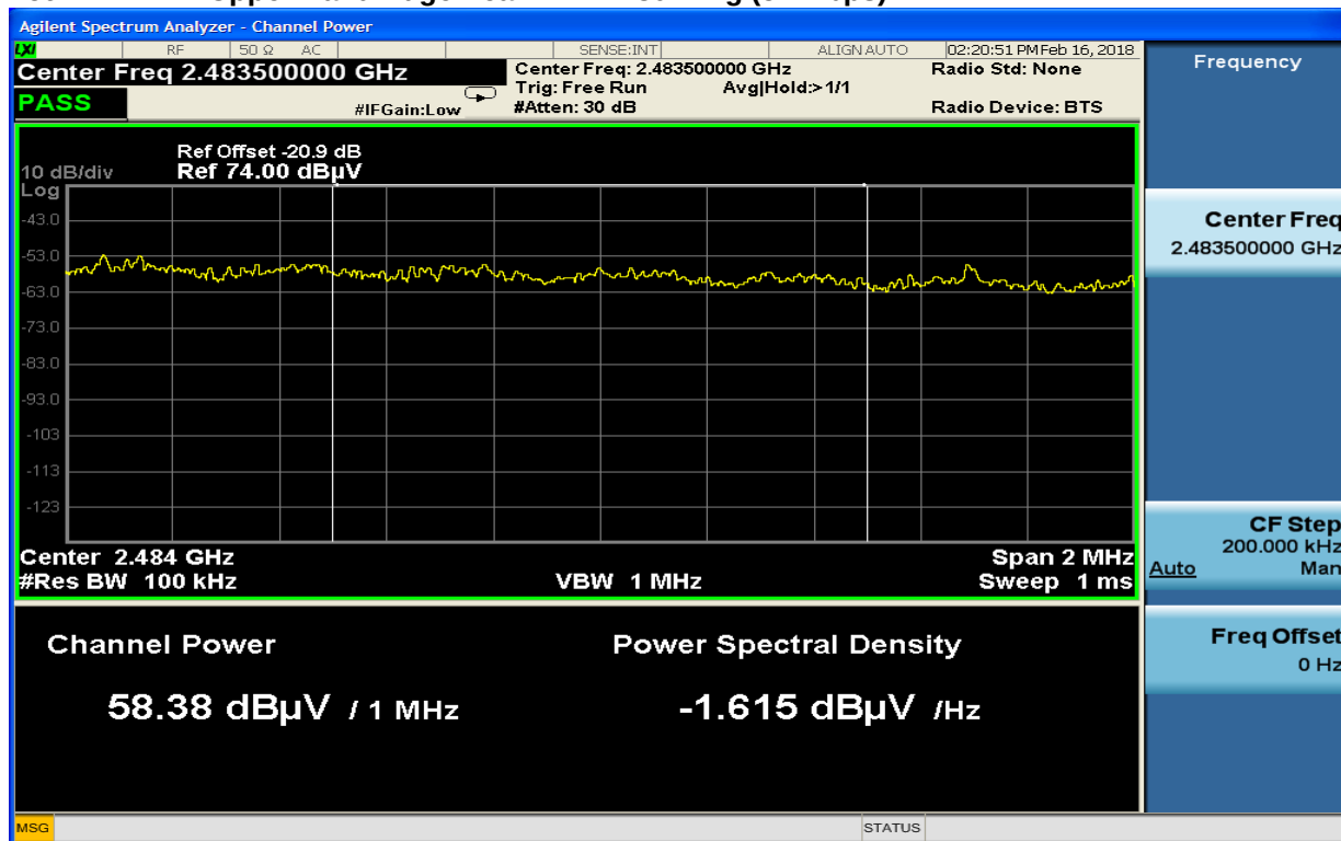
Plot 4-22: Upper Band Edge Peak: Wi-Fi 802.11g (54 Mbps)
