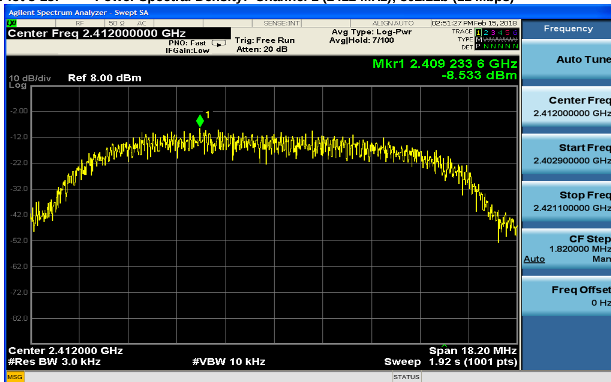
Plot 8-13: Power Spectral Density: Channel 1 (2412 MHz); 802.11b (11 Mbps)
