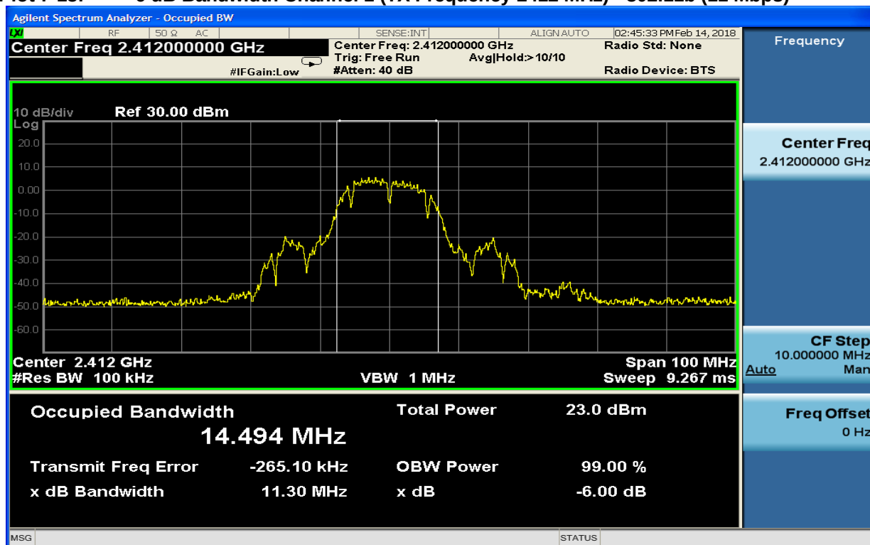
Plot 7-13: 6 dB Bandwidth Channel 1 (TX Frequency 2412 MHz) - 802.11b (11 Mbps)
