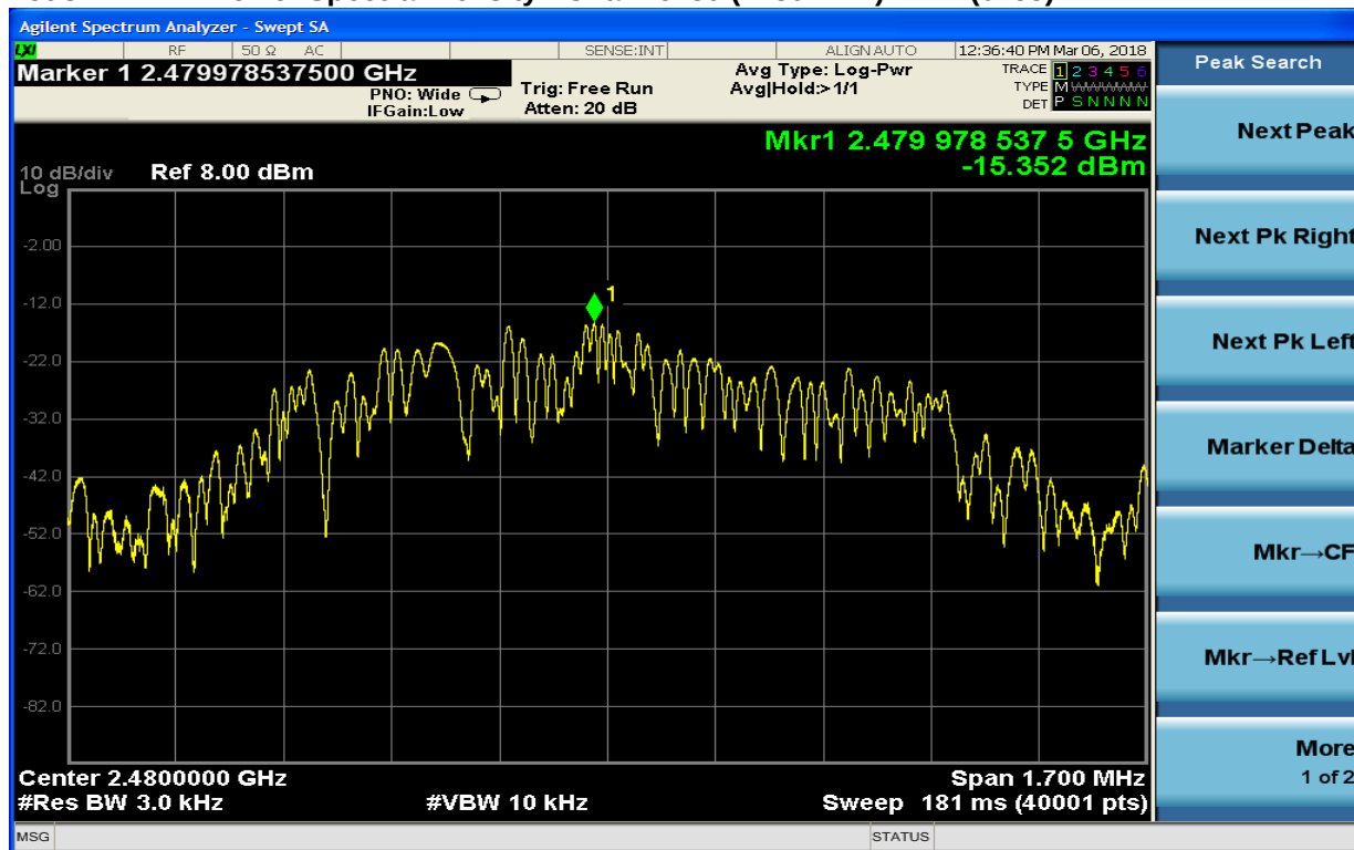
Plot 8-12: Power Spectral Density: Channel 39 (2480 MHz): BLE (0x55)
