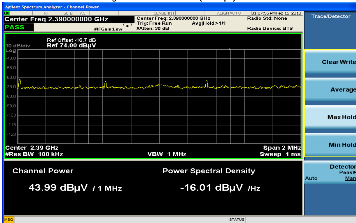
Plot 4-8: Lower Band Edge Peak: Wi Fi 802.11b (11 Mbps)
