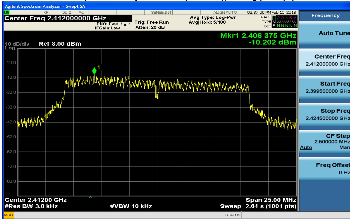
Plot 8-16: Power Spectral Density: Channel 1 (2412 MHz); 802.11g (54 Mbps)
