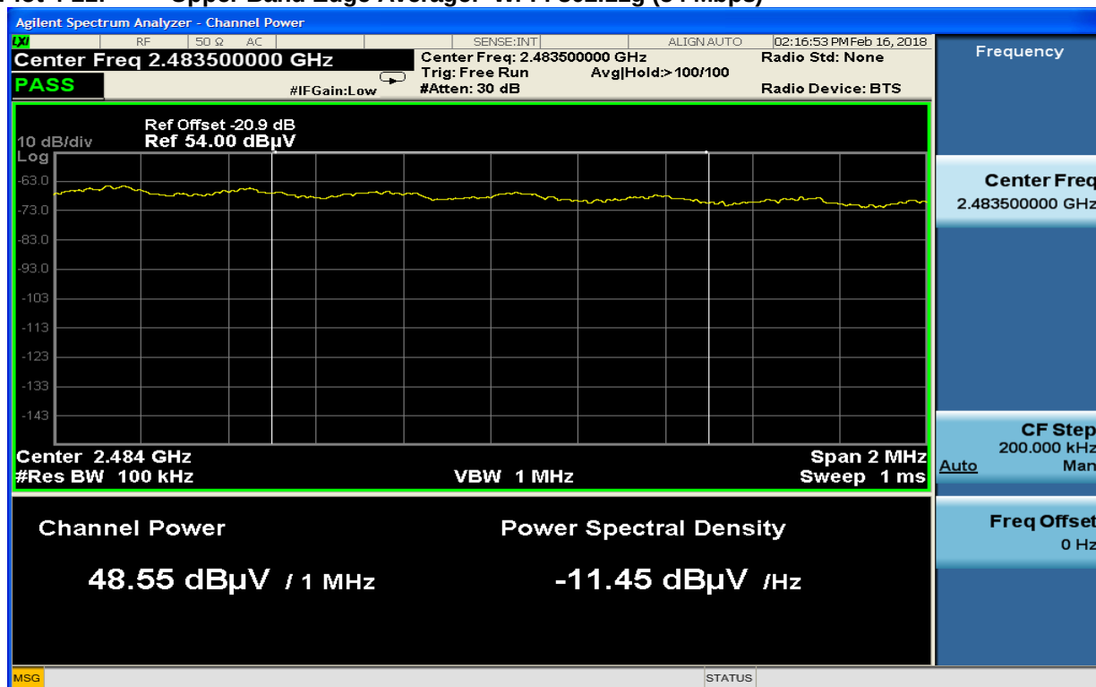
Plot 4-21: Upper Band Edge Average: Wi-Fi 802.11g (54 Mbps)
