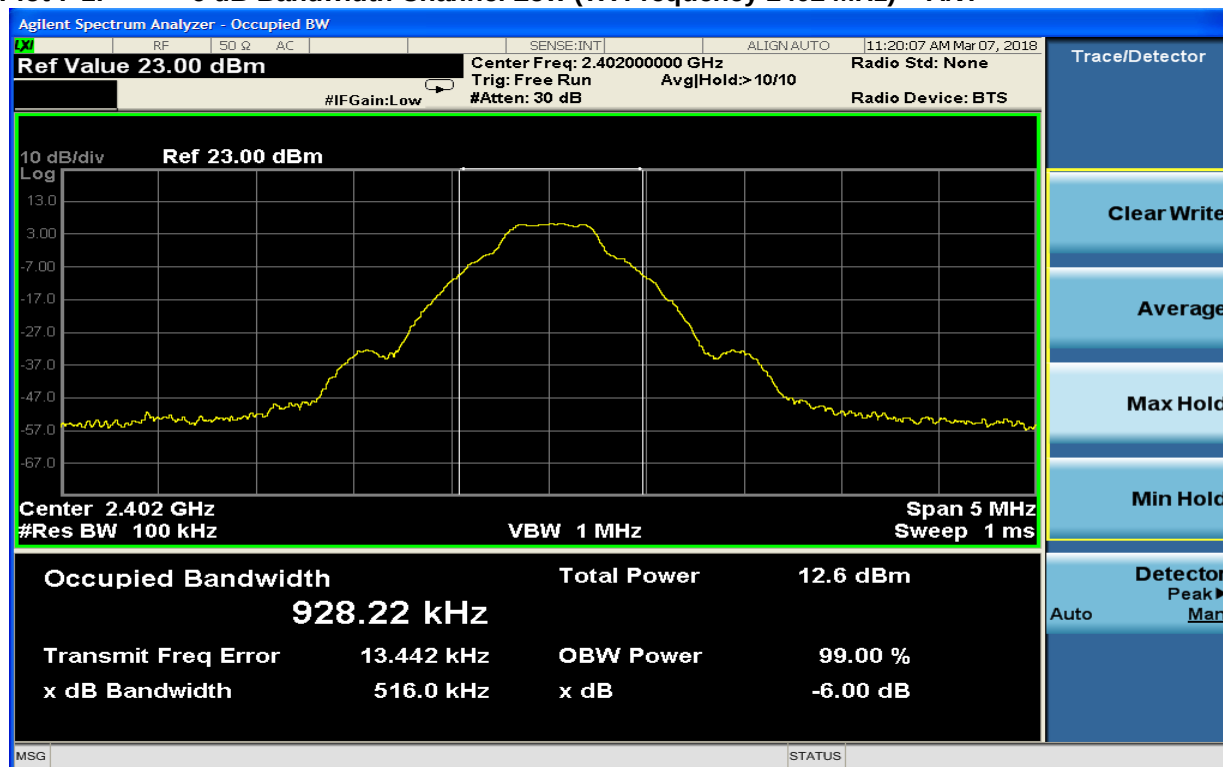
Plot 7-1: 6 dB Bandwidth Channel Low (TX Frequency 2402 MHz) – ANT+
