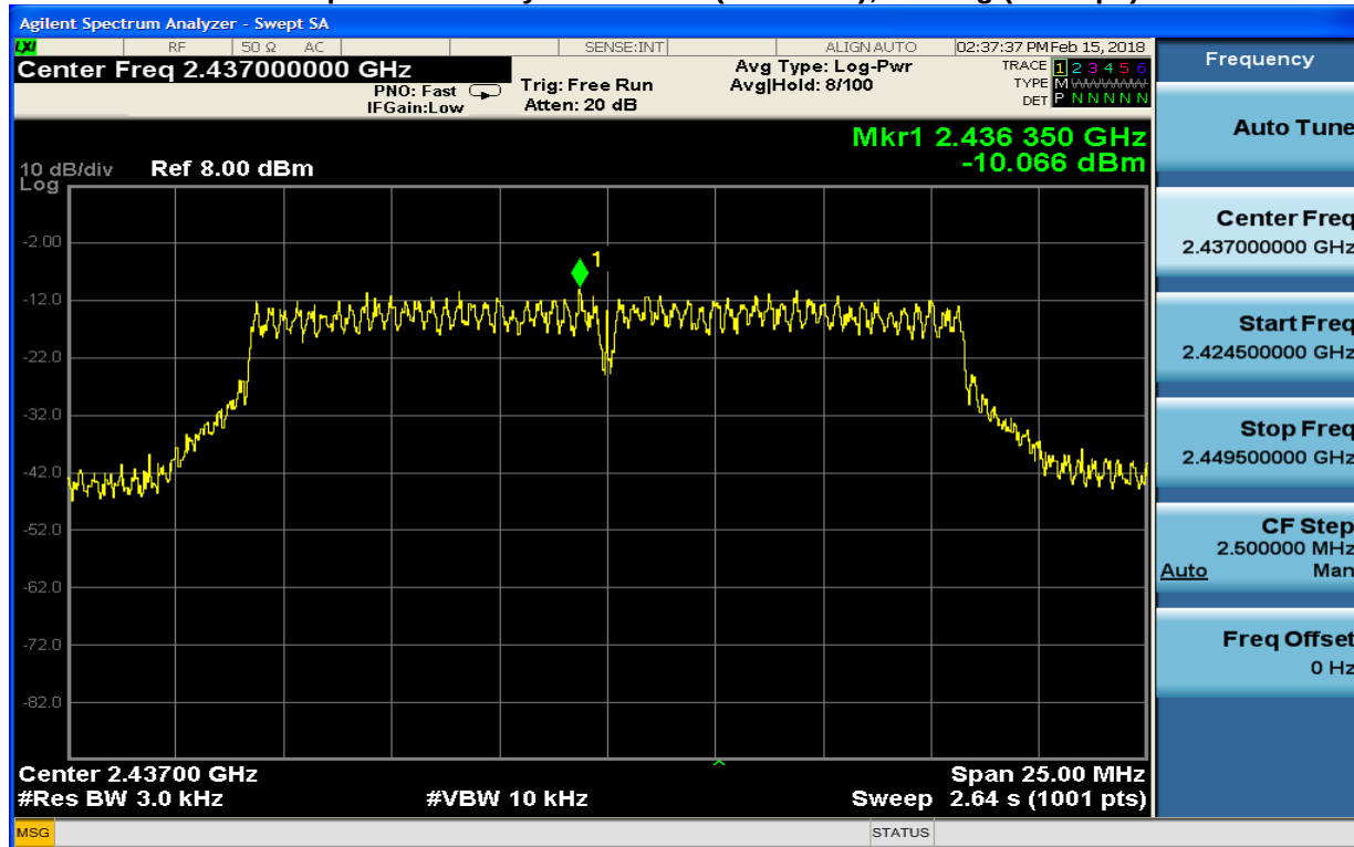
Plot 8-17: Power Spectral Density: Channel 6 (2437 MHz); 802.11g (54 Mbps)
