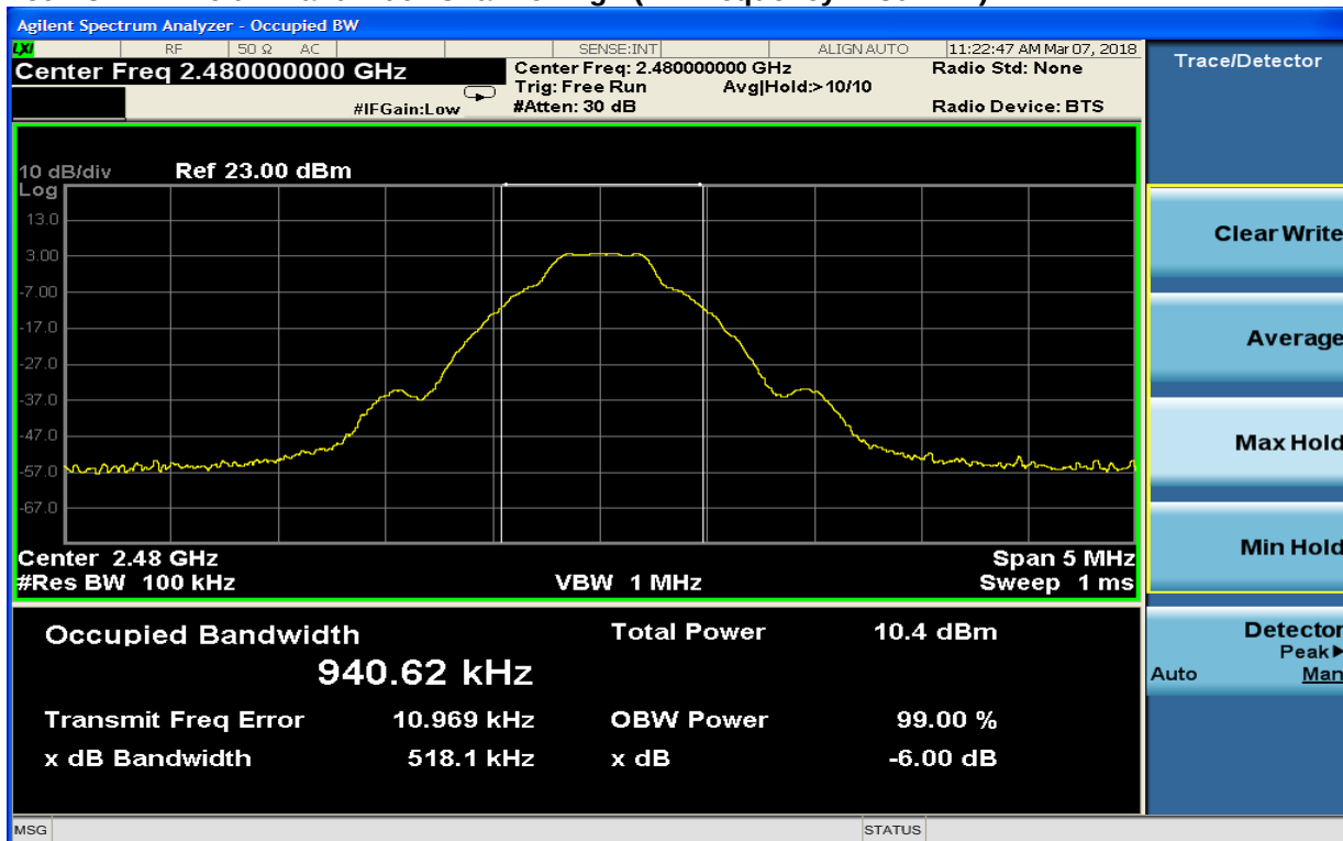
Plot 7-3: 6 dB Bandwidth Channel High (TX Frequency 2480 MHz) - ANT+
