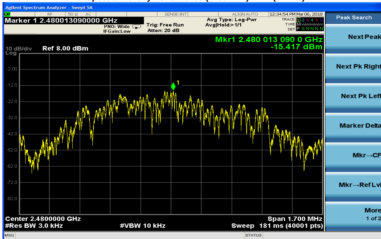
Plot 8-6: Power Spectral Density: Channel 39 (2480 MHz): BLE (PRB29)
