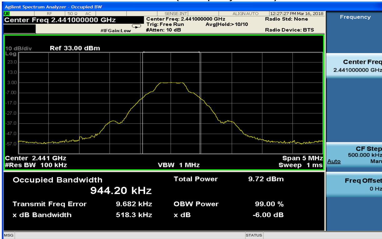
Plot 7-2: 6 dB Bandwidth Channel Mid (TX Frequency 2441 MHz) - ANT+
