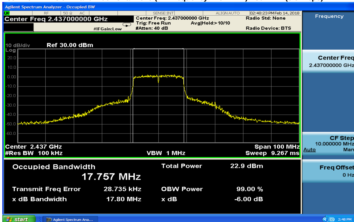
Plot 7-20: 6 dB Bandwidth Channel 6 (TX Frequency 2437 MHz) - 802.11n (6.5 Mbps)
