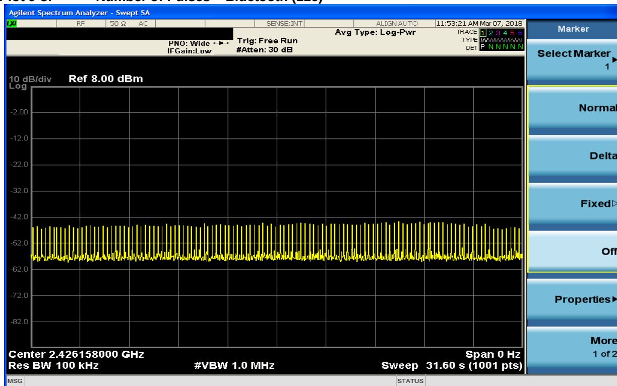
Plot 9-3: Number of Pulses – Bluetooth (116)
