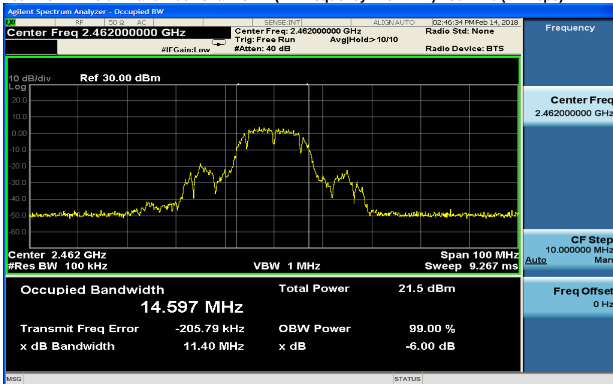
Plot 7-15: 6 dB Bandwidth Channel 11 (TX Frequency 2462 MHz) - 802.11b (11 Mbps)
