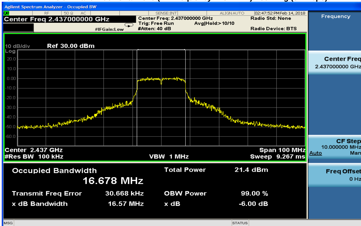
Plot 7-17: 6 dB Bandwidth Channel 6 (TX Frequency 2437 MHz) - 802.11g (54 Mbps)
