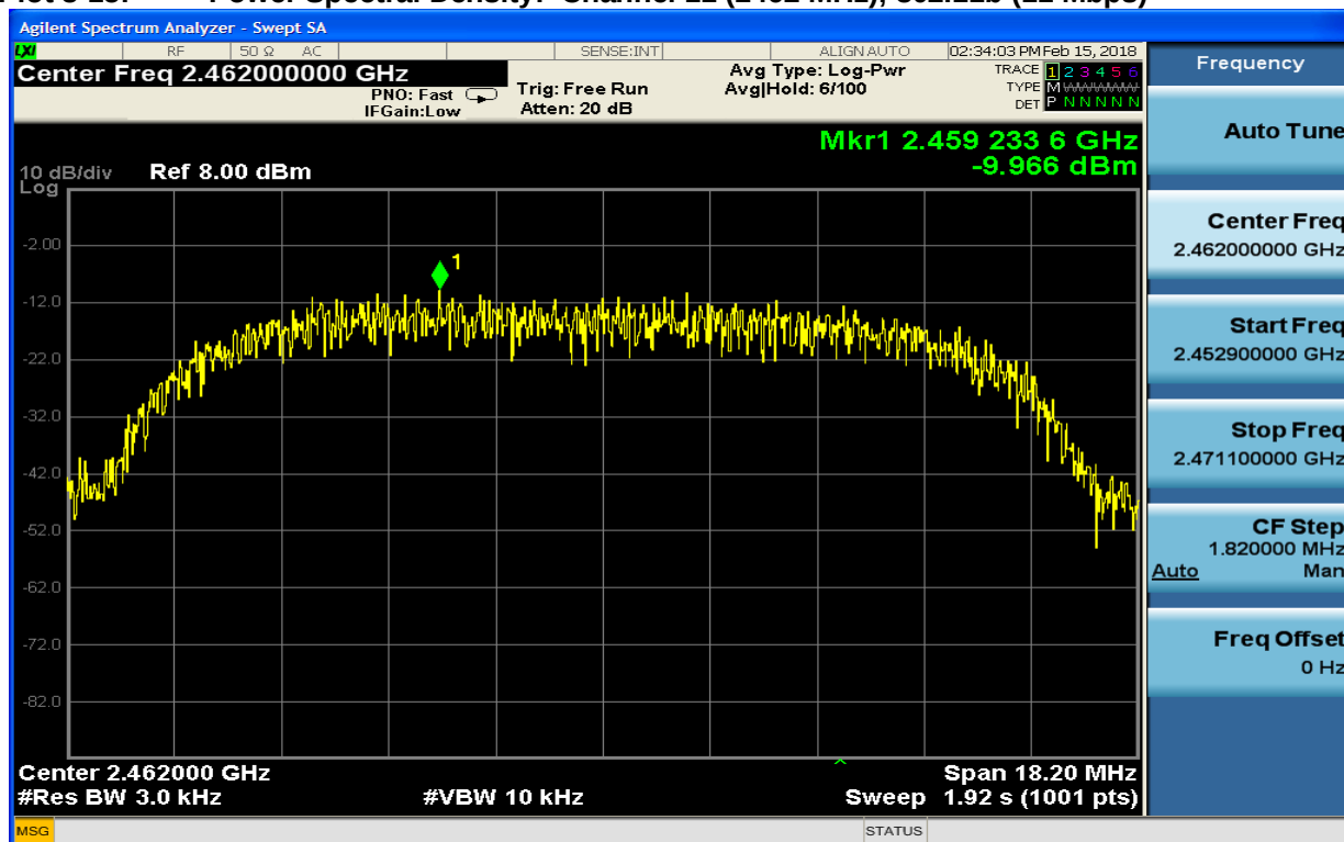
Plot 8-15: Power Spectral Density: Channel 11 (2462 MHz); 802.11b (11 Mbps)
