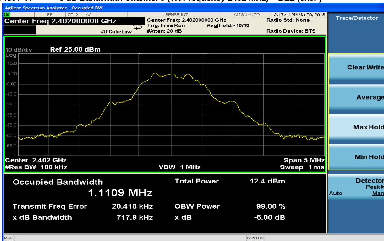
Plot 7-7: 6 dB Bandwidth Channel 0 (TX Frequency 2402 MHz) – BLE (0x0F)
