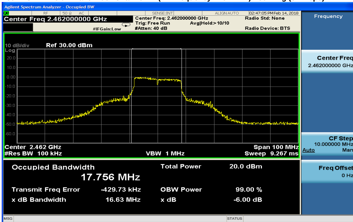
Plot 7-18: 6 dB Bandwidth Channel 11 (TX Frequency 2462 MHz) - 802.11g (54 Mbps)
