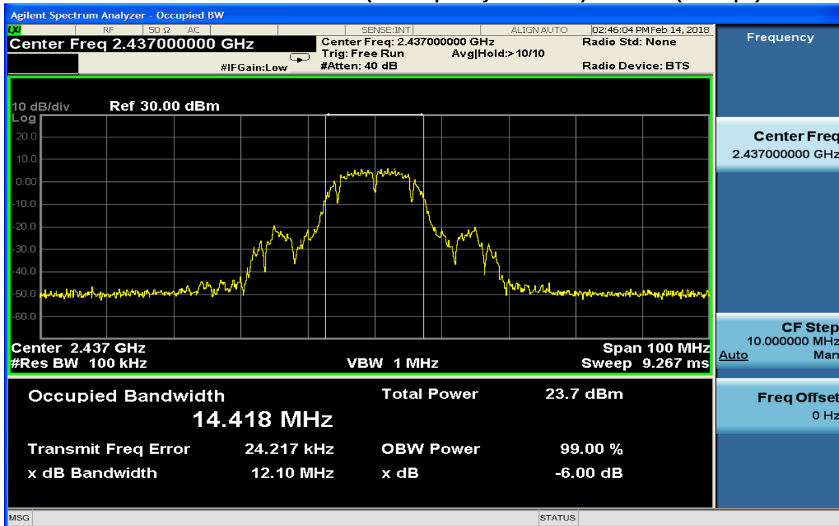
Plot 7-14: 6 dB Bandwidth Channel 6 (TX Frequency 2437 MHz) - 802.11b (11 Mbps)
