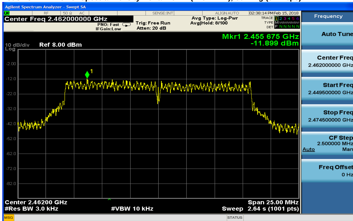
Plot 8-18: Power Spectral Density: Channel 11 (2462 MHz); 802.11g (54 Mbps)
