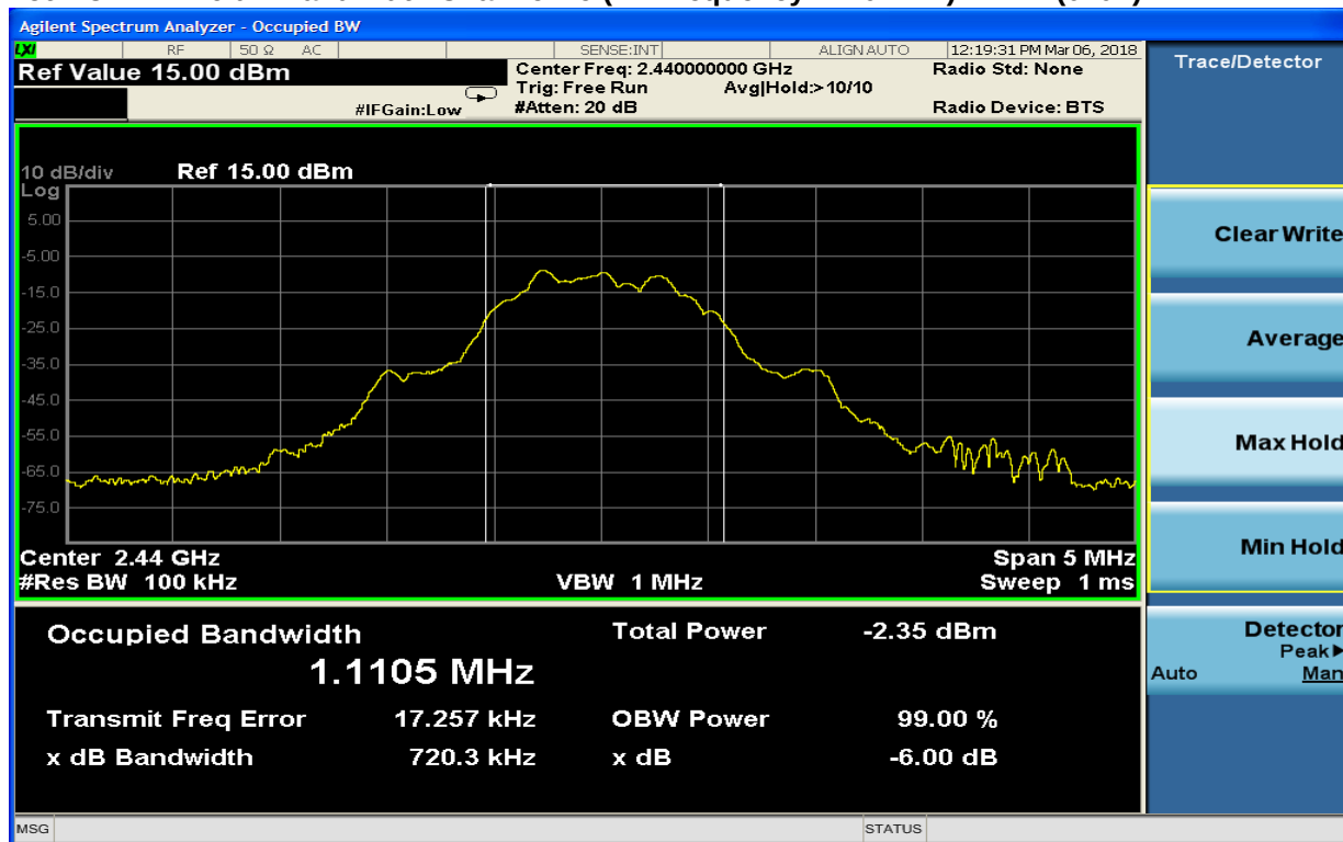
Plot 7-8: 6 dB Bandwidth Channel 19 (TX Frequency 2440 MHz) – BLE (0x0F)
