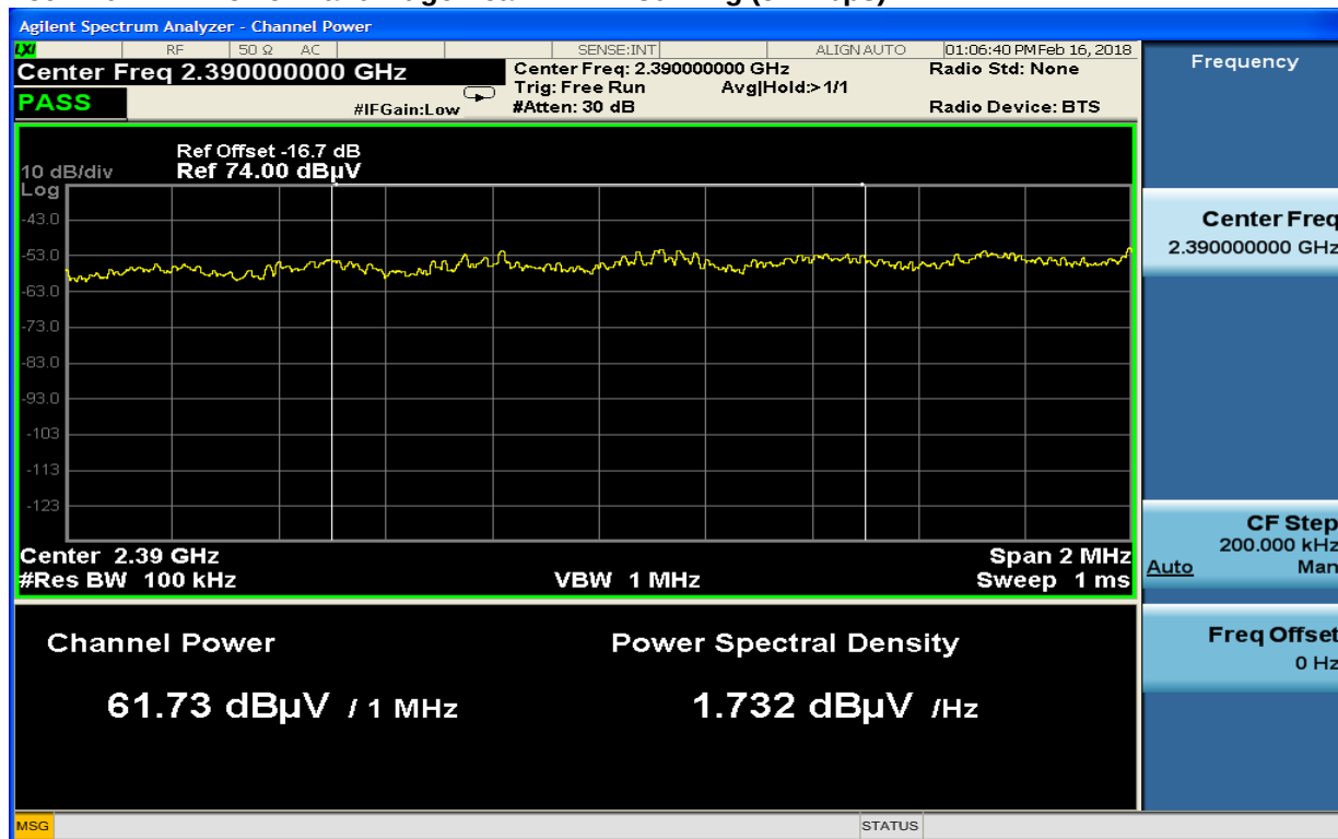
Plot 4-10: Lower Band Edge Peak: Wi-Fi 802.11g (54 Mbps)
