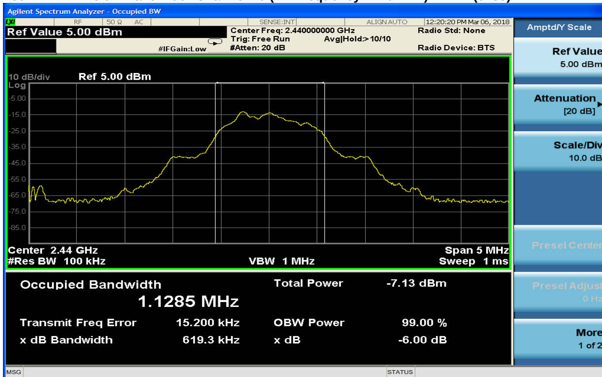
Plot 7-11: 6 dB Bandwidth Channel 19 (TX Frequency 2440 MHz) – BLE (0x55)
