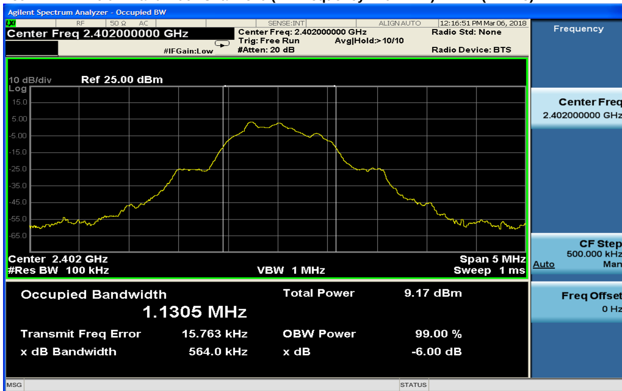
Plot 7-4: 6 dB Bandwidth Channel 0 (TX Frequency 2402 MHz) – BLE (PRB29)
