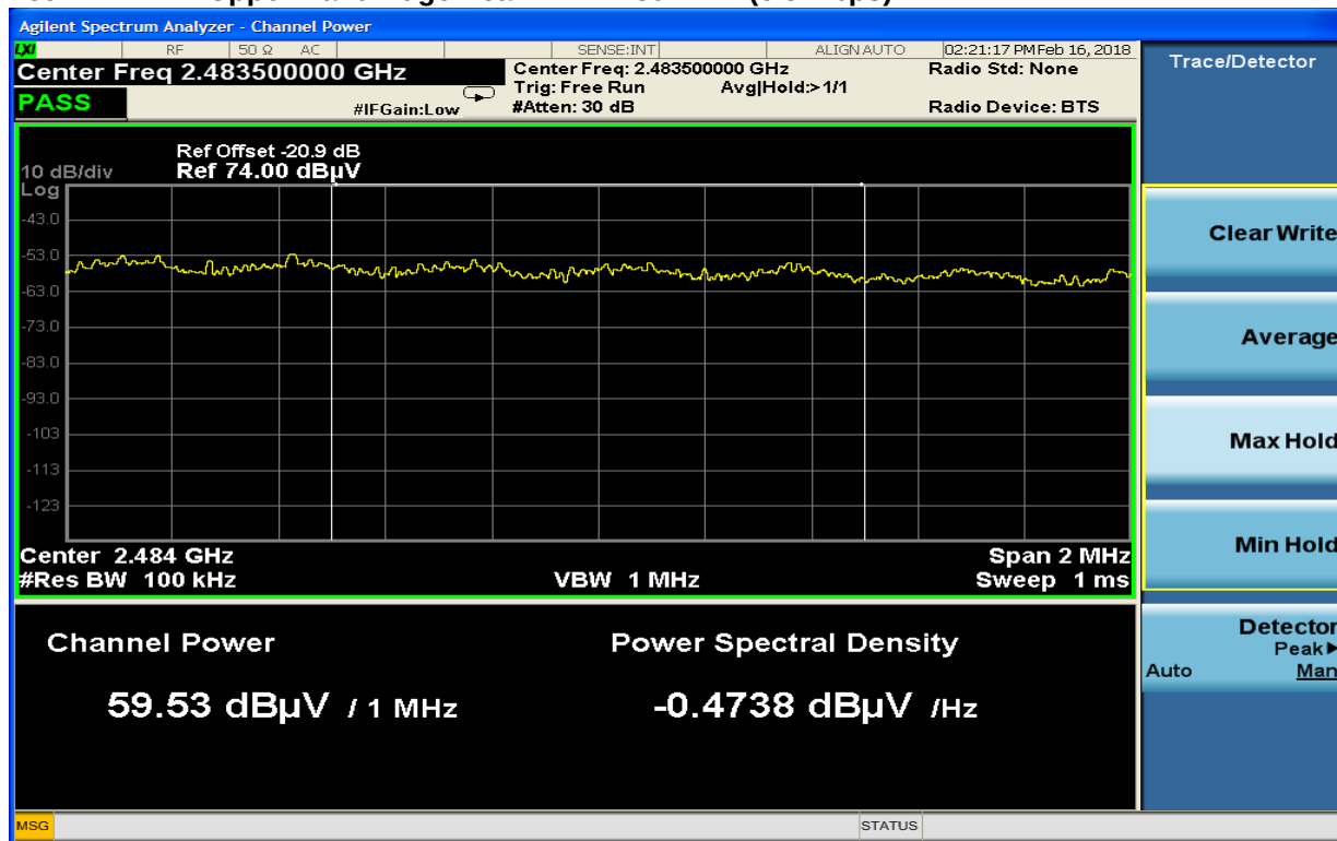
Plot 4-24: Upper Band Edge Peak: Wi-Fi 802.11n (6.5 Mbps)
