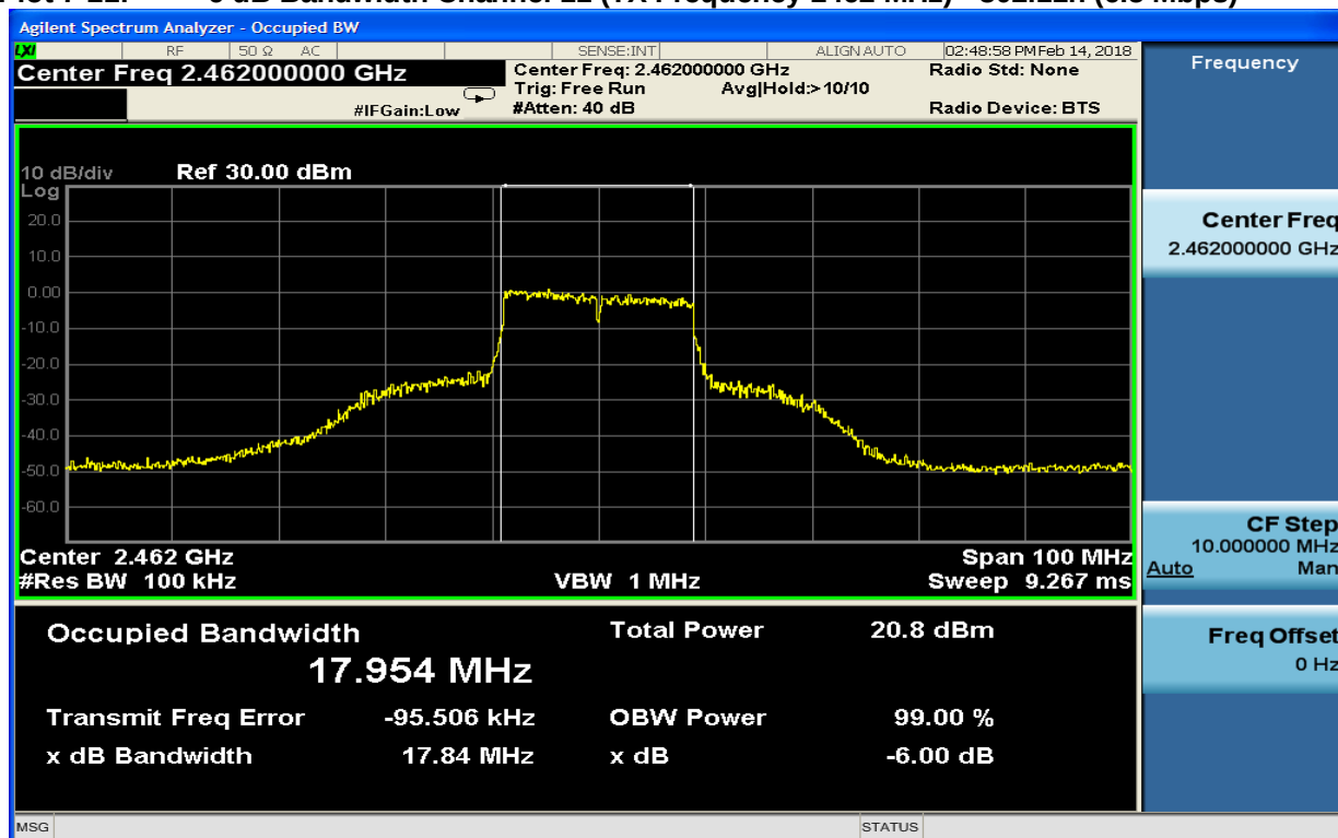
Plot 7-21: 6 dB Bandwidth Channel 11 (TX Frequency 2462 MHz) - 802.11n (6.5 Mbps)
