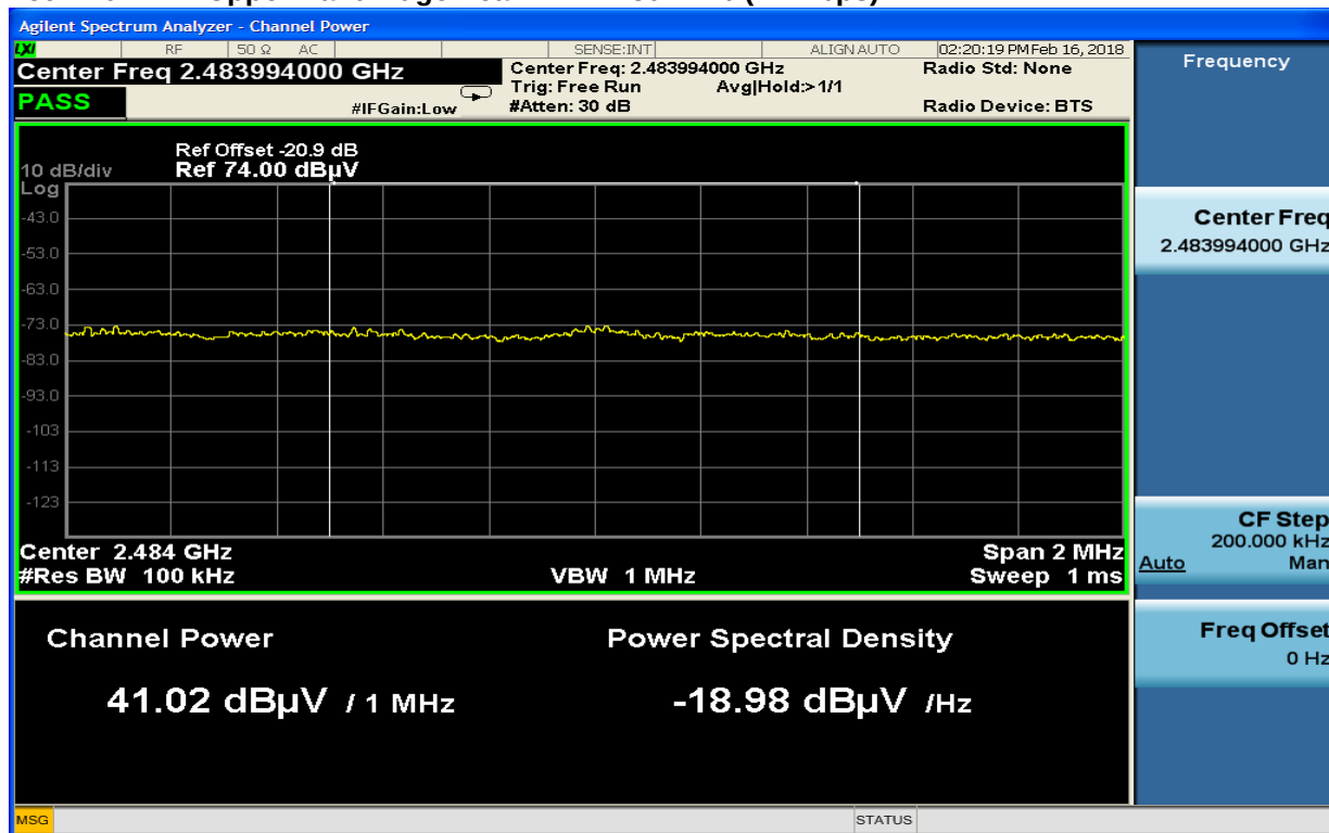
Plot 4-20: Upper Band Edge Peak: Wi-Fi 802.11b (11 Mbps)
