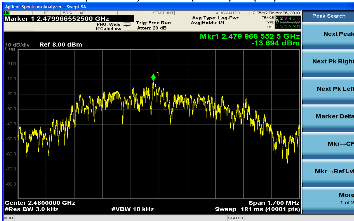
Plot 8-9: Power Spectral Density: Channel 39 (2480 MHz): BLE (0x0F)
