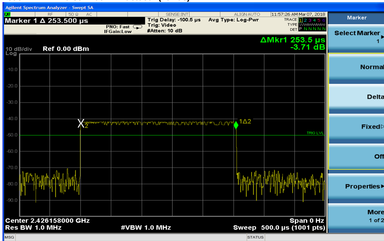
Plot 9-4: Pulse Width – Bluetooth (254 us)
