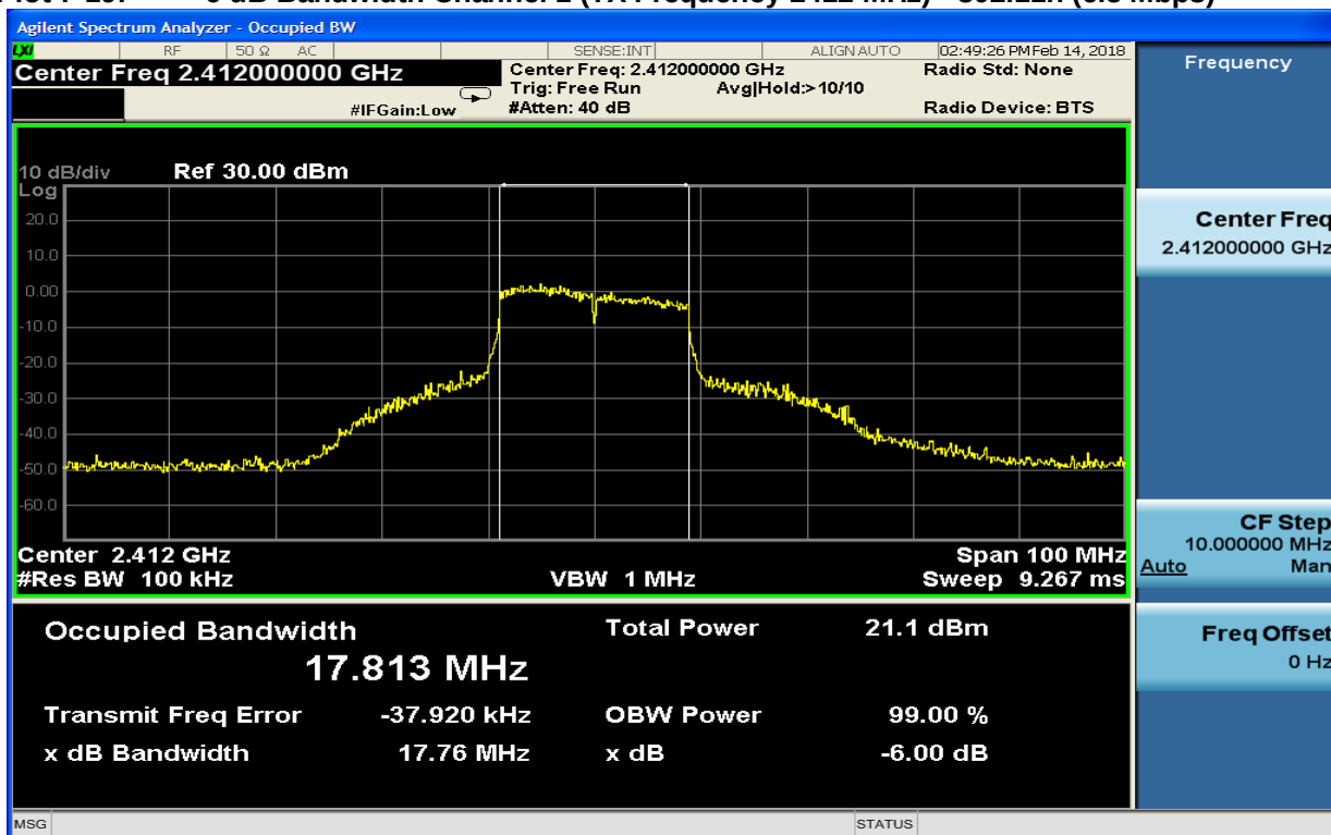
Plot 7-19: 6 dB Bandwidth Channel 1 (TX Frequency 2412 MHz) - 802.11n (6.5 Mbps)
