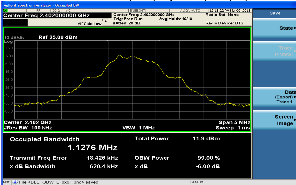
Plot 7-10: 6 dB Bandwidth Channel 0 (TX Frequency 2402 MHz) – BLE (0x55)
