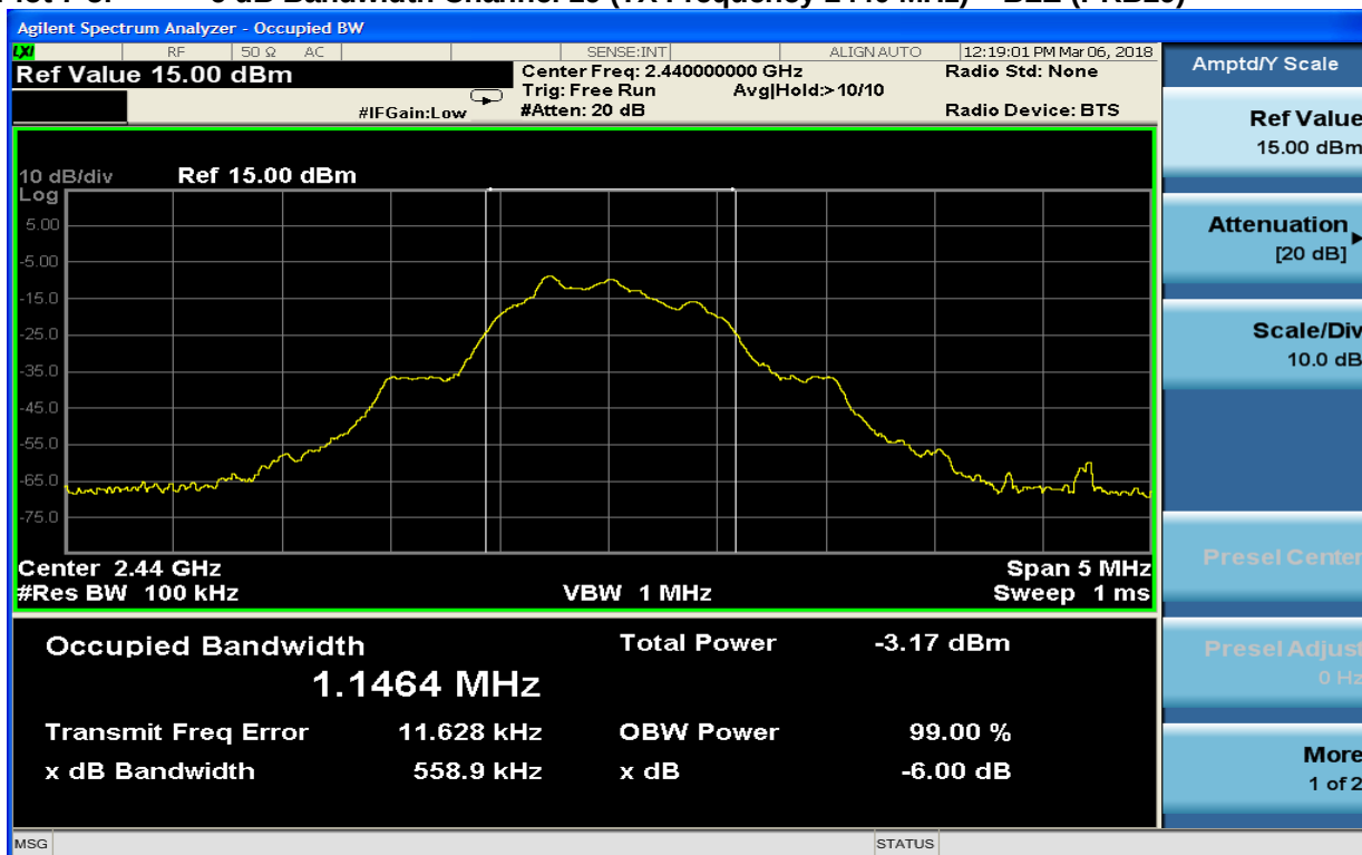
Plot 7-5: 6 dB Bandwidth Channel 19 (TX Frequency 2440 MHz) – BLE (PRB29)
