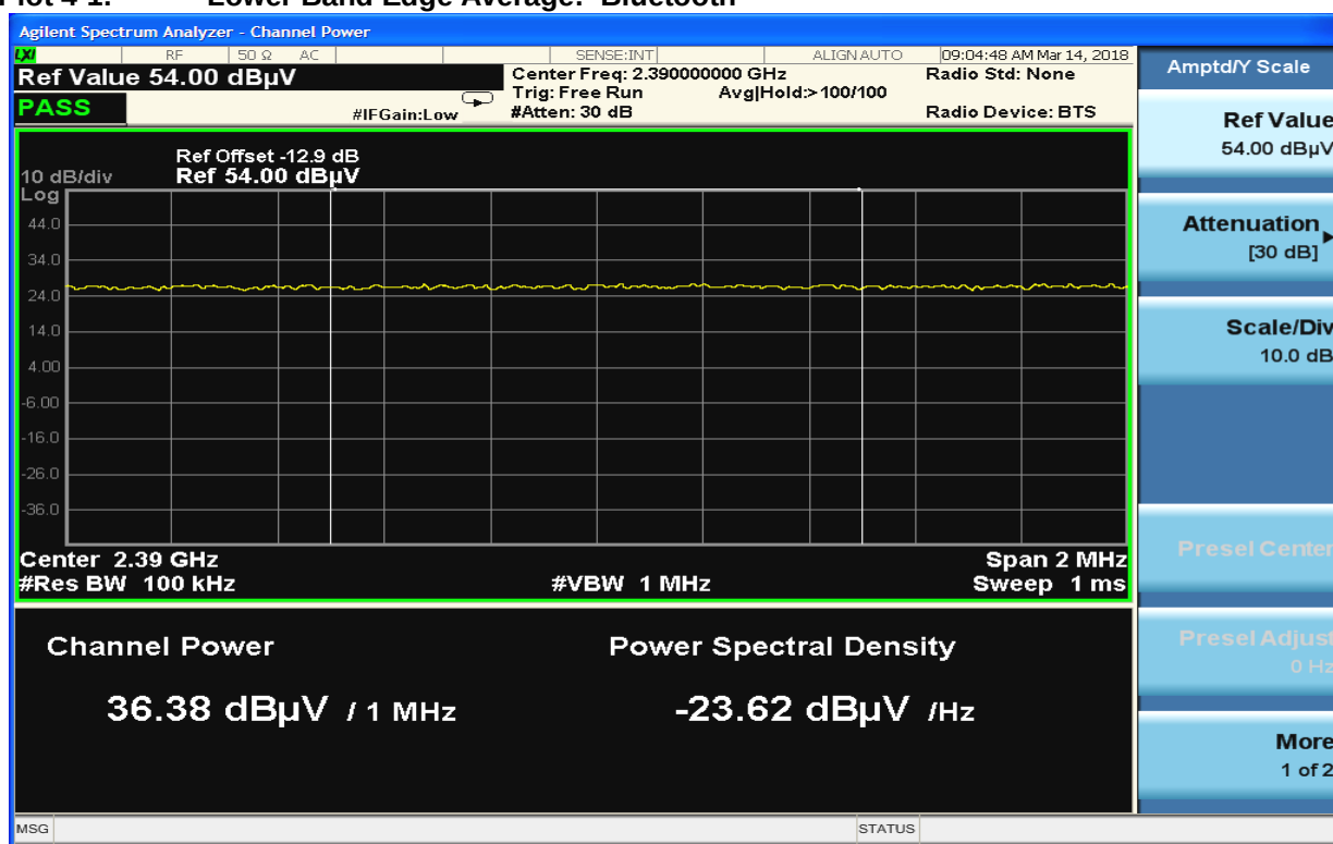
Plot 4-1: Lower Band Edge Average: Bluetooth
