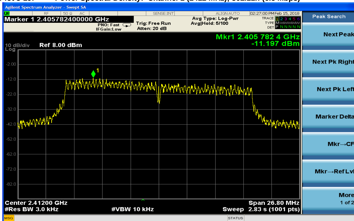
Plot 8-19: Power Spectral Density: Channel 1 (2412 MHz); 802.11n (6.5 Mbps)
