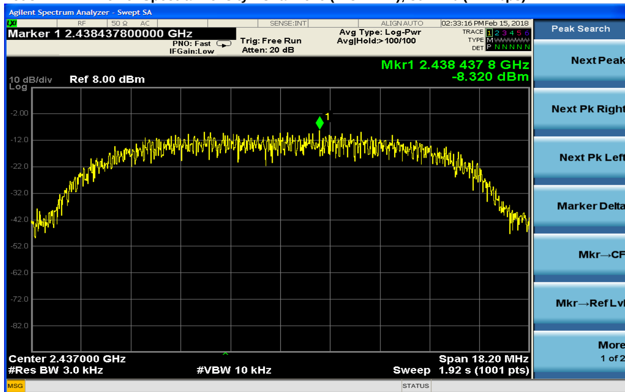
Plot 8-14: Power Spectral Density: Channel 6 (2437 MHz); 802.11b (11 Mbps)
