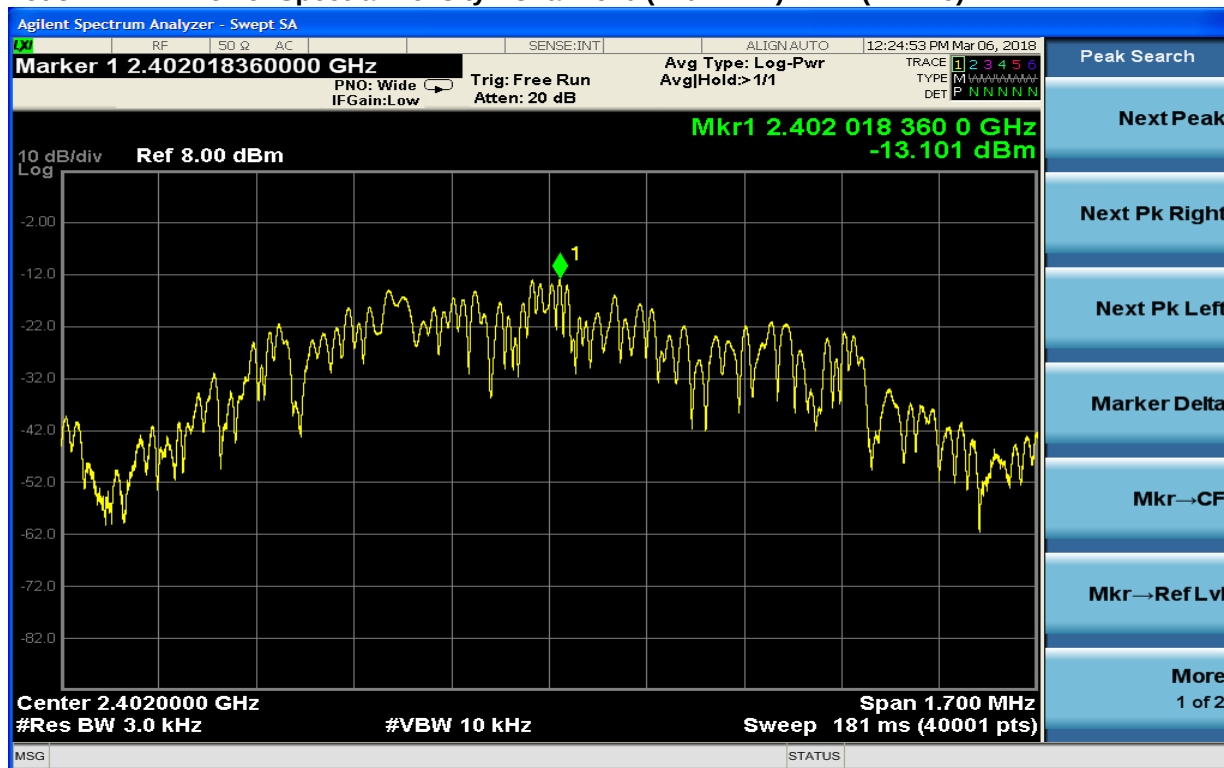
Plot 8-4: Power Spectral Density: Channel 0 (2402 MHz): BLE (PRB29)
