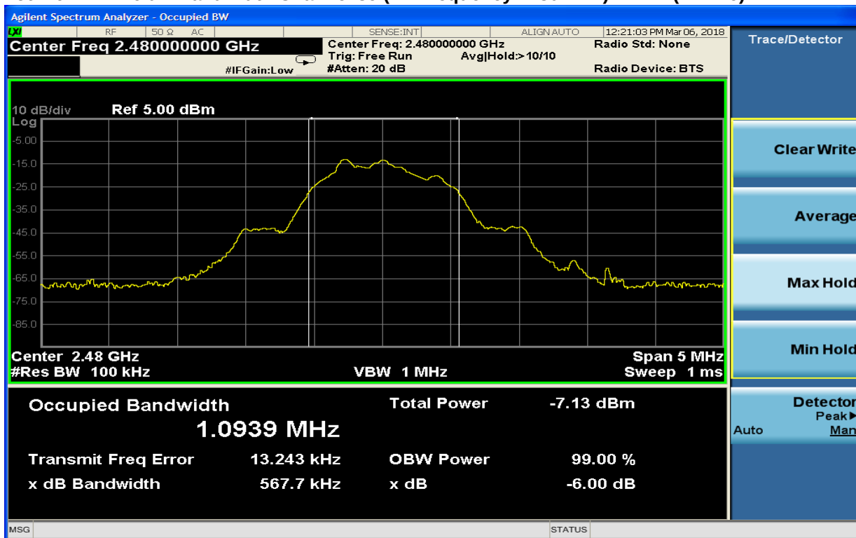
Plot 7-6: 6 dB Bandwidth Channel 39 (TX Frequency 2480 MHz) – BLE (PRB29)
