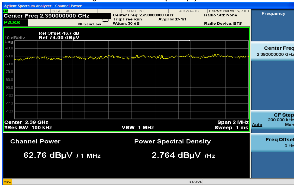
Plot 4-12: Lower Band Edge Peak: Wi-Fi 802.11n (6.5 Mbps)
