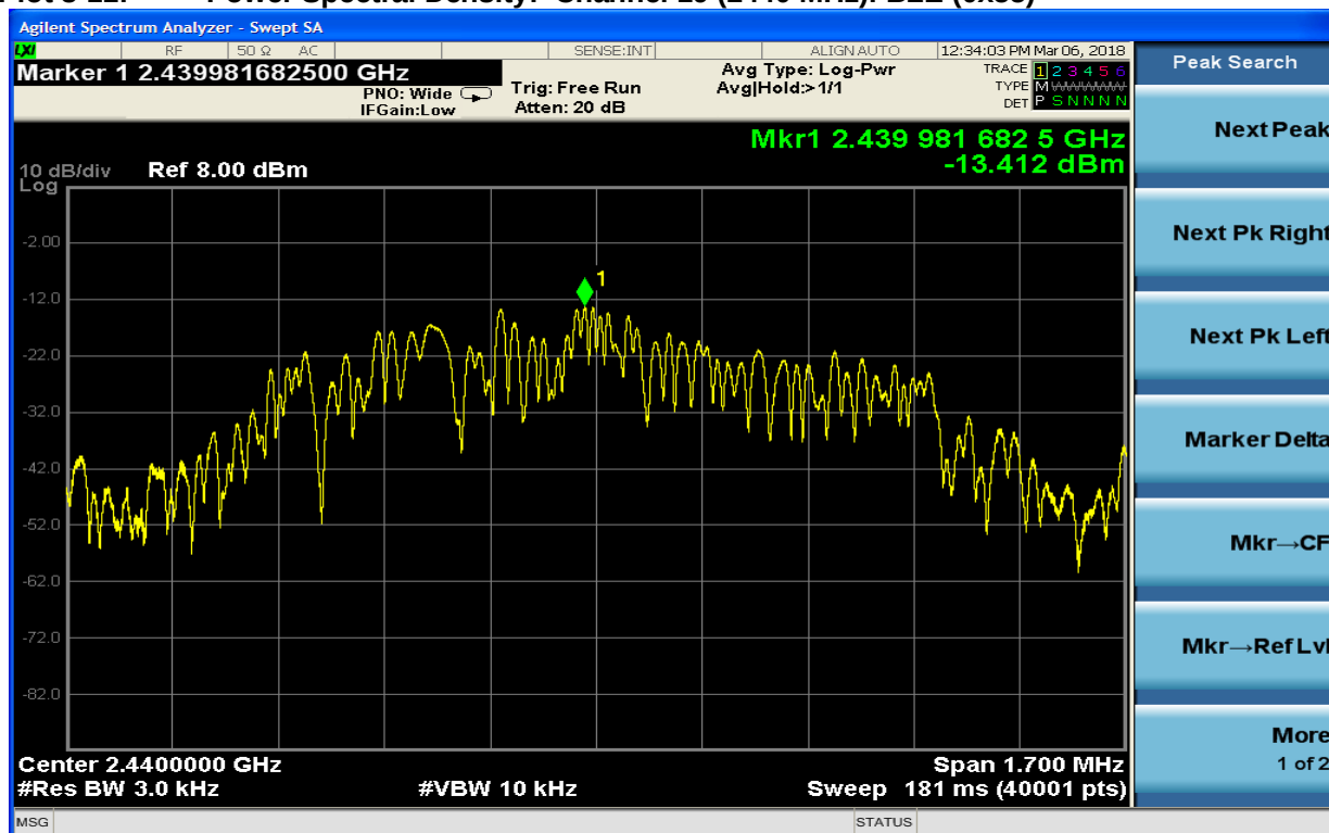
Plot 8-11: Power Spectral Density: Channel 19 (2440 MHz): BLE (0x55)
