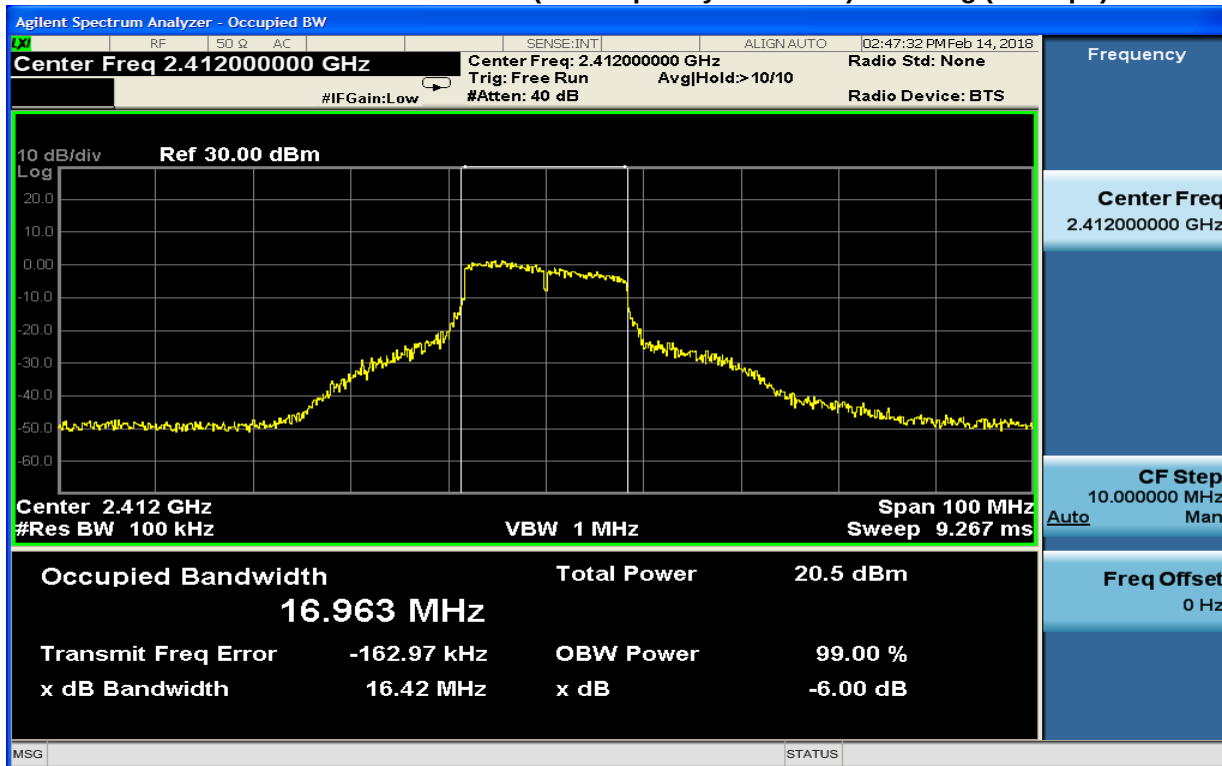
Plot 7-16: 6 dB Bandwidth Channel 1 (TX Frequency 2412 MHz) - 802.11g (54 Mbps)
