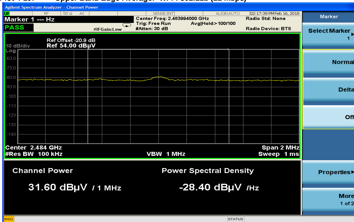
Plot 4-19: Upper Band Edge Average: Wi-Fi 802.11b (11 Mbps)
