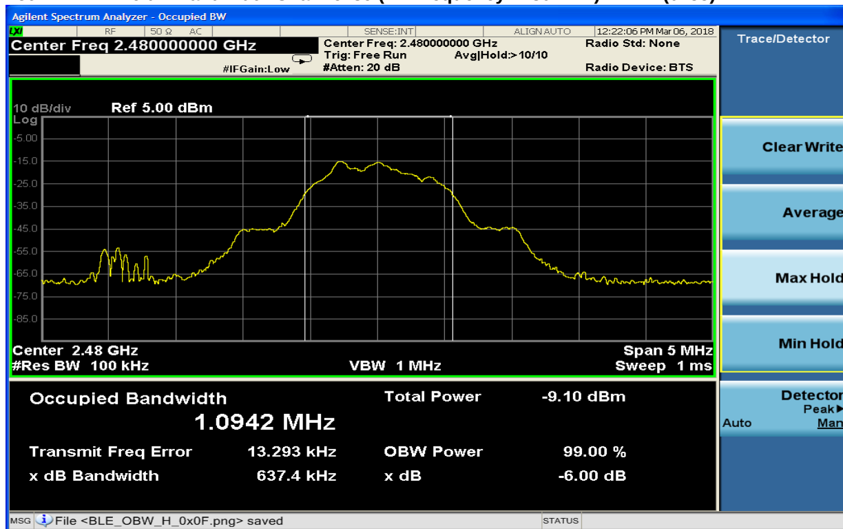
Plot 7-12: 6 dB Bandwidth Channel 39 (TX Frequency 2480 MHz) – BLE (0x55)
