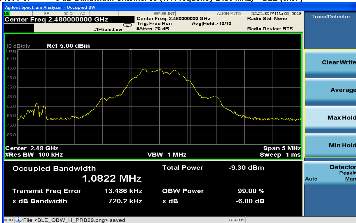
Plot 7-9: 6 dB Bandwidth Channel 39 (TX Frequency 2480 MHz) – BLE (0x0F)
