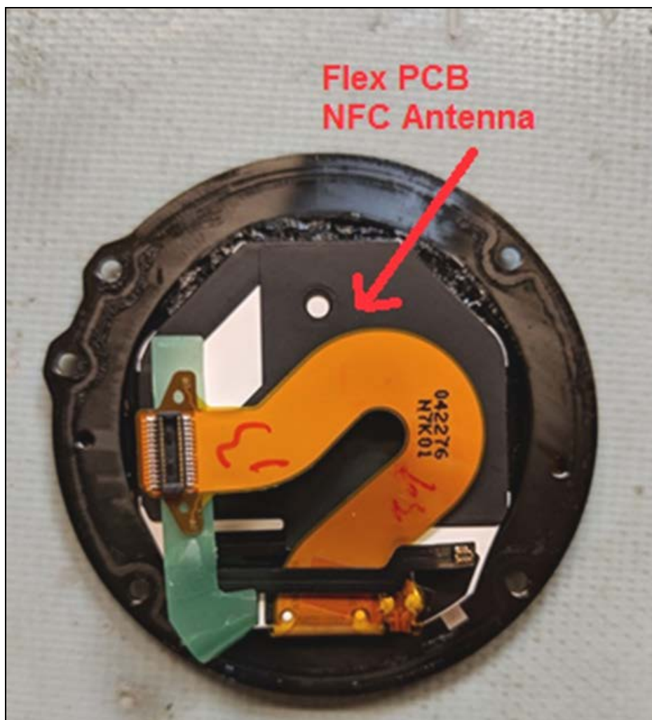
Display Assembly with NFC Antenna
