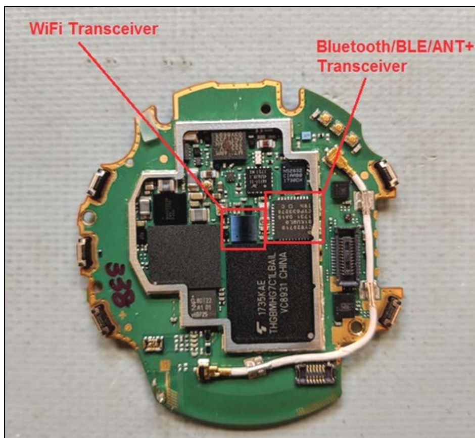
Main Board without Shield – Top View
