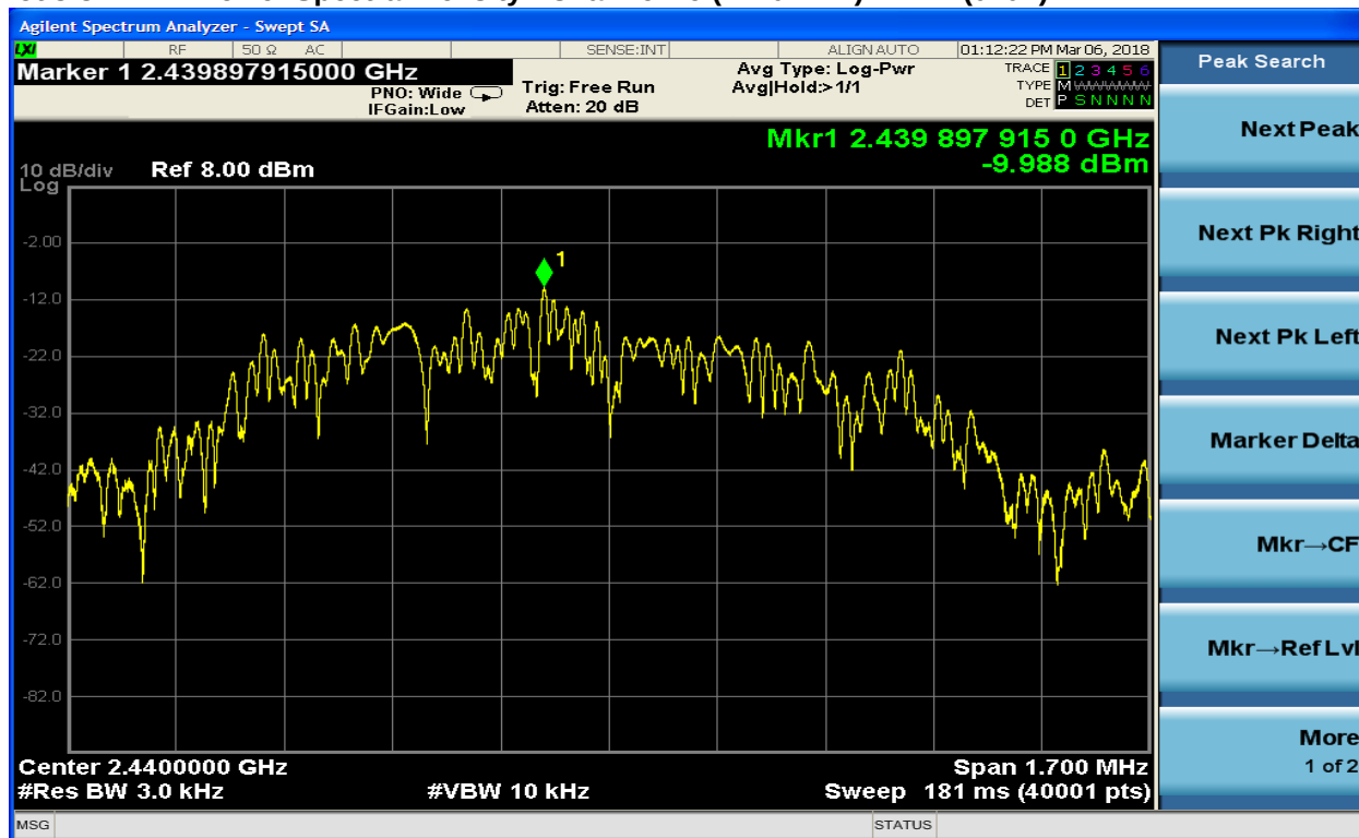
Plot 8-8: Power Spectral Density: Channel 19 (2440 MHz) – BLE (0x0F)
