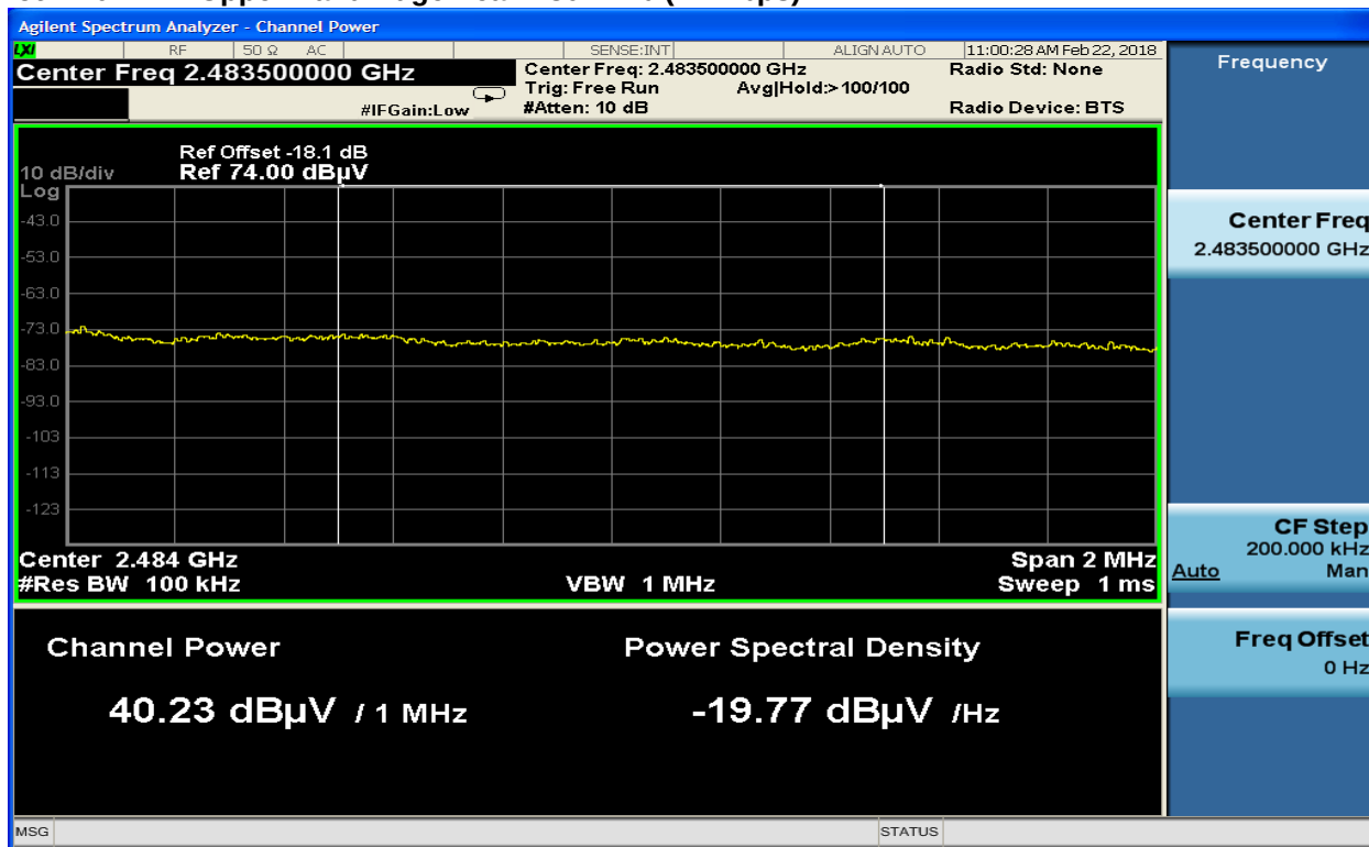
Plot 4-20: Upper Band Edge Peak: 802.11b (11 Mbps)
