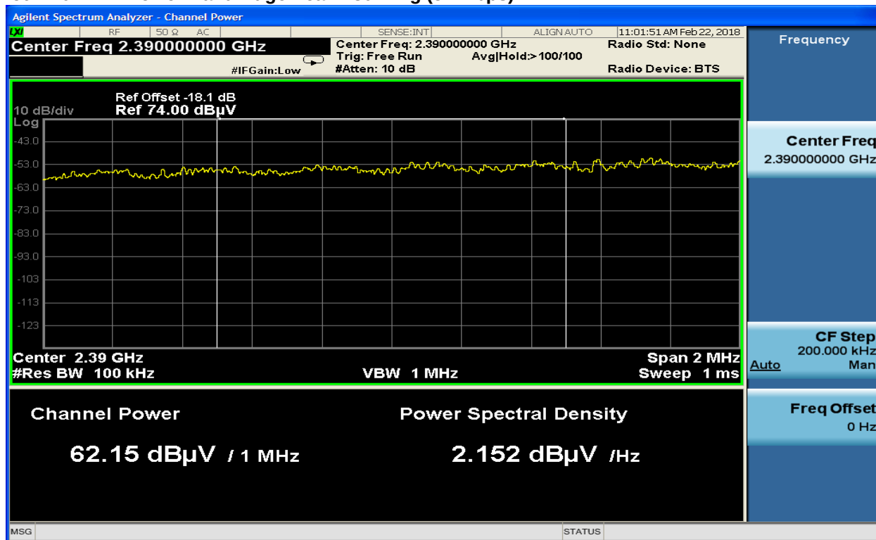
Plot 4-10: Lower Band Edge Peak: 802.11g (54 Mbps)
