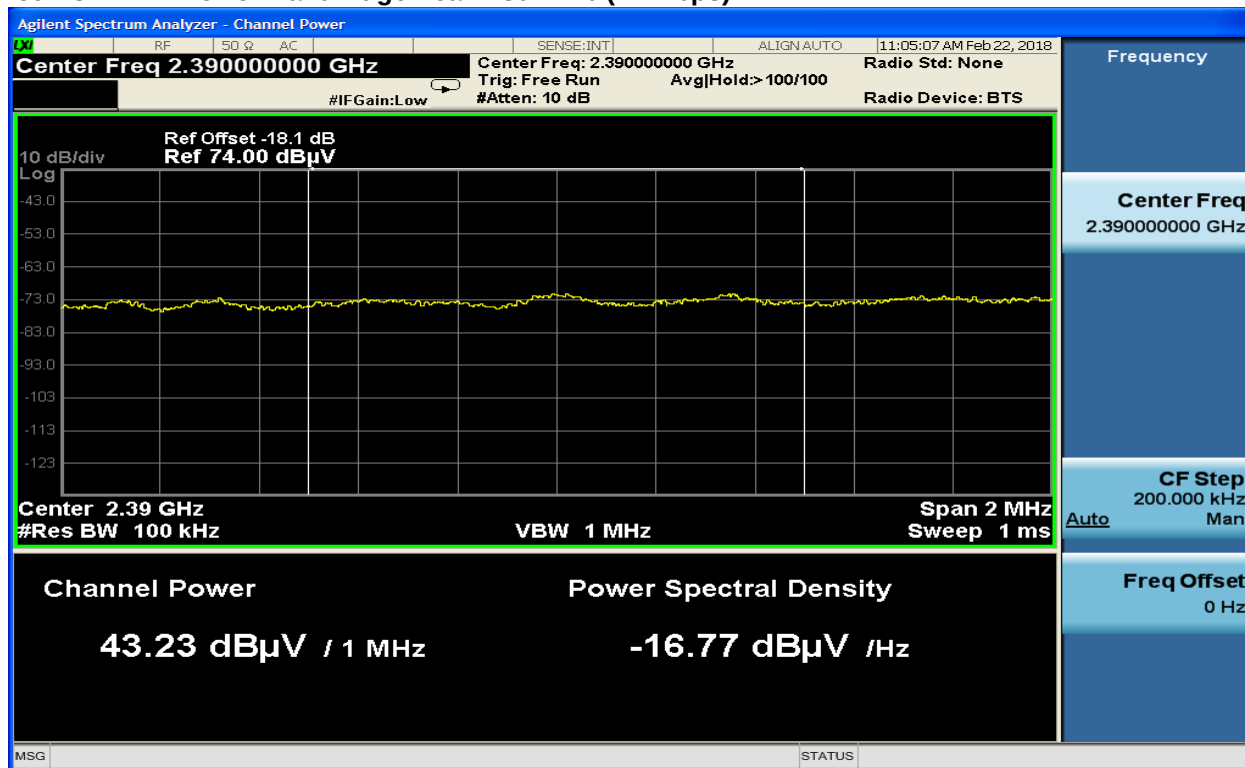
Plot 4-8: Lower Band Edge Peak: 802.11b (11 Mbps)
