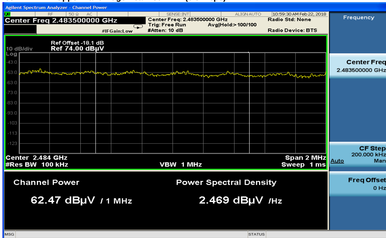
Plot 4-24: Upper Band Edge Peak: 802.11n (6.5 Mbps)
