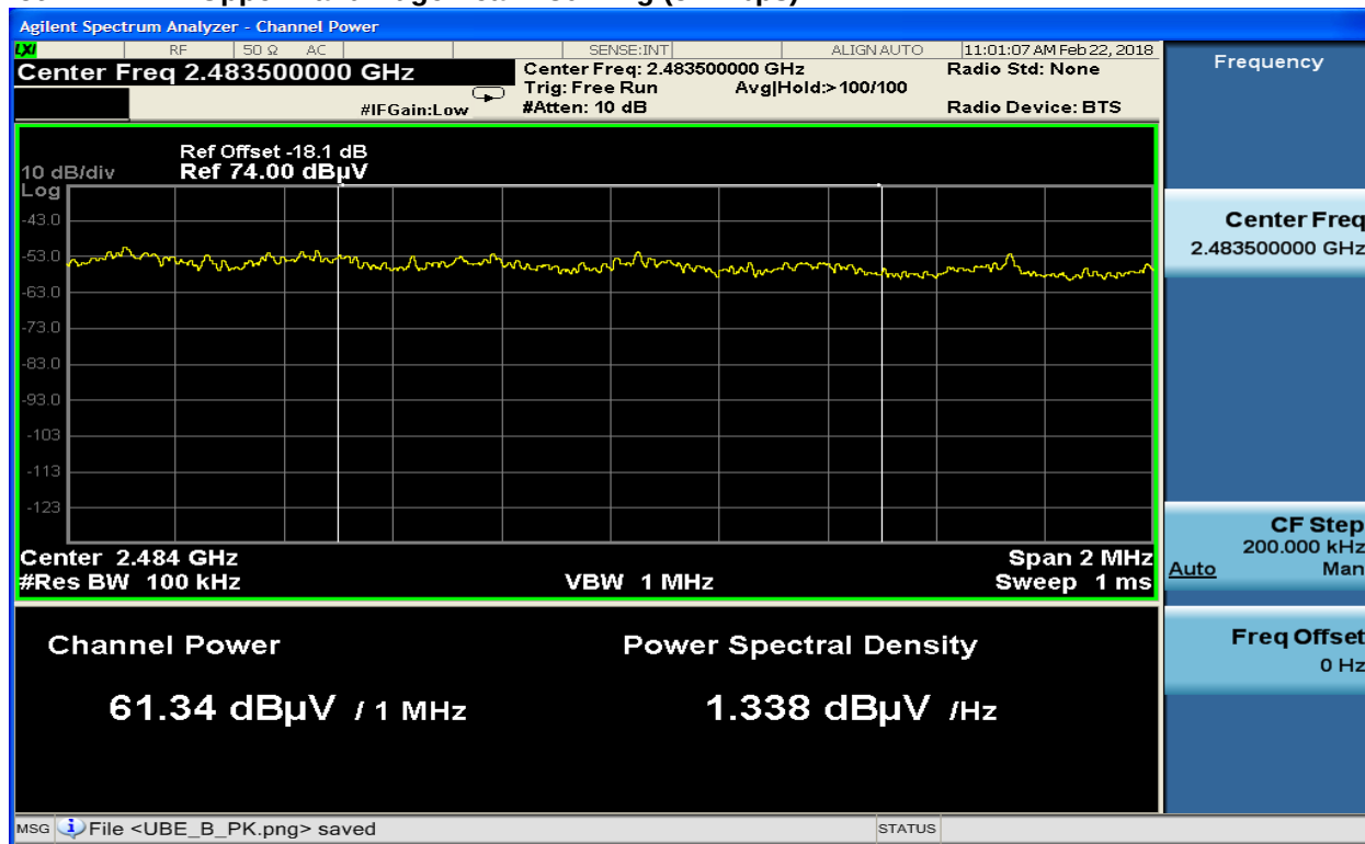
Plot 4-22: Upper Band Edge Peak: 802.11g (54 Mbps)
