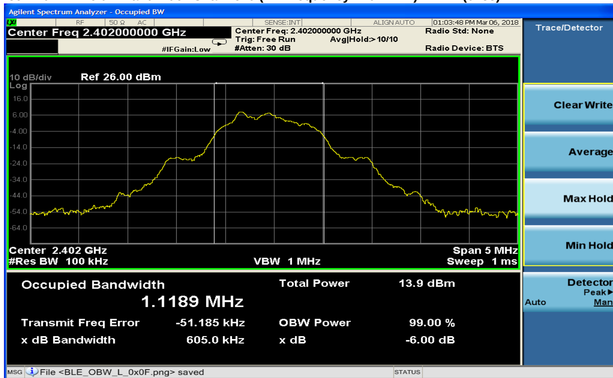
Plot 7-10: 6 dB Bandwidth Channel 0 (TX Frequency 2402 MHz) – BLE (0x55)
