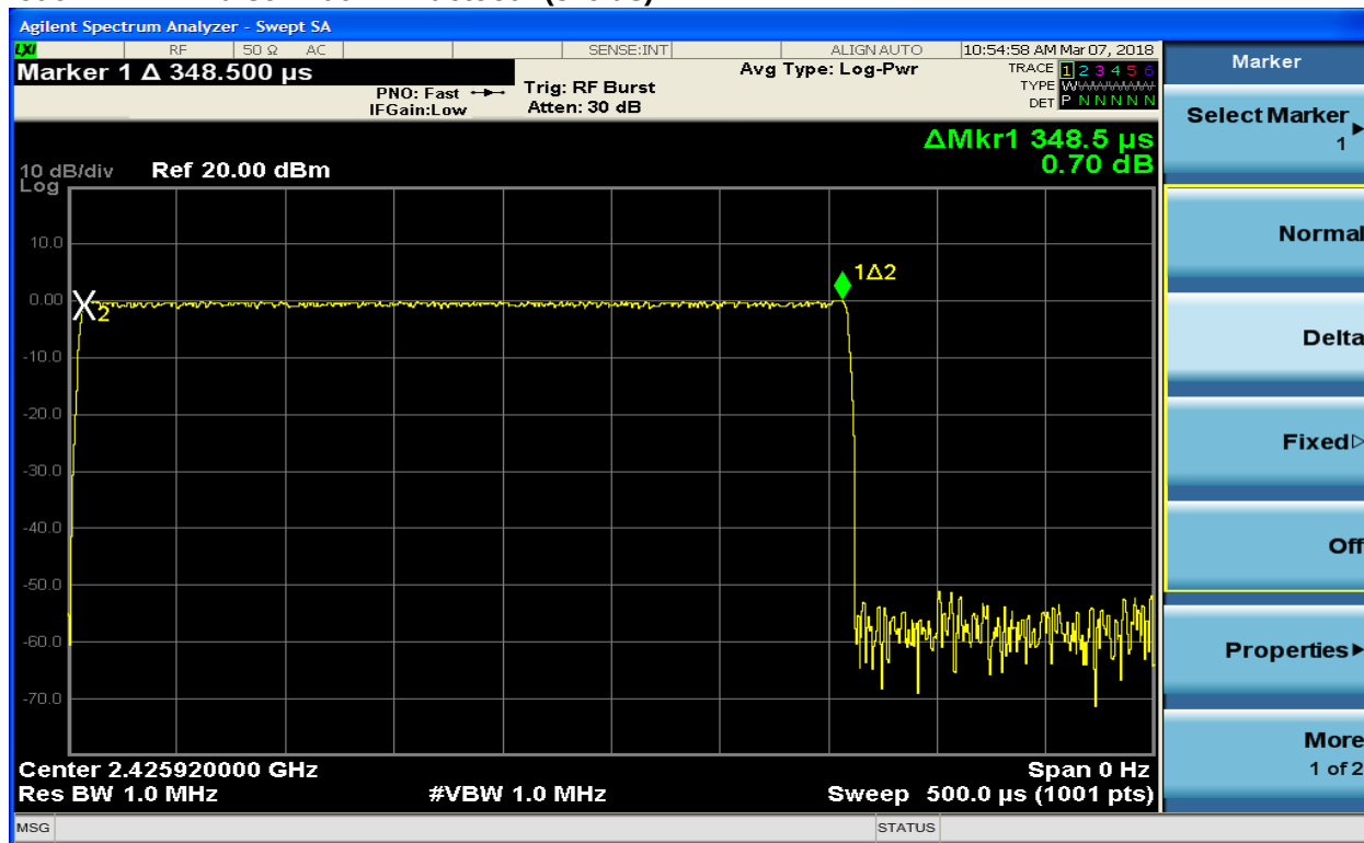
Plot 9-4: Pulse Width – Bluetooth (349 us)
