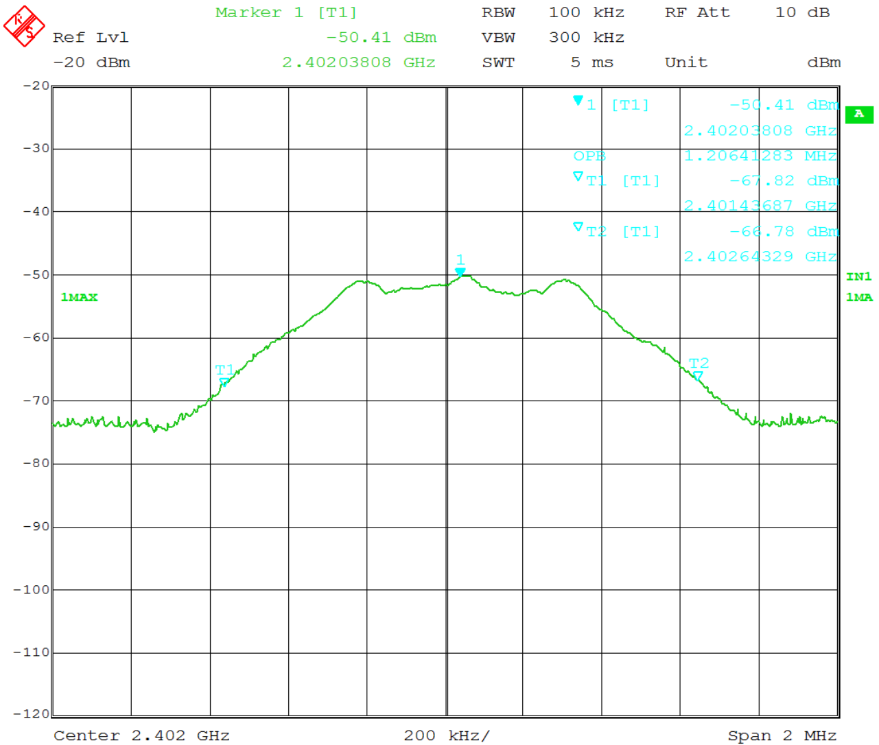
Date: 11.APR.2019 12:35:07 Figure 10 - 99% Occupied Bandwidth, Low Channel, GFSK
