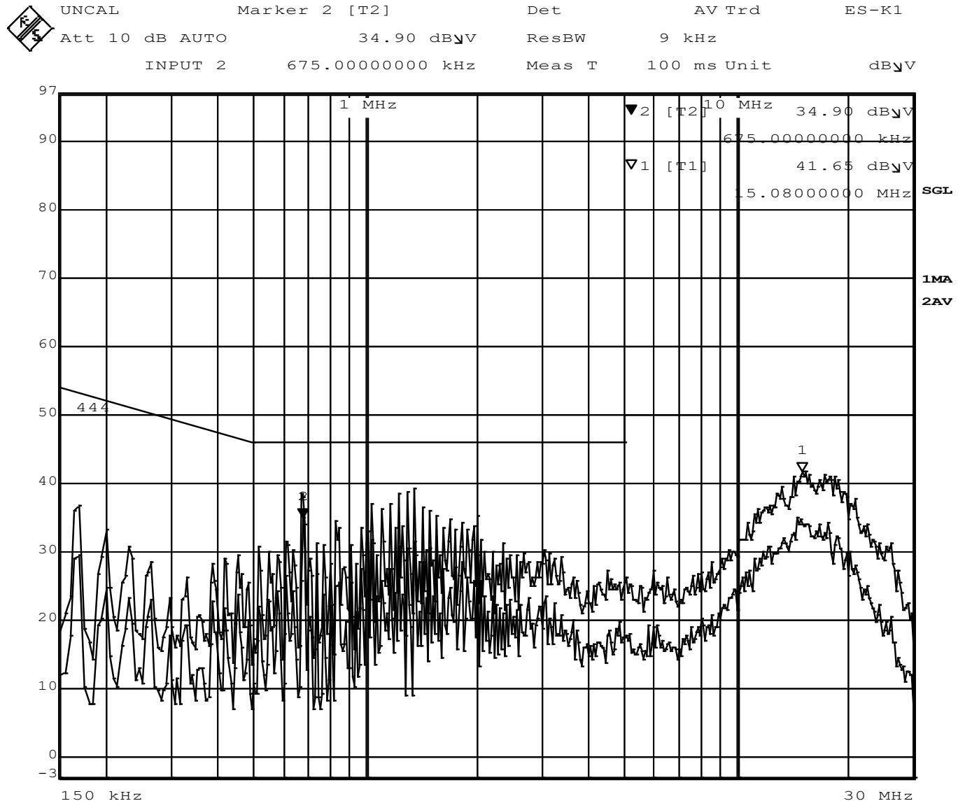
Figure 11 - Conducted Emissions Plot, L-F
