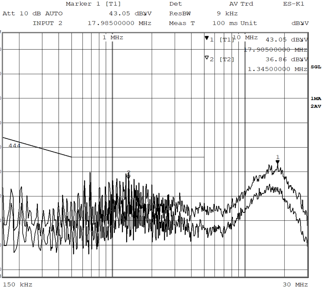
Figure 12 - Conducted Emissions Plot, N-F All Measurements were found to be at least 10 dB below the limits.
