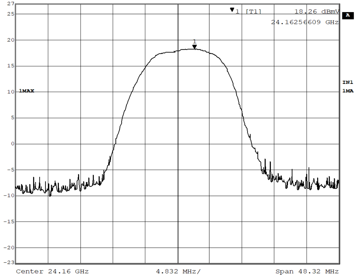
Figure 2 - Analyzer Measurement – Fundamental, Channel Mid
