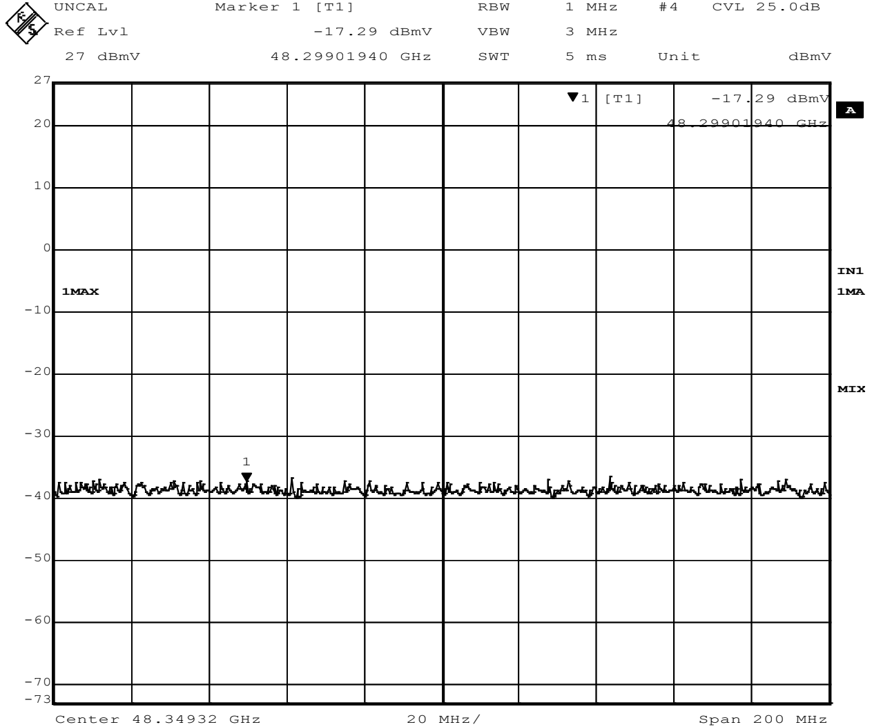
Figure 7 - Analyzer Measurement – 2nd Harmonic, Channel High
