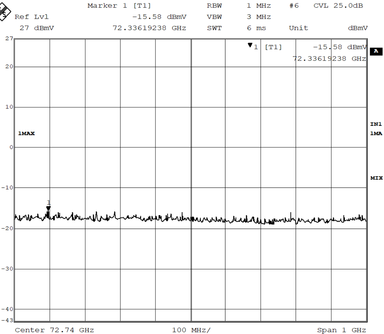
Figure 9 - Analyzer Measurement – 3rd Harmonic, Channel Mid
