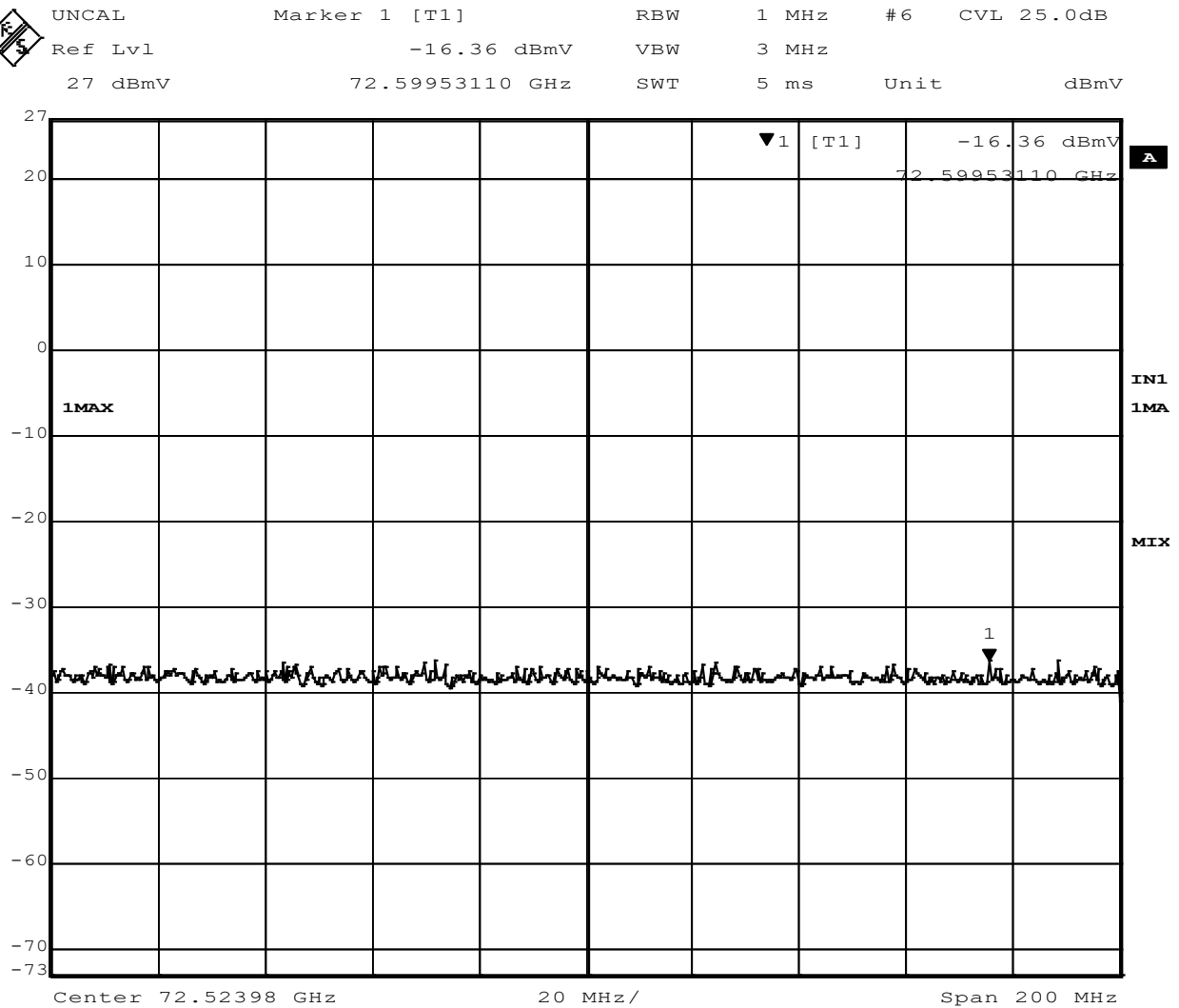
Figure 10 - Analyzer Measurement – 3rd Harmonic, Channel High
