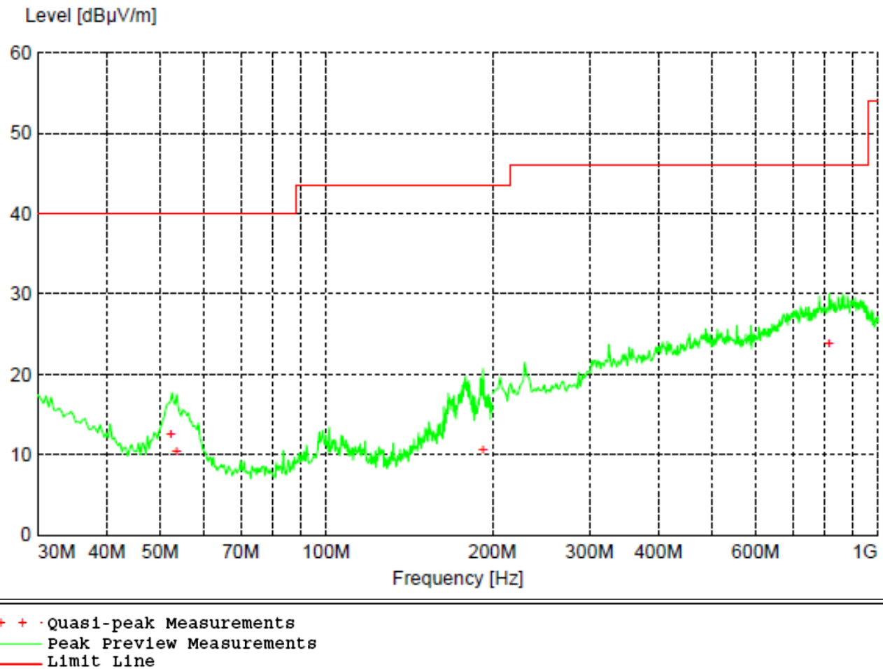
Figure 24 - Radiated Emissions Plot, GMSK
