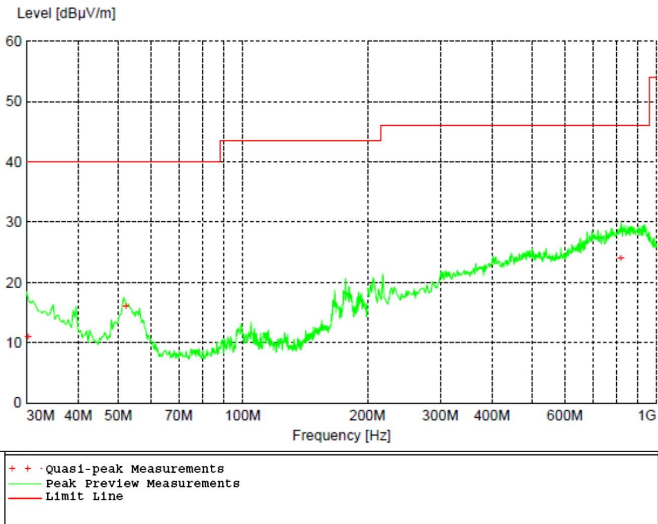
Figure 23 - Radiated Emissions Plot, Receive, GFSK
