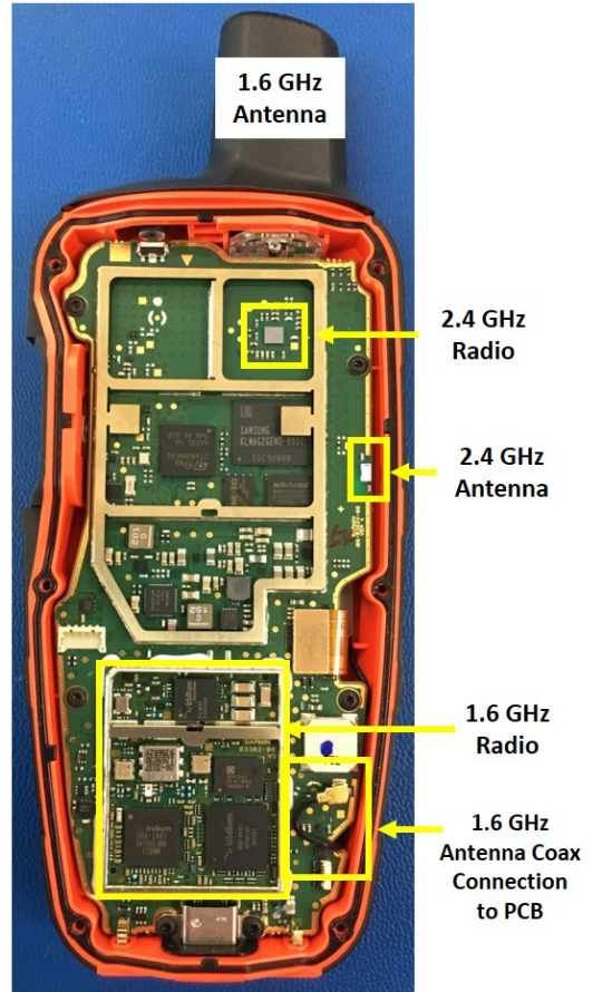
Back of PCBA w/o Shields
