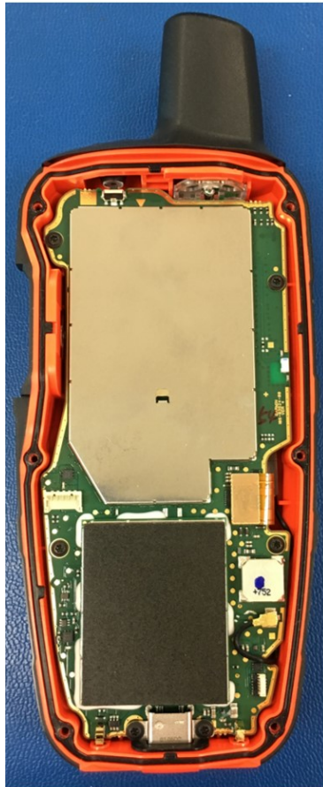
Back of PCBA w/Shields
