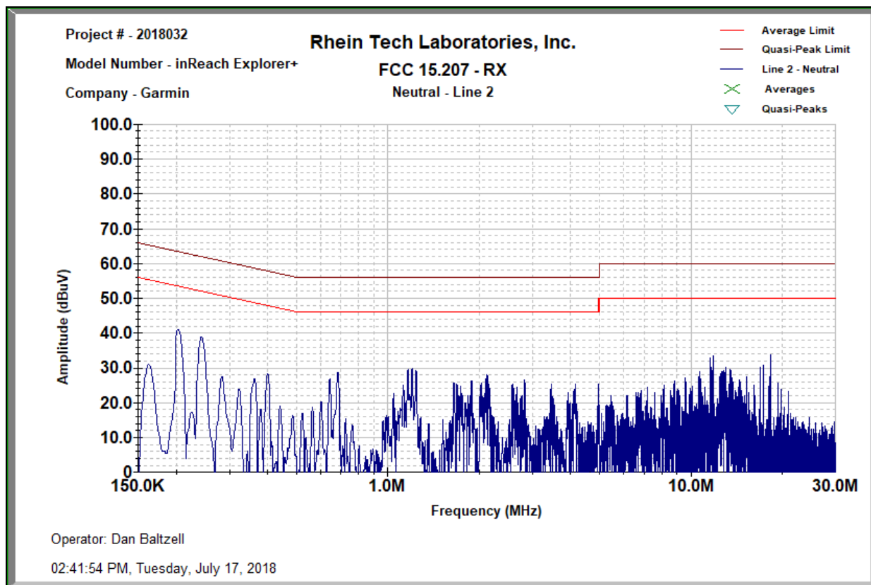
Plot 10-9: Conducted Emissions - Neutral Side – RX – AC Adapter PSAI05R-050Q
