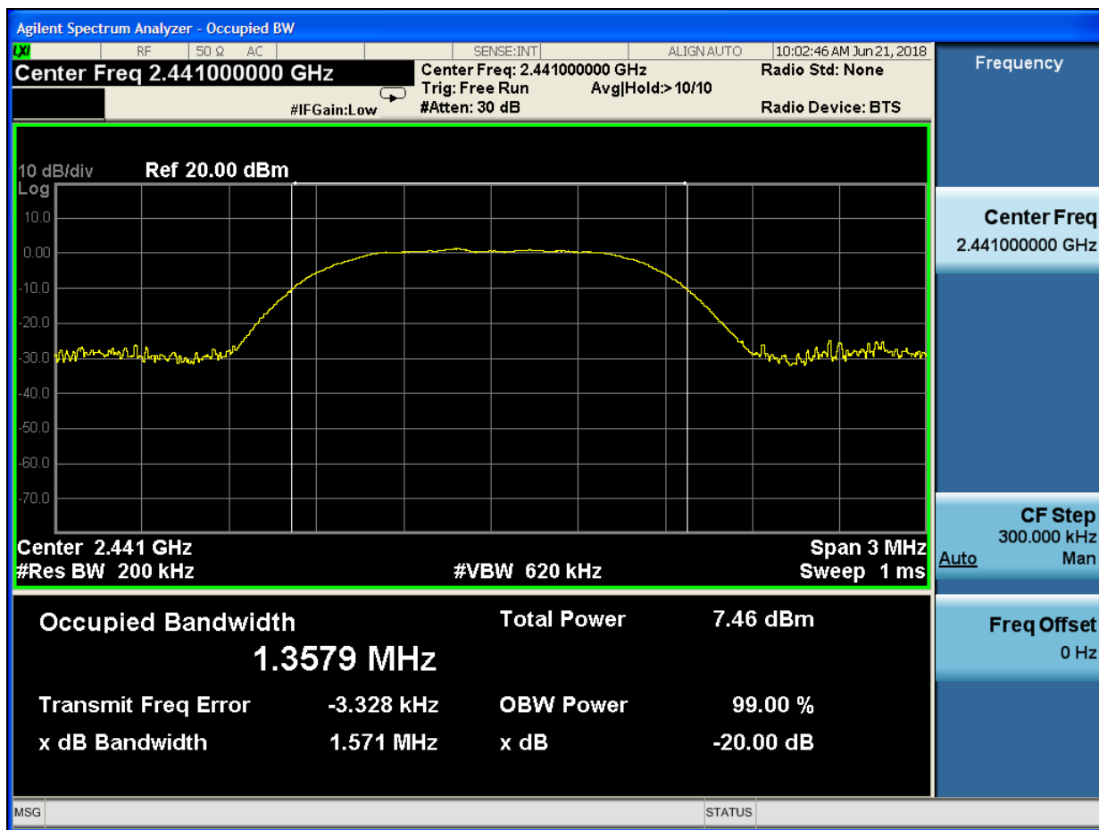
Plot 7-2: Bandwidth Channel 39 (TX Frequency 2441 MHz) – 2-EDR
