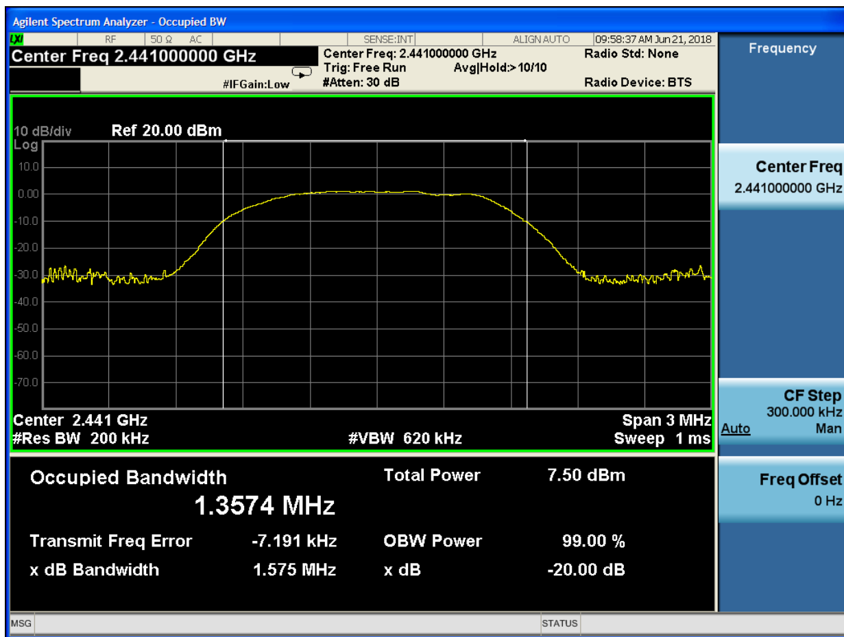
Plot 7-5: Bandwidth Channel 39 (TX Frequency 2441 MHz) – 3-EDR
