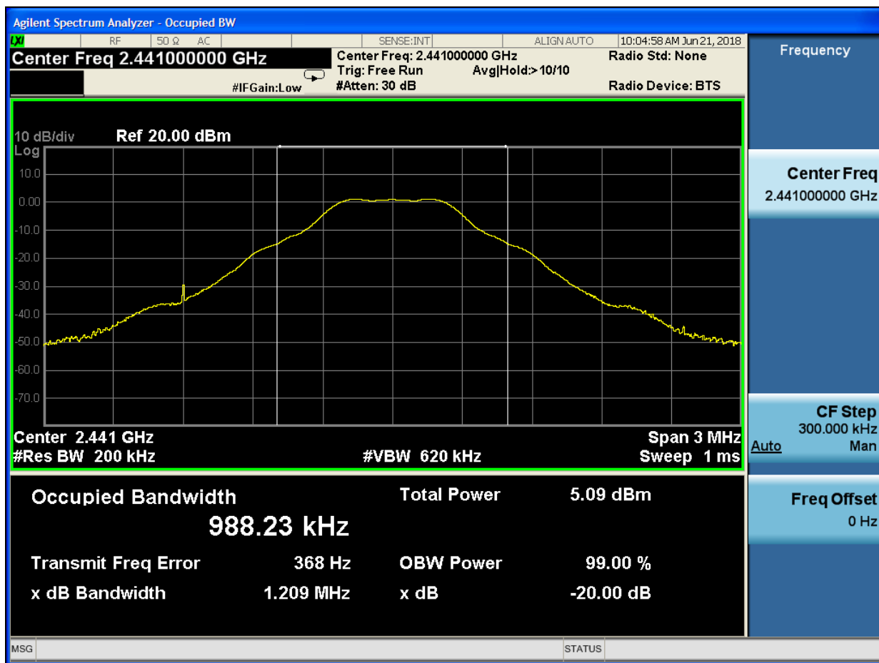
Plot 7-8: Bandwidth Channel 39 (TX Frequency 2441 MHz) – GFSK
