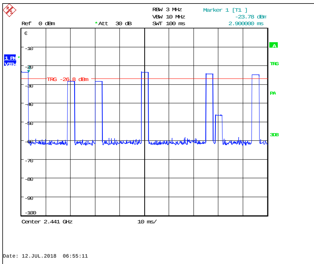
Plot 4-1: Duty Cycle
