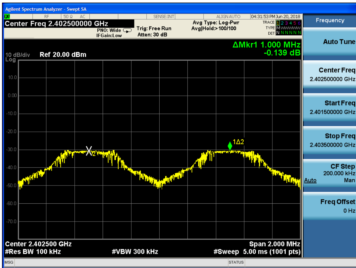
Plot 8-2: Channel Separation – Bluetooth (1 MHz)
