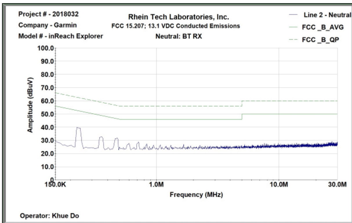
Plot 10-13: Conducted Emissions - Neutral Side – RX – Car Charger Adapter RF-279-G021-0
