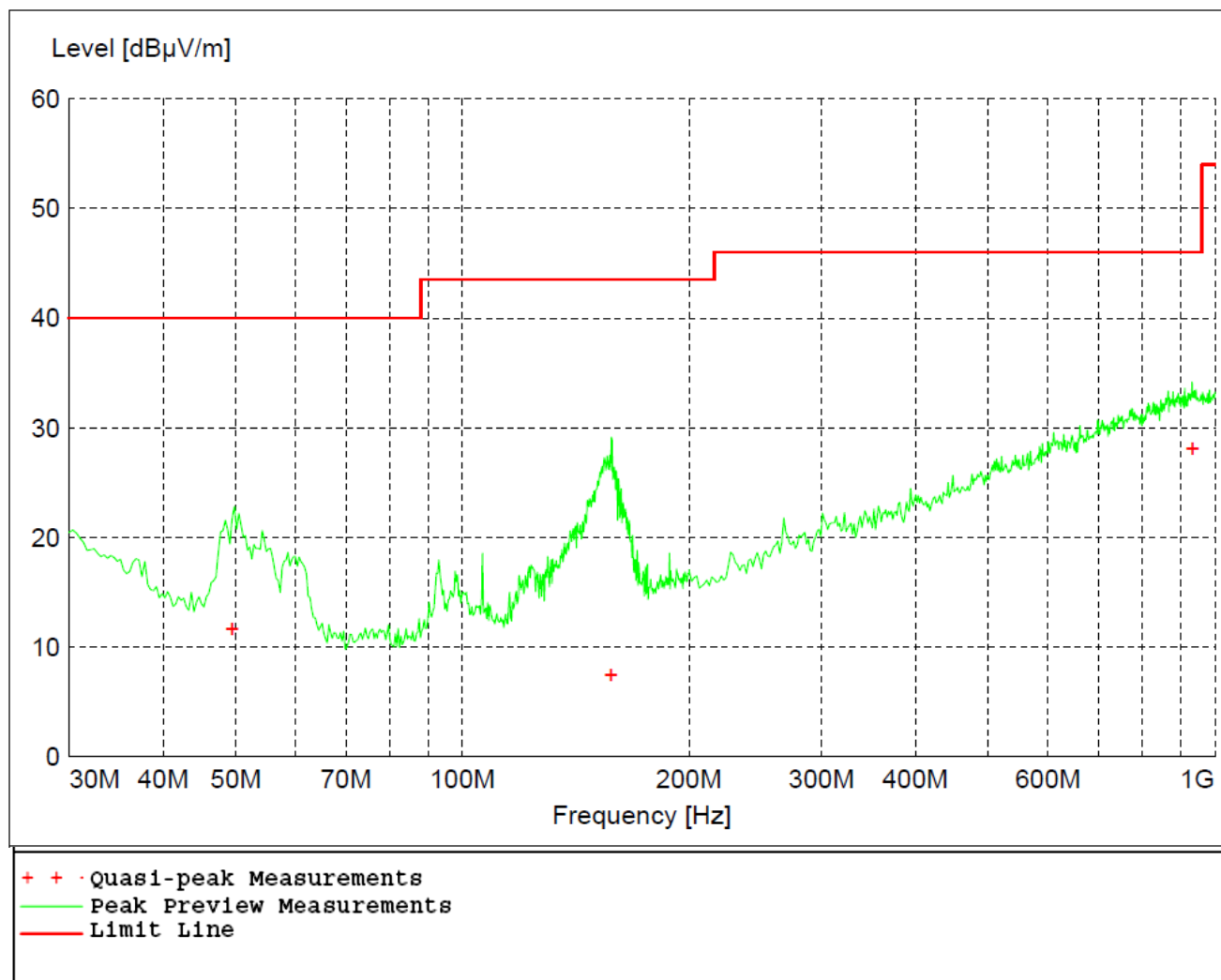
Figure 15 - Radiated Emissions Plot, Receive, GFSK
