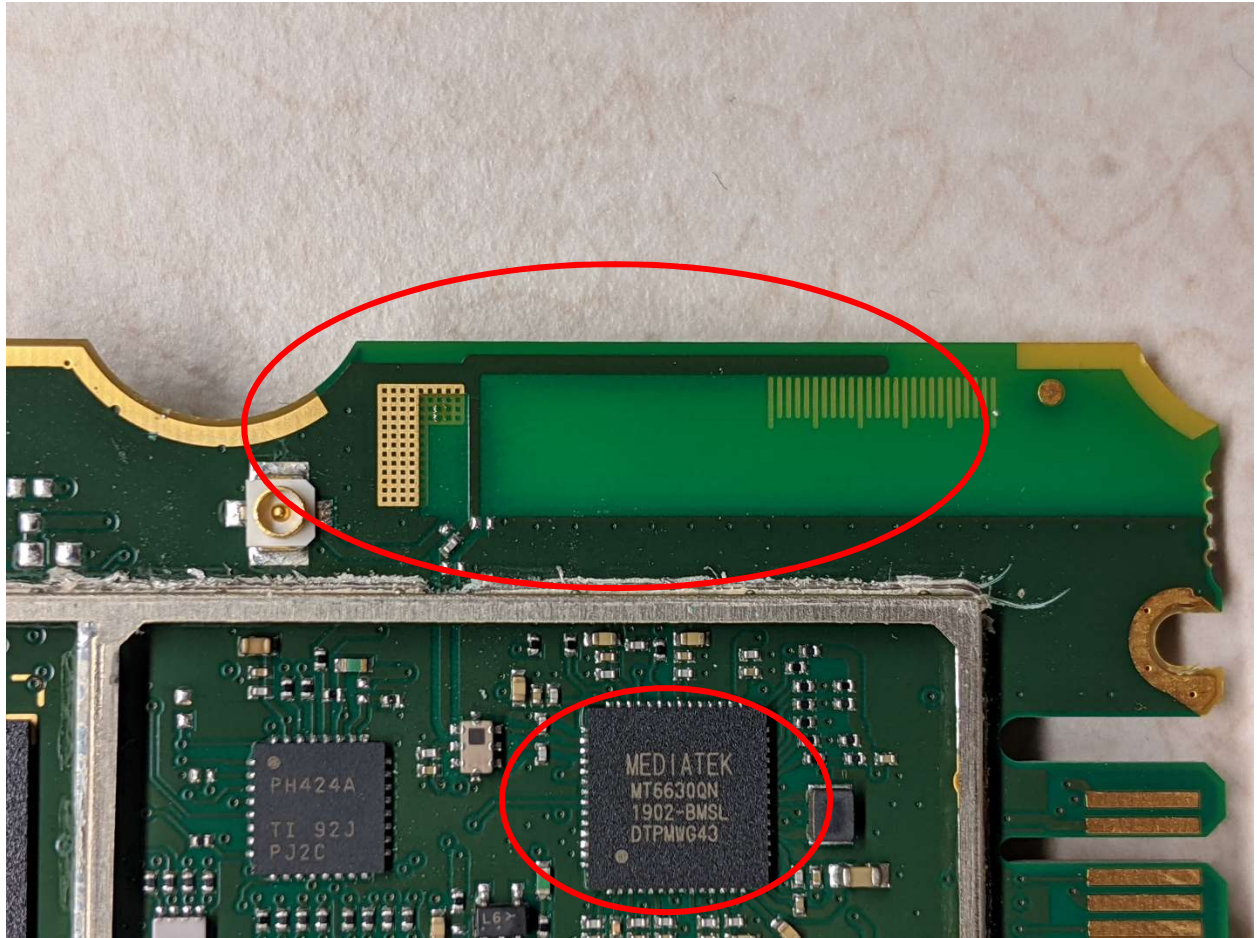
Figure 3- M/N: C3545 Transceiver IC and Antenna
