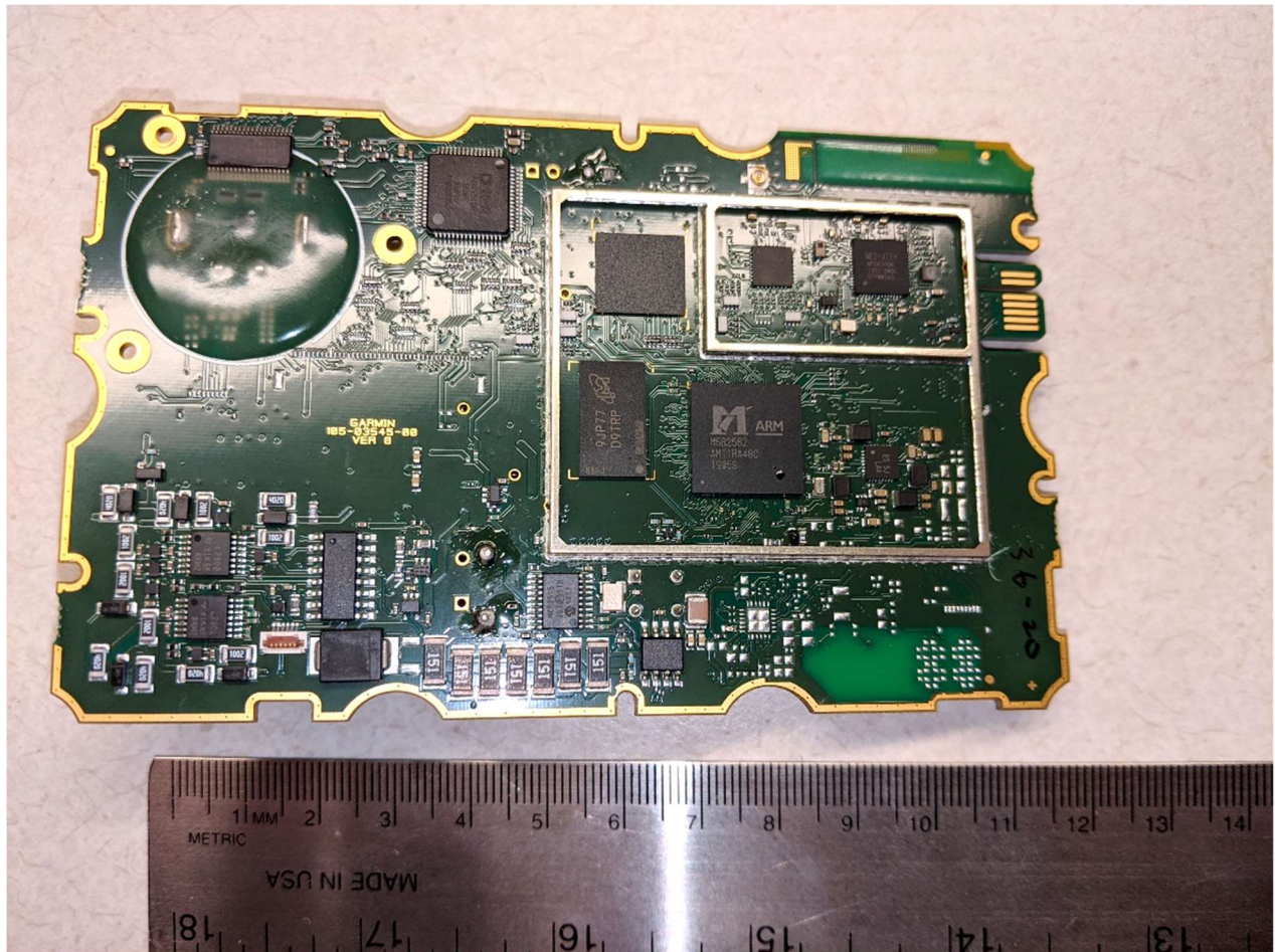
Figure 2 - M/N: C3545 PCB Rear
