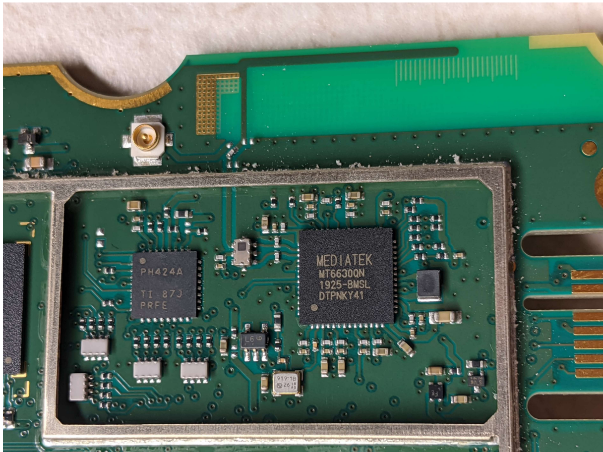
Figure 6 - M/N: A3545 Antenna and TX Chip
