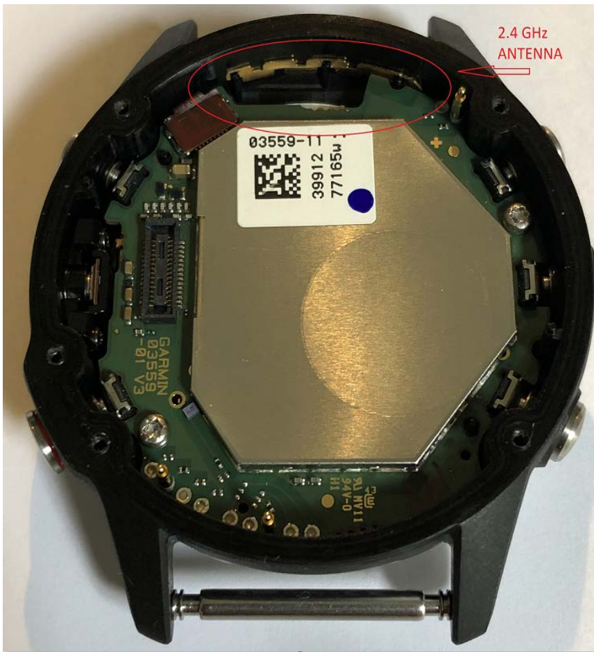
Figure 7 - Antenna
