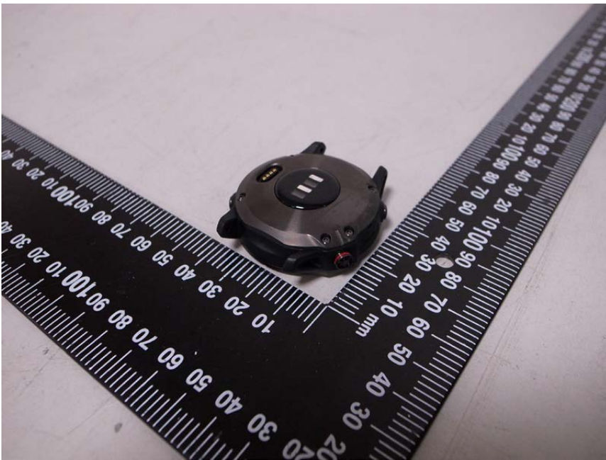
Figure 2 - EUT Rear
