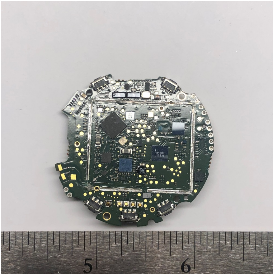
Figure 4- PCB Front Un-Shielded
