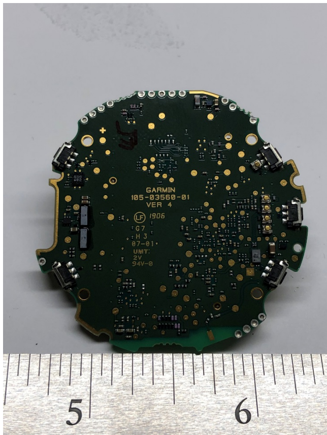
Figure 3 - PCB Front
