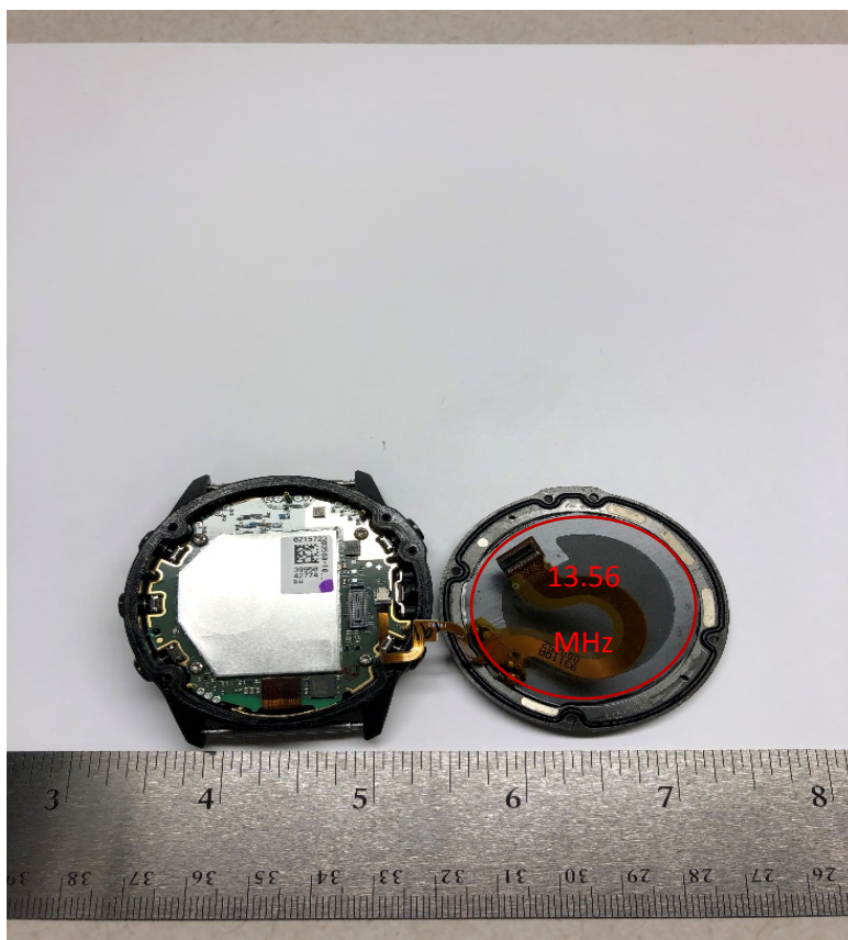
Figure 4 - EUT Rear (shielded), 13.56MHz Antenna
