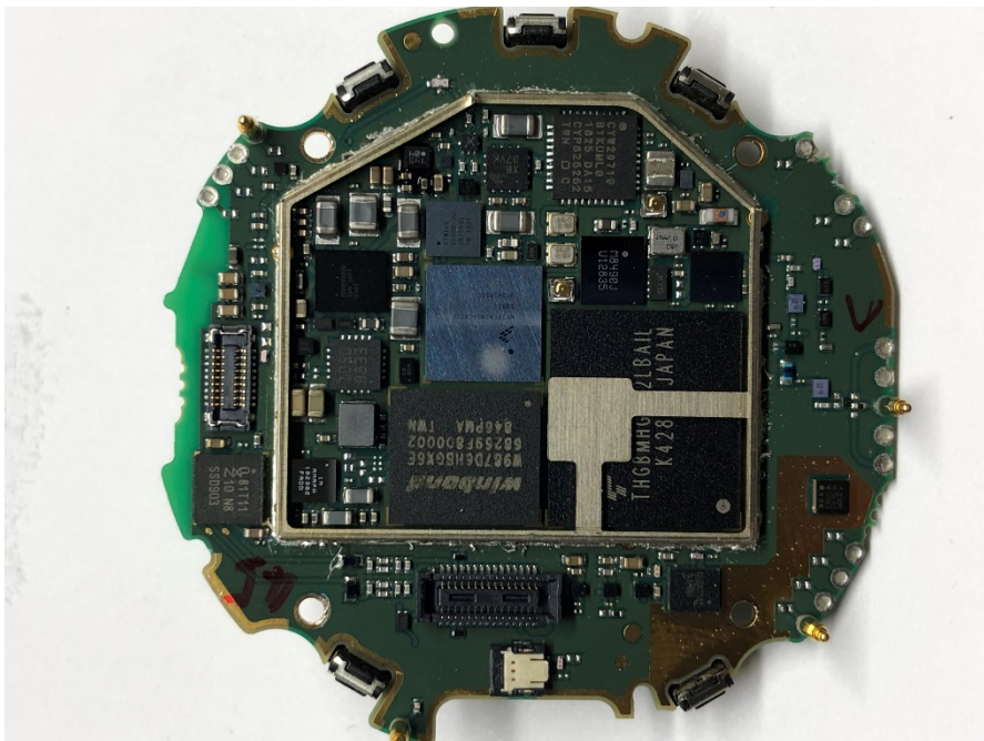
Figure 5 - PCB Rear (un-shielded)
