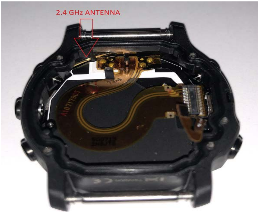
Figure 7 - ANTENNA
