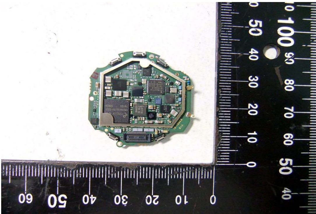
Figure 6 - PCB Front (un-shielded)
