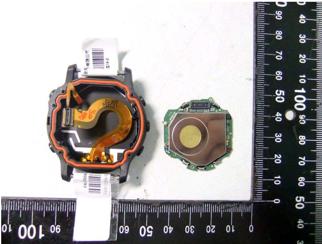
Figure 5 - PCB Front (shielded)
